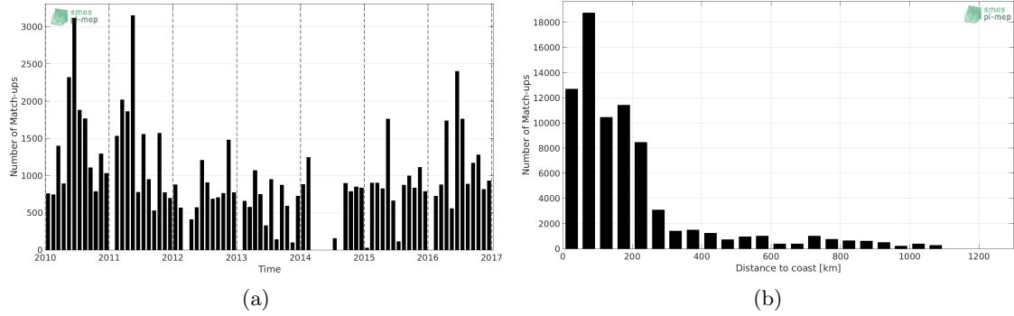
Figure 1: Number of match-ups between TSG-LEGOS-DM and SMOS-L3-CATDS-CECOS-LOCEAN-V3-9DAYS-25KM SSS as a function of time (a) and as function of the distance to coast (b) over the South Atlantic Ocean Pi-MEP region and for the full satellite product period.
