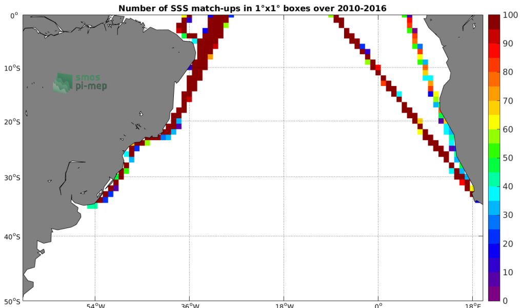
Figure 4: Number of SSS match-ups between TSG-LEGOS-DM SSS and the SMOS-L3-CATDS-CECOS-LOCEAN-V3-9DAYS-25KM SSS product for the South Atlantic Ocean Pi-MEP region over 1^\circ \times 1^\circ boxes and for the full satellite product period.
