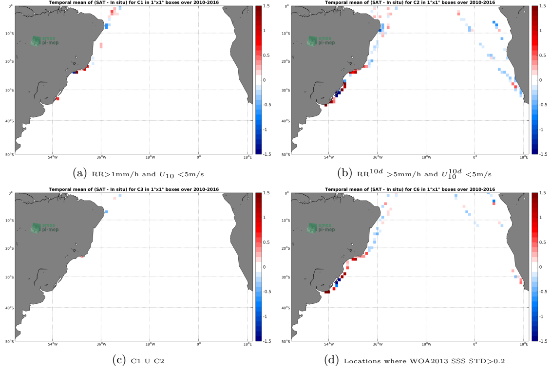
Figure 12: Temporal mean gridded over spatial boxes of size 1^\circ \times 1^\circ of \Delta SSS (SMOS-L3-CATDS-CECOS-LOCEAN-V3-9DAYS-25KM - TSG-LEGOS-DM) for 4 different subdatasets corresponding to: RR > 1\text{mm/h} and U_{10} < 5\text{m/s} (a), RR^{10d} > 5\text{mm/h} and U_{10}^{10d} < 5\text{m/s} (b), C1 U C2 (c), Locations where WOA2013 SSS STD > 0.2 (d).
