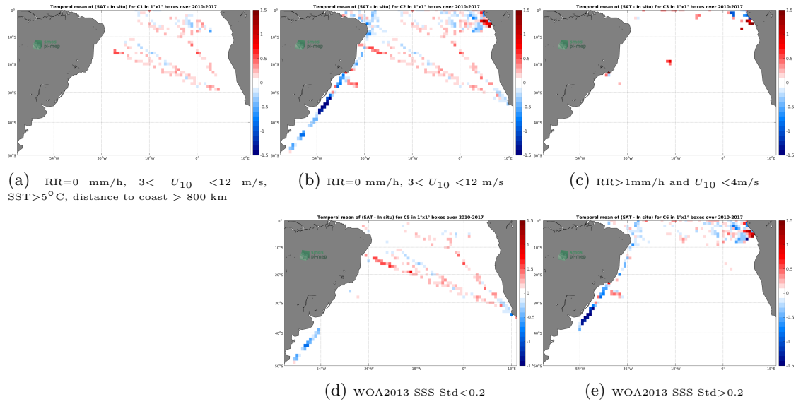
Figure 12: Temporal mean gridded over spatial boxes of size 1^\circ \times 1^\circ of \Delta SSS (SMOS-L3-CATDS-CECOS-LOCEAN-V3-9DAYS-25KM - TSG-GOSUD-Research-vessel) for 5 different subdatasets corresponding to: RR=0 mm/h, 3 < U_{10} < 12 m/s, SST > 5^\circ C , distance to coast > 800 km (a), RR=0 mm/h, 3 < U_{10} < 12 m/s (b), RR > 1 mm/h and U_{10} < 4 m/s (c), WOA2013 SSS Std < 0.2 (d), WOA2013 SSS Std > 0.2 (e).
