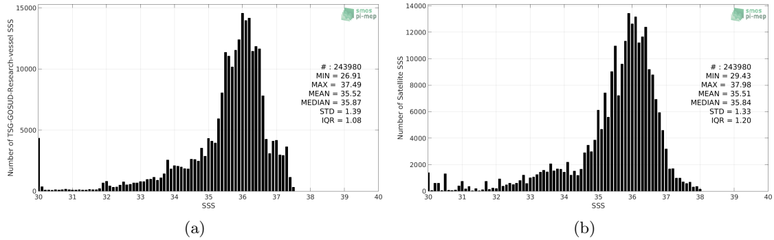
Figure 2: Histograms of SSS from TSG-GOSUD-Research-vessel (a) and SMOS-L3-CATDS-CECOS-LOCEAN-V3-9DAYS-25KM (b) considering all match-up pairs per bins of 0.1 over the South Atlantic Ocean Pi-MEP region and for the full satellite product period.
