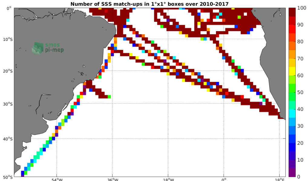
Figure 4: Number of SSS match-ups between TSG-GOSUD-Research-vessel SSS and the SMOS-L3-CATDS-CECOS-LOCEAN-V3-9DAYS-25KM SSS product for the South Atlantic Ocean Pi-MEP region over 1°x1° boxes and for the full satellite product period.
