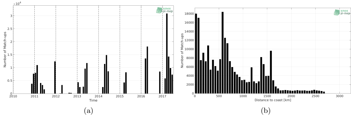
Figure 1: Number of match-ups between TSG-GOSUD-Research-vessel and SMOS-L3-CATDS-CECOS-LOCEAN-V3-9DAYS-25KM SSS as a function of time (a) and as function of the distance to coast (b) over the South Atlantic Ocean Pi-MEP region and for the full satellite product period.
