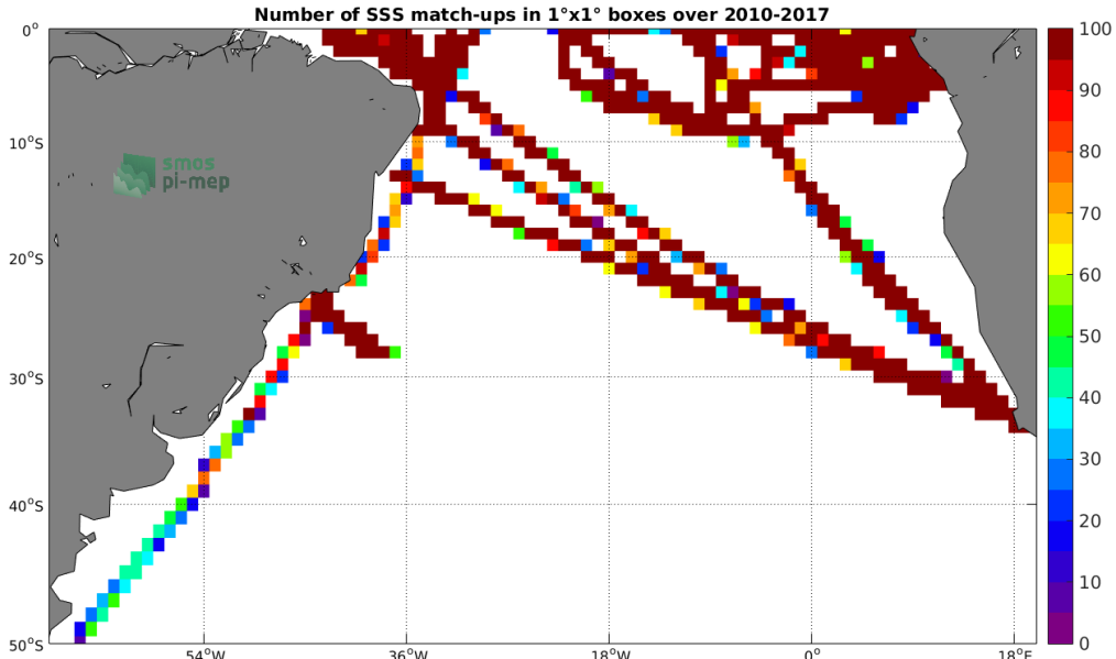
Figure 4: Number of SSS match-ups between TSG-GOSUD-Research-vessel SSS and the SMOS-L3-CATDS-CECOS-LOCEAN-V3-9DAYS-25KM SSS product for the South Atlantic Ocean Pi-MEP region over 1^\circ \times 1^\circ boxes and for the full satellite product period.
