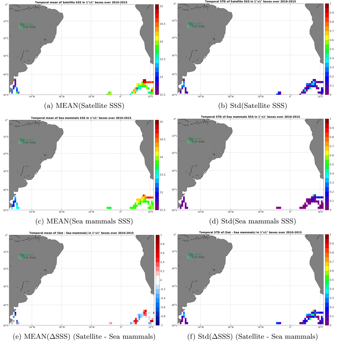
Figure 6: Temporal mean (left) and Std (right) of SSS from SMOS-L3-CATDS-CECOS-LOCEAN-V3-9DAYS-25KM (top), Sea mammals (middle), and of \Delta SSS (Satellite - Sea mammals). Only match-up pairs are used to generate these maps.
