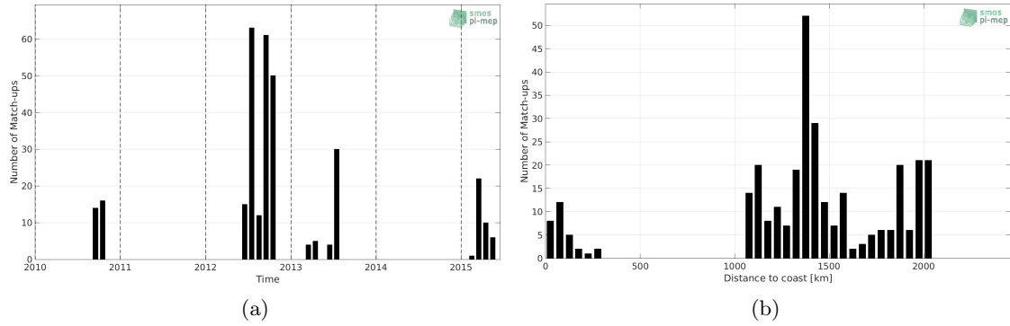
Figure 1: Number of match-ups between Sea mammals and SMOS-L3-CATDS-CECOS-LOCEAN-V3-9DAYS-25KM SSS as a function of time (a) and as function of the distance to coast (b) over the South Atlantic Ocean Pi-MEP region and for the full satellite product period.
