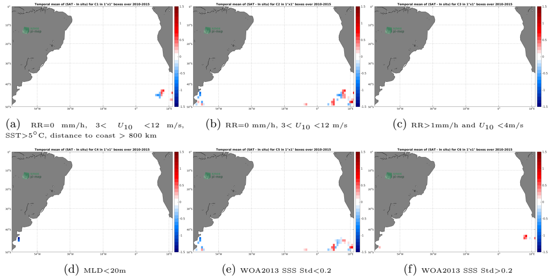
Figure 12: Temporal mean gridded over spatial boxes of size 1^\circ \times 1^\circ of \Delta SSS (SMOS-L3-CATDS-CECOS-LOCEAN-V3-9DAYS-25KM - Sea mammals) for 6 different subdatasets corresponding to: RR=0 mm/h, 3 < U_{10} < 12 m/s, SST > 5^\circ C , distance to coast > 800 km (a), RR=0 mm/h, 3 < U_{10} < 12 m/s (b), RR > 1 mm/h and U_{10} < 4 m/s (c), MLD < 20 m (d), WOA2013 SSS Std < 0.2 (e), WOA2013 SSS Std > 0.2 (f).
