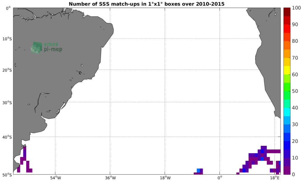
Figure 4: Number of SSS match-ups between Sea mammals SSS and the SMOS-L3-CATDS-CECOS-LOCEAN-V3-9DAYS-25KM SSS product for the South Atlantic Ocean Pi-MEP region over 1°x1° boxes and for the full satellite product period.
