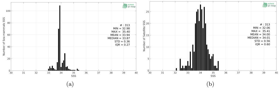
Figure 2: Histograms of SSS from Sea mammals (a) and SMOS-L3-CATDS-CECOS-LOCEAN-V3-9DAYS-25KM (b) considering all match-up pairs per bins of 0.1 over the South Atlantic Ocean Pi-MEP region and for the full satellite product period.
