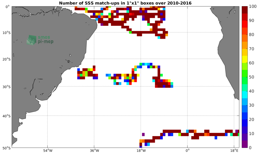
Figure 3: Number of SSS match-ups between Surface drifters SSS and the SMOS-L3-CATDS-CECOS-LOCEAN-V3-9DAYS-25KM SSS product for the South Atlantic Ocean Pi-MEP region over 1^\circ \times 1^\circ boxes and for the full satellite product period.
