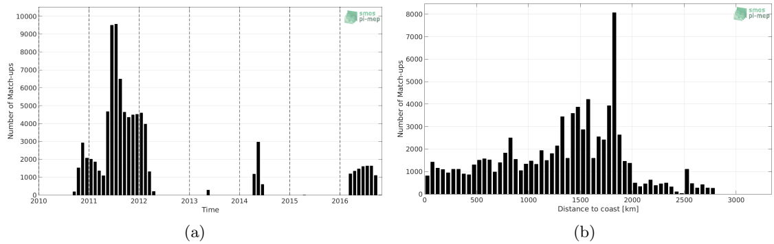
Figure 1: Number of match-ups between Surface drifters and SMOS-L3-CATDS-CECOS-LOCEAN-V3-9DAYS-25KM SSS as a function of time (a) and as function of the distance to coast (b) over the South Atlantic Ocean Pi-MEP region and for the full satellite product period.
