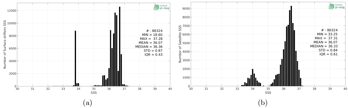
Figure 2: Histograms of SSS from Surface drifters (a) and SMOS-L3-CATDS-CECOS-LOCEAN-V3-9DAYS-25KM (b) considering all match-up pairs per bins of 0.1 over the South Atlantic Ocean Pi-MEP region and for the full satellite product period.
