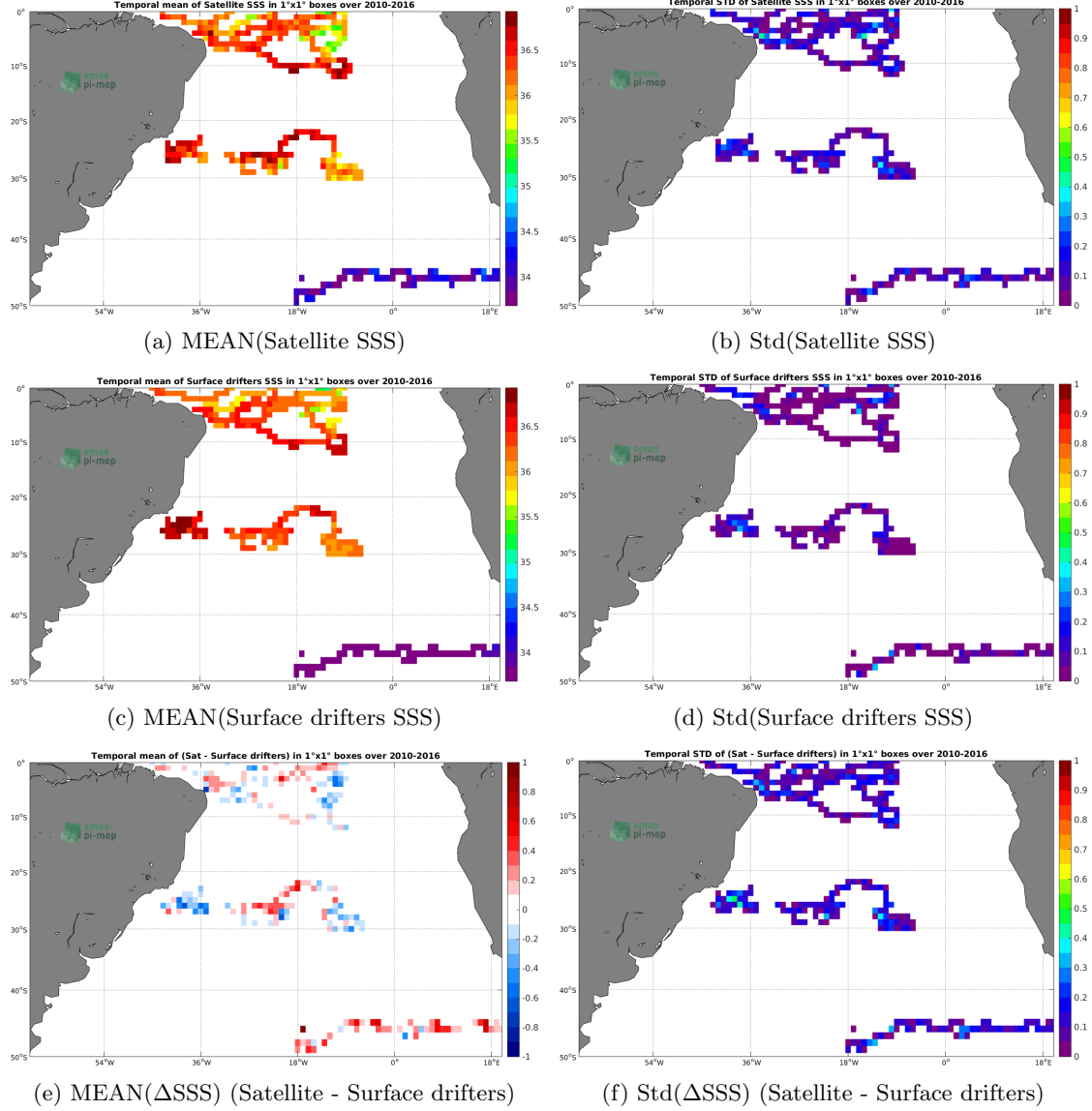
Figure 5: Temporal mean (left) and Std (right) of SSS from SMOS-L3-CATDS-CECOS-LOCEAN-V3-9DAYS-25KM (top), Surface drifters (middle), and of \Delta SSS (Satellite - Surface drifters). Only match-up pairs are used to generate these maps.
