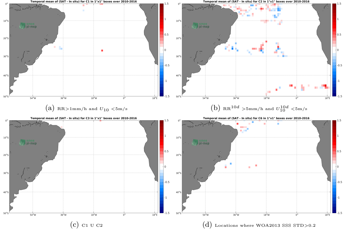
Figure 11: Temporal mean gridded over spatial boxes of size 1^\circ \times 1^\circ of \Delta SSS (SMOS-L3-CATDS-CECOS-LOCEAN-V3-9DAYS-25KM - Surface drifters) for 4 different subdatasets corresponding to: RR > 1\text{mm/h} and U_{10} < 5\text{m/s} (a), RR^{10d} > 5\text{mm/h} and U_{10}^{10d} < 5\text{m/s} (b), C1 U C2 (c), Locations where WOA2013 SSS STD > 0.2 (d).
