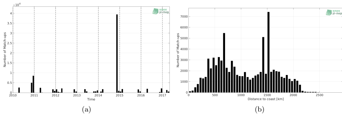
Figure 1: Number of match-ups between TSG-POLARSTERN and SMOS-L3-CATDS-CECOS-LOCEAN-V3-18DAYS-25KM SSS as a function of time (a) and as function of the distance to coast (b) over the South Atlantic Ocean Pi-MEP region and for the full satellite product period.
