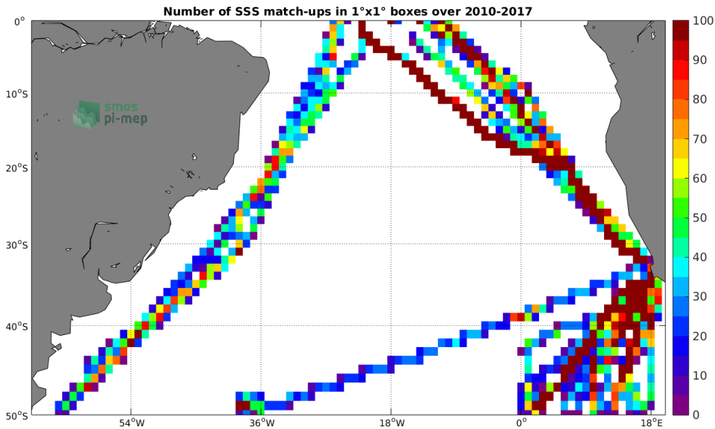
Figure 4: Number of SSS match-ups between TSG-POLARSTERN SSS and the SMOS-L3-CATDS-CECOS-LOCEAN-V3-18DAYS-25KM SSS product for the South Atlantic Ocean Pi-MEP region over 1°x1° boxes and for the full satellite product period.
