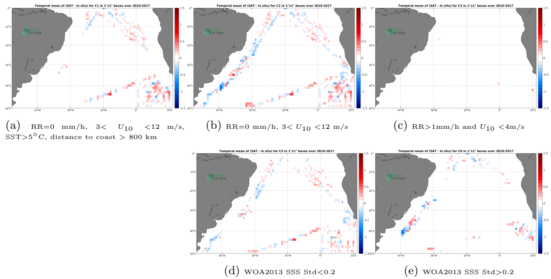
Figure 12: Temporal mean gridded over spatial boxes of size 1^\circ \times 1^\circ of \Delta SSS (SMOS-L3-CATDS-CECOS-LOCEAN-V3-18DAYS-25KM - TSG-POLARSTERN) for 5 different subdatasets corresponding to:RR=0 mm/h, 3 < U_{10} < 12 m/s, SST >5^\circ C, distance to coast > 800 km (a), RR=0 mm/h, 3 < U_{10} < 12 m/s (b), RR >1 mm/h and U_{10} < 4 m/s (c), WOA2013 SSS Std <0.2 (d), WOA2013 SSS Std >0.2 (e).
