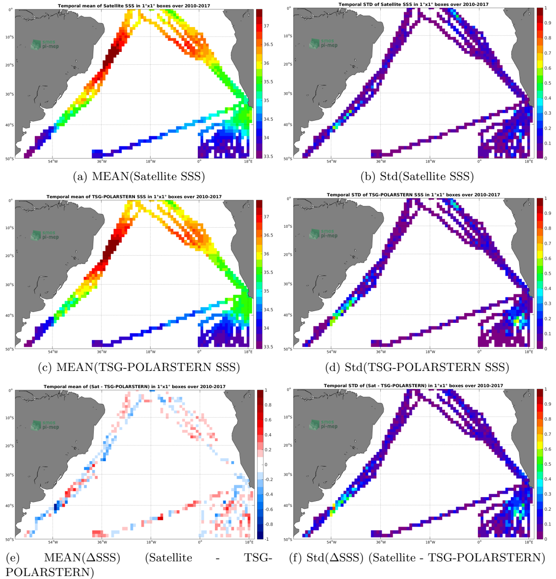
Figure 6: Temporal mean (left) and Std (right) of SSS from SMOS-L3-CATDS-CECOS-LOCEAN-V3-18DAYS-25KM (top), TSG-POLARSTERN (middle), and of \Delta SSS (Satellite - TSG-POLARSTERN). Only match-up pairs are used to generate these maps.
