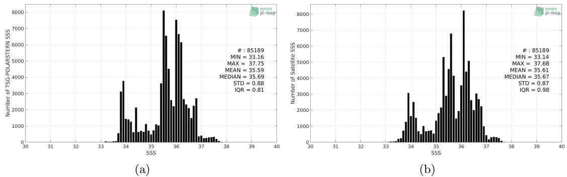
Figure 2: Histograms of SSS from TSG-POLARSTERN (a) and SMOS-L3-CATDS-CECOS-LOCEAN-V3-18DAYS-25KM (b) considering all match-up pairs per bins of 0.1 over the South Atlantic Ocean Pi-MEP region and for the full satellite product period.
