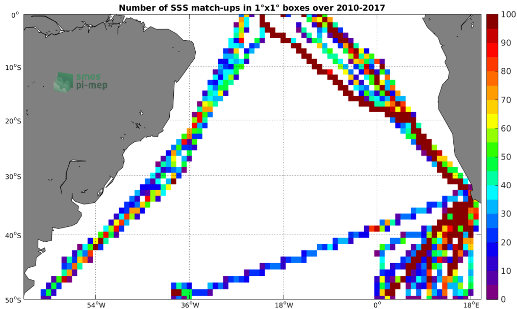
Figure 4: Number of SSS match-ups between TSG-POLARSTERN SSS and the SMOS-L3-CATDS-CECOS-LOCEAN-V3-18DAYS-25KM SSS product for the South Atlantic Ocean Pi-MEP region over 1^\circ \times 1^\circ boxes and for the full satellite product period.
