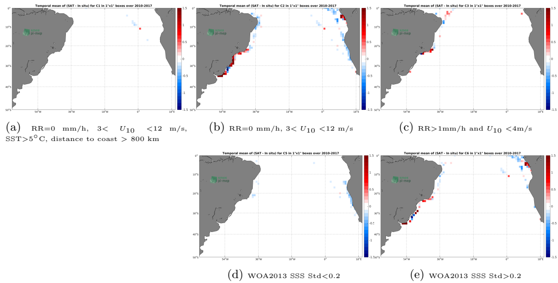
Figure 12: Temporal mean gridded over spatial boxes of size 1^\circ \times 1^\circ of \Delta SSS (SMOS-L3-CATDS-CECOS-LOCEAN-V3-18DAYS-25KM - TSG-LEGOS-DM) for 5 different subdatasets corresponding to: RR=0 mm/h, 3 < U_{10} < 12 m/s, SST > 5^\circ C , distance to coast > 800 km (a), RR=0 mm/h, 3 < U_{10} < 12 m/s (b), RR > 1 mm/h and U_{10} < 4 m/s (c), WOA2013 SSS Std < 0.2 (d), WOA2013 SSS Std > 0.2 (e).
