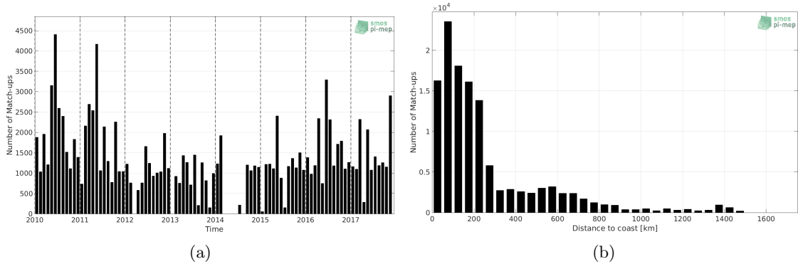
Figure 1: Number of match-ups between TSG-LEGOS-DM and SMOS-L3-CATDS-CECOS-LOCEAN-V3-18DAYS-25KM SSS as a function of time (a) and as function of the distance to coast (b) over the South Atlantic Ocean Pi-MEP region and for the full satellite product period.
