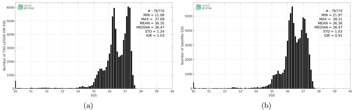
Figure 2: Histograms of SSS from TSG-LEGOS-DM (a) and SMOS-L3-CATDS-CECOS-LOCEAN-V3-18DAYS-25KM (b) considering all match-up pairs per bins of 0.1 over the South Atlantic Ocean Pi-MEP region and for the full satellite product period.
