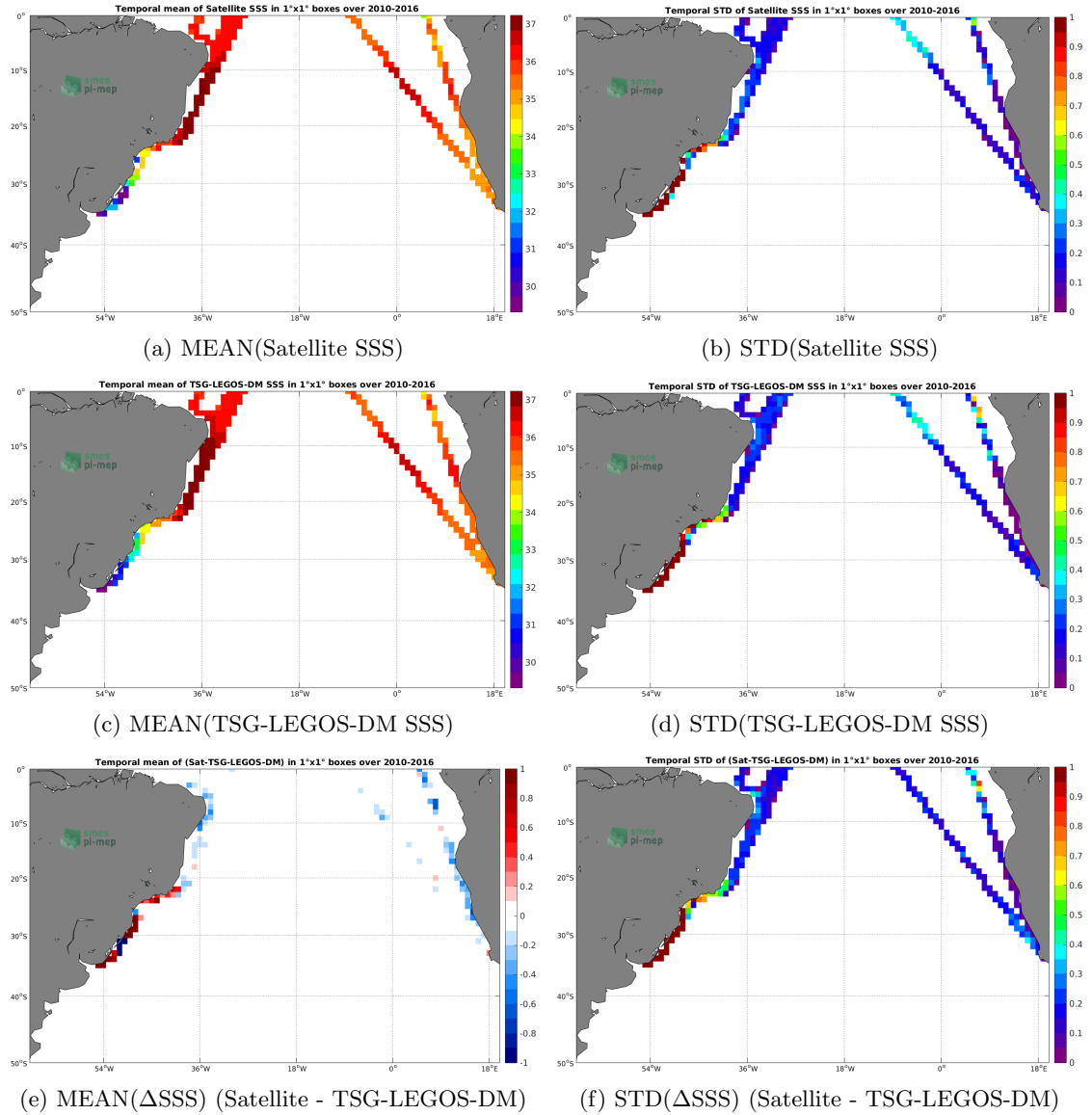
Figure 6: Temporal mean (left) and STD (right) of SSS from SMOS-L3-CATDS-CECOS-LOCEAN-V3-18DAYS-25KM (top), TSG-LEGOS-DM (middle), and of \Delta SSS (Satellite - TSG-LEGOS-DM). Only match-up pairs are used to generate these maps.
