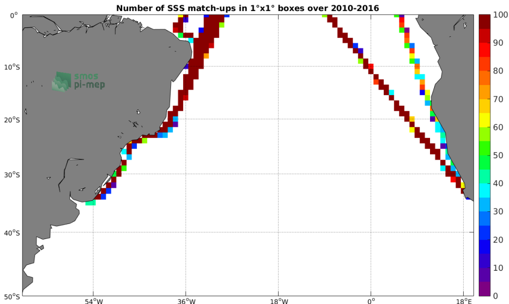
Figure 4: Number of SSS match-ups between TSG-LEGOS-DM SSS and the SMOS-L3-CATDS-CECOS-LOCEAN-V3-18DAYS-25KM SSS product for the South Atlantic Ocean Pi-MEP region over 1^\circ \times 1^\circ boxes and for the full satellite product period.
