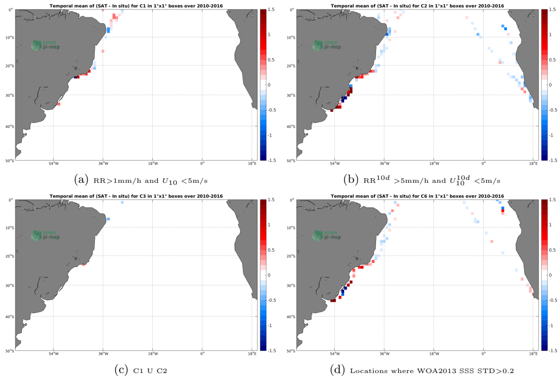
Figure 12: Temporal mean gridded over spatial boxes of size 1^\circ \times 1^\circ of \Delta SSS (SMOS-L3-CATDS-CECOS-LOCEAN-V3-18DAYS-25KM - TSG-LEGOS-DM) for 4 different subdatasets corresponding to:RR >1 mm/h and U_{10} < 5 m/s (a), RR^{10d} > 5 mm/h and U_{10}^{10d} < 5 m/s (b), C1 U C2 (c),Locations where WOA2013 SSS STD >0.2 (d).
