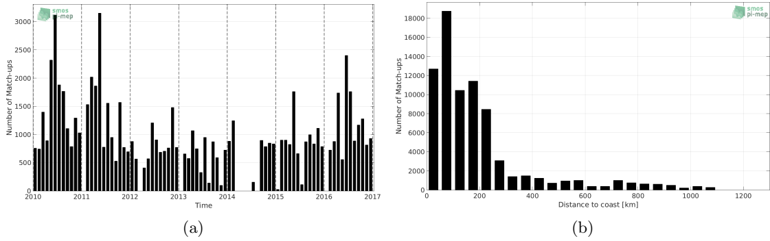
Figure 1: Number of match-ups between TSG-LEGOS-DM and SMOS-L3-CATDS-CECOS-LOCEAN-V3-18DAYS-25KM SSS as a function of time (a) and as function of the distance to coast (b) over the South Atlantic Ocean Pi-MEP region and for the full satellite product period.
