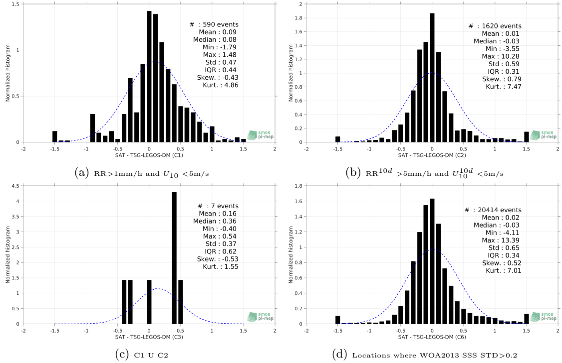
Figure 13: Normalized histogram of \Delta SSS (SMOS-L3-CATDS-CECOS-LOCEAN-V3-18DAYS-25KM - TSG-LEGOS-DM) for 6 different subdatasets corresponding to: RR > 1\text{mm/h} and U_{10} < 5\text{m/s} (a), RR^{10d} > 5\text{mm/h} and U_{10}^{10d} < 5\text{m/s} (b), C1 U C2 (c), Locations where WOA2013 SSS STD > 0.2 (d).
