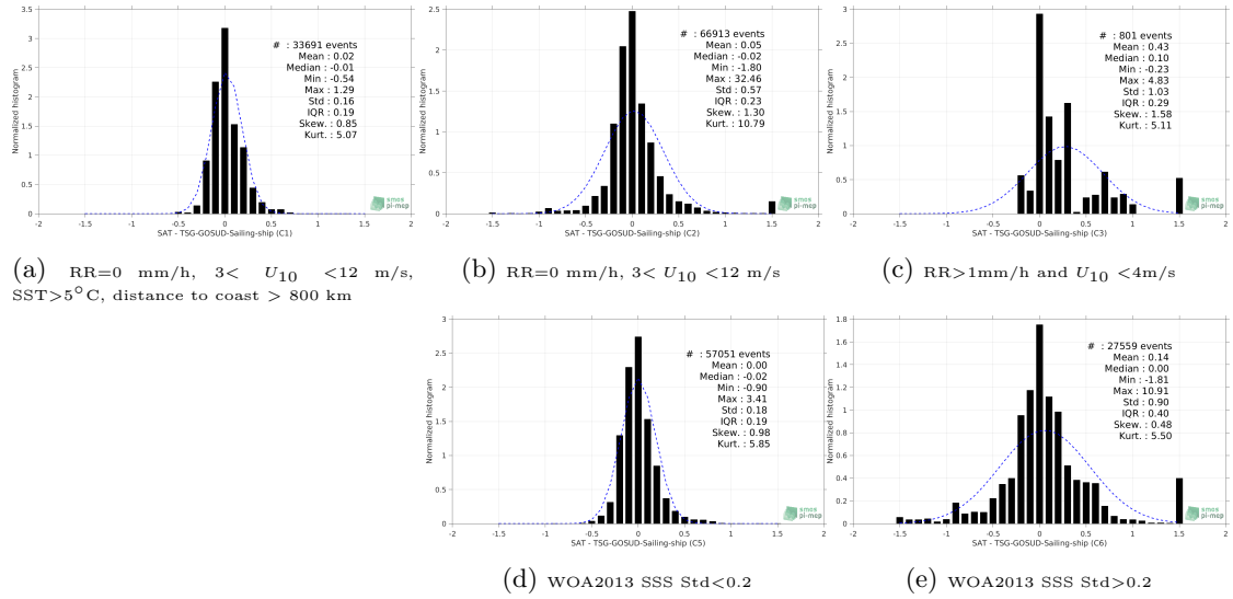
Figure 13: Normalized histogram of \Delta SSS (SMOS-L3-CATDS-CECOS-LOCEAN-V3-18DAYS-25KM - TSG-GOSUD-Sailing-ship) for 5 different subdatasets corresponding to: RR=0 mm/h, 3 < U_{10} < 12 m/s, SST > 5°C, distance to coast > 800 km (a), RR=0 mm/h, 3 < U_{10} < 12 m/s (b), RR > 1mm/h and U_{10} < 4 m/s (c), WOA2013 SSS Std < 0.2 (d), WOA2013 SSS Std > 0.2 (e).
