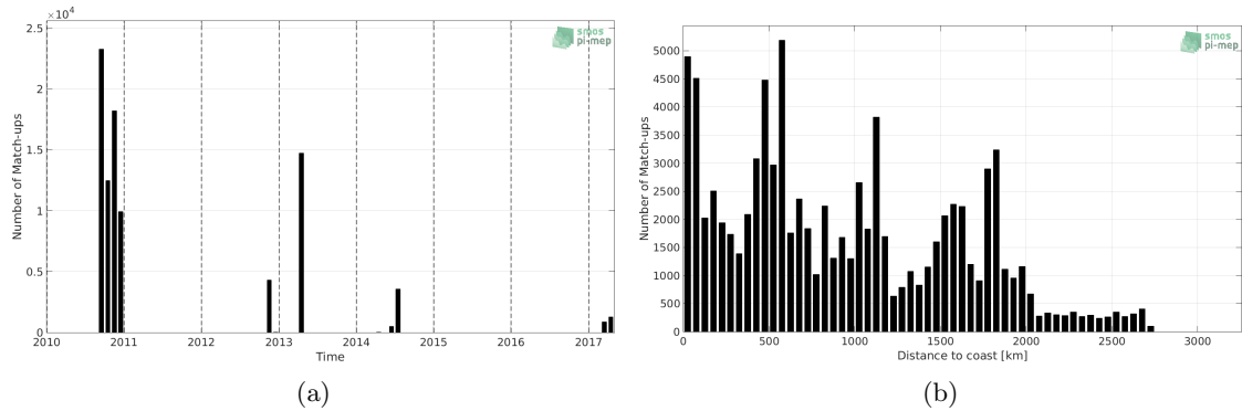
Figure 1: Number of match-ups between TSG-GOSUD-Sailing-ship and SMOS-L3-CATDS-CECOS-LOCEAN-V3-18DAYS-25KM SSS as a function of time (a) and as function of the distance to coast (b) over the South Atlantic Ocean Pi-MEP region and for the full satellite product period.
