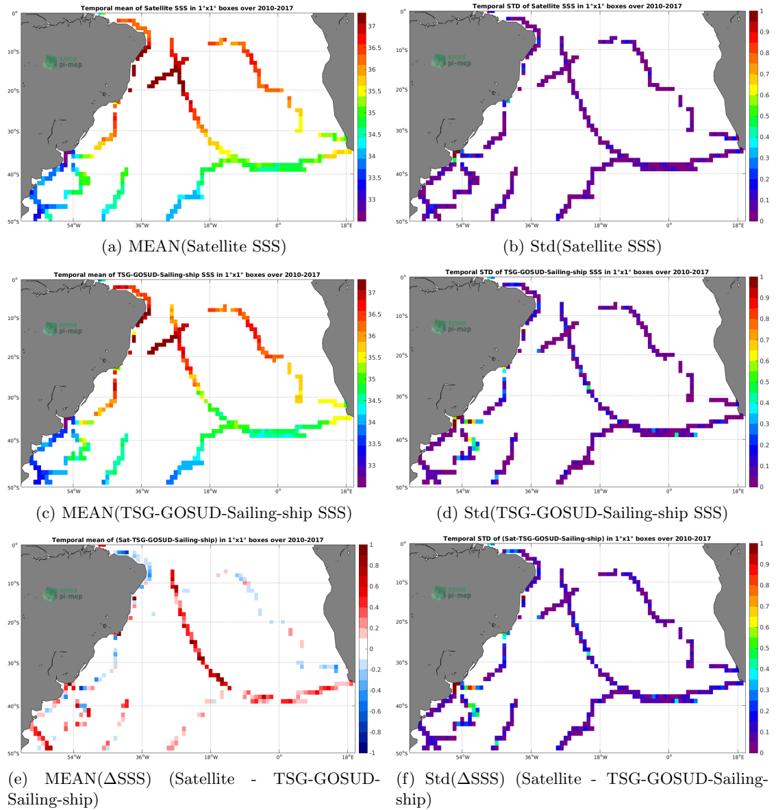
Figure 6: Temporal mean (left) and Std (right) of SSS from SMOS-L3-CATDS-CECOS-LOCEAN-V3-18DAYS-25KM (top), TSG-GOSUD-Sailing-ship (middle), and of \Delta SSS (Satellite - TSG-GOSUD-Sailing-ship). Only match-up pairs are used to generate these maps.
