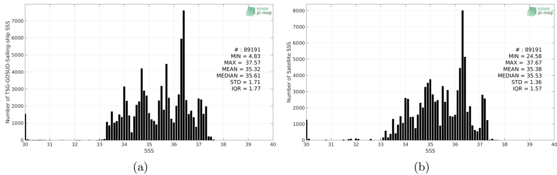
Figure 2: Histograms of SSS from TSG-GOSUD-Sailing-ship (a) and SMOS-L3-CATDS-CECOS-LOCEAN-V3-18DAYS-25KM (b) considering all match-up pairs per bins of 0.1 over the South Atlantic Ocean Pi-MEP region and for the full satellite product period.
