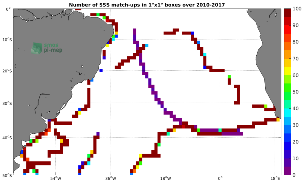
Figure 4: Number of SSS match-ups between TSG-GOSUD-Sailing-ship SSS and the SMOS-L3-CATDS-CECOS-LOCEAN-V3-18DAYS-25KM SSS product for the South Atlantic Ocean Pi-MEP region over 1^\circ \times 1^\circ boxes and for the full satellite product period.
