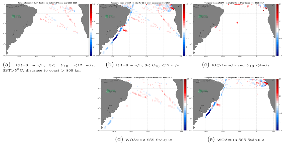
Figure 12: Temporal mean gridded over spatial boxes of size 1^\circ \times 1^\circ of \Delta SSS (SMOS-L3-CATDS-CECOS-LOCEAN-V3-18DAYS-25KM - TSG-GOSUD-Research-vessel) for 5 different subdatasets corresponding to:RR=0 mm/h, 3 < U_{10} < 12 m/s, SST >5^\circ\text{C} , distance to coast > 800 km (a), RR=0 mm/h, 3 < U_{10} < 12 m/s (b), RR >1 mm/h and U_{10} < 4 m/s (c), WOA2013 SSS Std <0.2 (d), WOA2013 SSS Std >0.2 (e).
