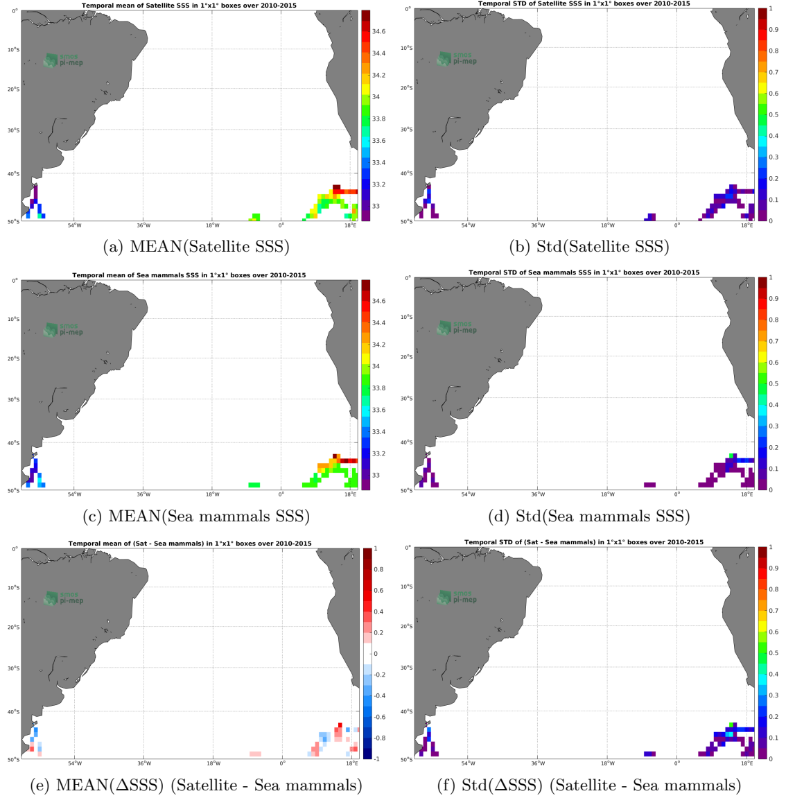
Figure 6: Temporal mean (left) and Std (right) of SSS from SMOS-L3-CATDS-CECOS-LOCEAN-V3-18DAYS-25KM (top), Sea mammals (middle), and of \Delta SSS (Satellite - Sea mammals). Only match-up pairs are used to generate these maps.
