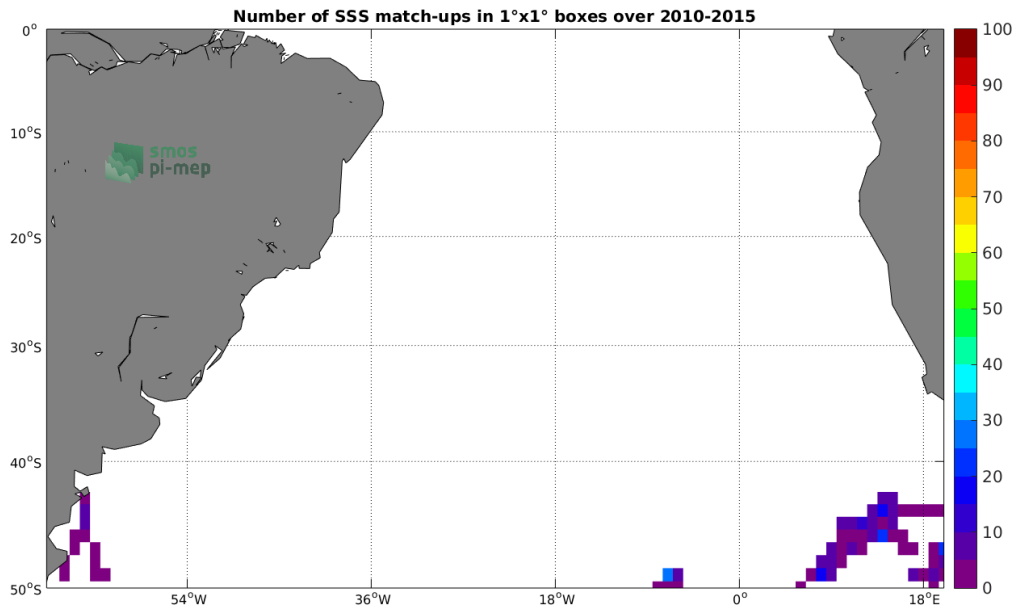
Figure 4: Number of SSS match-ups between Sea mammals SSS and the SMOS-L3-CATDS-CECOS-LOCEAN-V3-18DAYS-25KM SSS product for the South Atlantic Ocean Pi-MEP region over 1°x1° boxes and for the full satellite product period.
