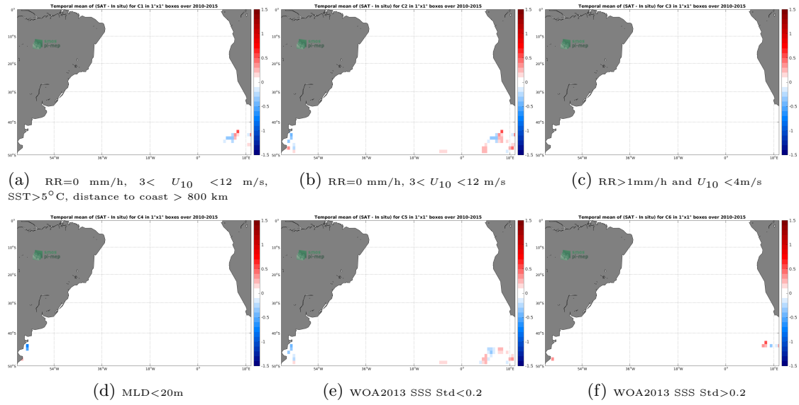
Figure 12: Temporal mean gridded over spatial boxes of size 1^\circ \times 1^\circ of \Delta SSS (SMOS-L3-CATDS-CECOS-LOCEAN-V3-18DAYS-25KM - Sea mammals) for 6 different subdatasets corresponding to: RR=0 mm/h, 3 < U_{10} < 12 m/s, SST > 5^\circ C , distance to coast > 800 km (a), RR=0 mm/h, 3 < U_{10} < 12 m/s (b), RR > 1 mm/h and U_{10} < 4 m/s (c), MLD < 20 m (d), WOA2013 SSS Std < 0.2 (e), WOA2013 SSS Std > 0.2 (f).
