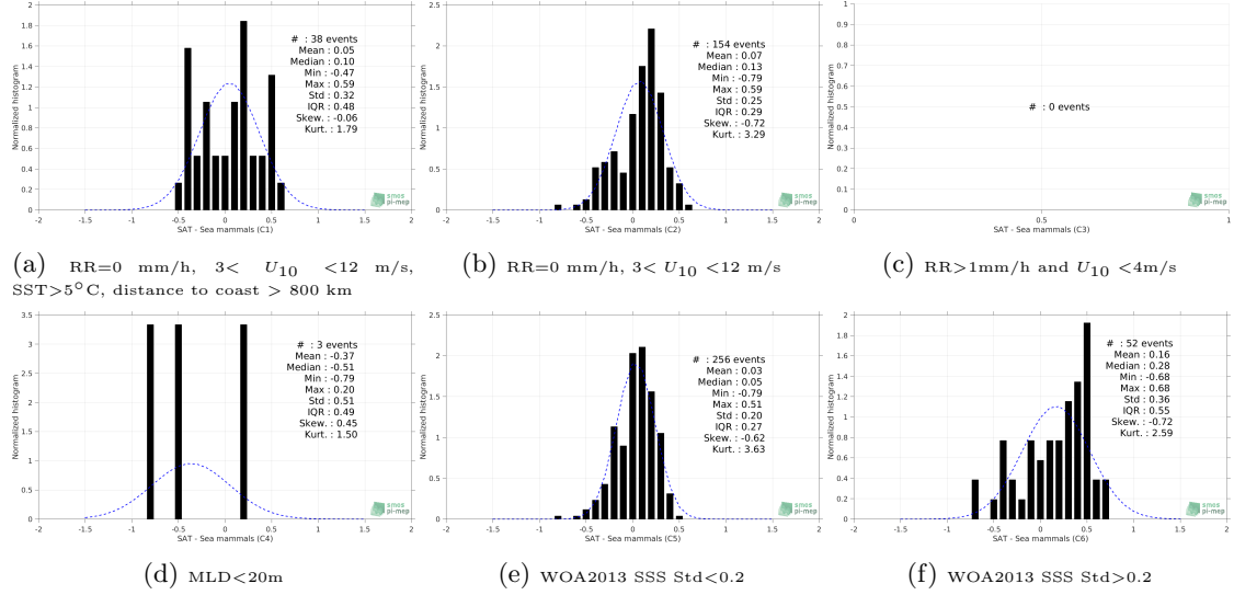
Figure 13: Normalized histogram of \Delta SSS (SMOS-L3-CATDS-CECOS-LOCEAN-V3-18DAYS-25KM - Sea mammals) for 6 different subdatasets corresponding to: RR=0 mm/h, 3 < U_{10} < 12 m/s, SST > 5^\circ\text{C} , distance to coast > 800 km (a), RR=0 mm/h, 3 < U_{10} < 12 m/s (b), RR > 1 mm/h and U_{10} < 4 m/s (c), MLD < 20 m (d), WOA2013 SSS Std < 0.2 (e), WOA2013 SSS Std > 0.2 (f).
