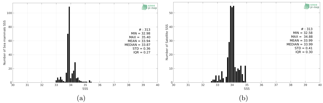
Figure 2: Histograms of SSS from Sea mammals (a) and SMOS-L3-CATDS-CECOS-LOCEAN-V3-18DAYS-25KM (b) considering all match-up pairs per bins of 0.1 over the South Atlantic Ocean Pi-MEP region and for the full satellite product period.
