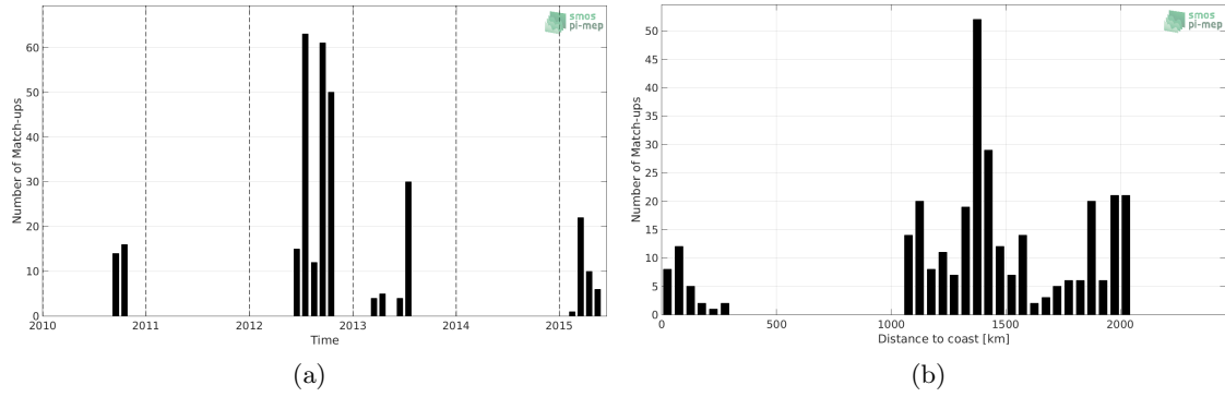
Figure 1: Number of match-ups between Sea mammals and SMOS-L3-CATDS-CECOS-LOCEAN-V3-18DAYS-25KM SSS as a function of time (a) and as function of the distance to coast (b) over the South Atlantic Ocean Pi-MEP region and for the full satellite product period.
