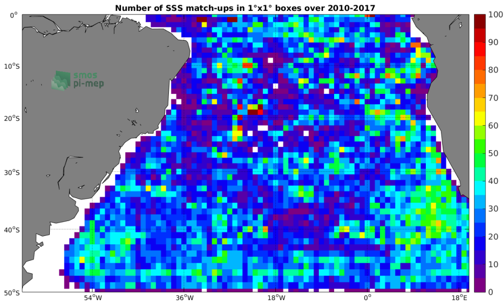
Figure 4: Number of SSS match-ups between Argo SSS and the SMOS-L3-CATDS-CECOS-LOCEAN-V3-18DAYS-25KM SSS product for the South Atlantic Ocean Pi-MEP region over 1^\circ \times 1^\circ boxes and for the full satellite product period.
