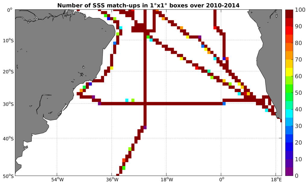
Figure 4: Number of SSS match-ups between TSG-SAMOS SSS and the SMOS-L3-CATDS-CECOS-LOCEAN-V2.1-9DAYS-25KM SSS product for the South Atlantic Ocean Pi-MEP region over 1°x1° boxes and for the full satellite product period.
