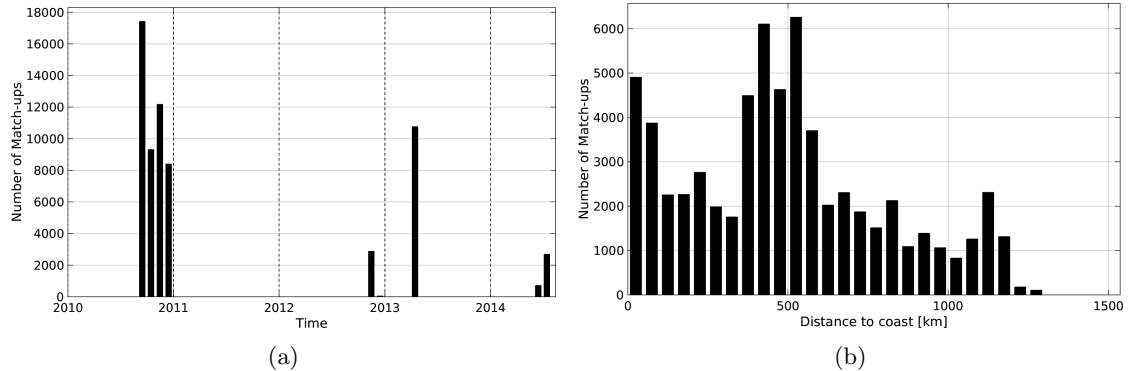
Figure 1: Number of match-ups between TSG-GOSUD-Sailing-ship and SMOS-L3-CATDS-CECOS-LOCEAN-V2.1-9DAYS-25KM SSS as a function of time (a) and as function of the distance to coast (b) over the South Atlantic Ocean Pi-MEP region and for the full satellite product period.
