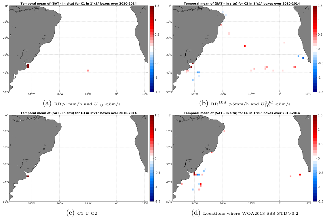
Figure 12: Temporal mean gridded over spatial boxes of size 1^\circ \times 1^\circ of \Delta SSS (SMOS-L3-CATDS-CECOS-LOCEAN-V2.1-9DAYS-25KM - TSG-GOSUD-Sailing-ship) for 4 different subdatasets corresponding to: RR > 1\text{mm/h} and U_{10} < 5\text{m/s} (a), RR^{10d} > 5\text{mm/h} and U_{10}^{10d} < 5\text{m/s} (b), C1 U C2 (c), Locations where WOA2013 SSS STD > 0.2 (d).
