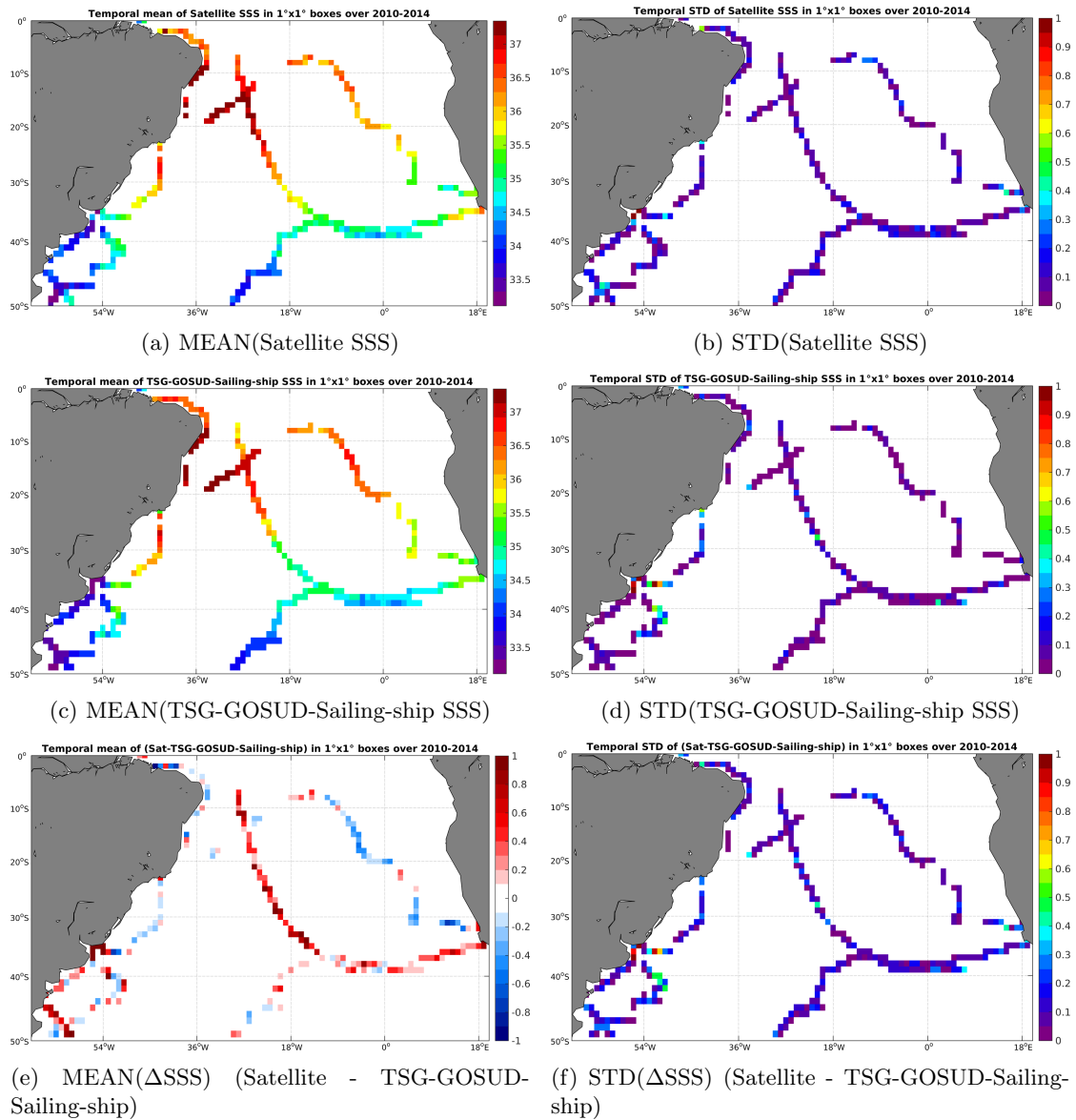
Figure 6: Temporal mean (left) and STD (right) of SSS from SMOS-L3-CATDS-CECOS-LOCEAN-V2.1-9DAYS-25KM (top), TSG-GOSUD-Sailing-ship (middle), and of \Delta SSS (Satellite - TSG-GOSUD-Sailing-ship). Only match-up pairs are used to generate these maps.
