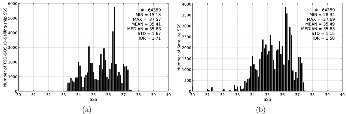
Figure 2: Histograms of SSS from TSG-GOSUD-Sailing-ship (a) and SMOS-L3-CATDS-CECOS-LOCEAN-V2.1-9DAYS-25KM (b) considering all match-up pairs per bins of 0.1 over the South Atlantic Ocean Pi-MEP region and for the full satellite product period.
