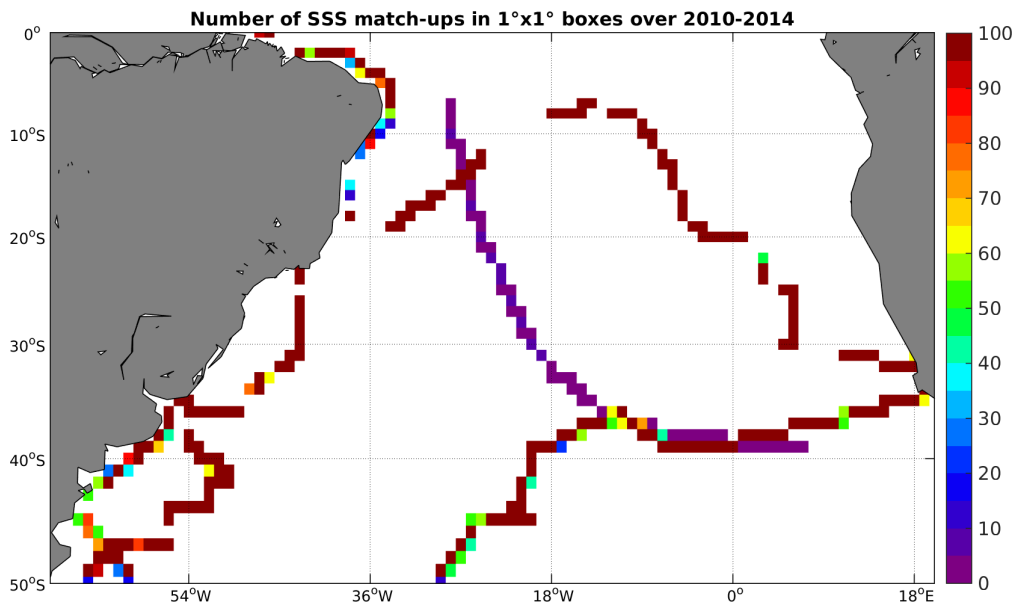
Figure 4: Number of SSS match-ups between TSG-GOSUD-Sailing-ship SSS and the SMOS-L3-CATDS-CECOS-LOCEAN-V2.1-9DAYS-25KM SSS product for the South Atlantic Ocean Pi-MEP region over 1^\circ \times 1^\circ boxes and for the full satellite product period.
