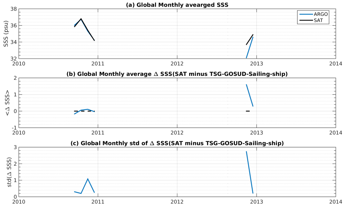
Figure 7: Time series of the monthly averaged mean SSS (top), mean \Delta SSS (Satellite - TSG-GOSUD-Sailing-ship) and STD of \Delta SSS (Satellite - TSG-GOSUD-Sailing-ship) over the South Atlantic Ocean Pi-MEP region considering all match-ups collected by the Pi-MEP platform.
