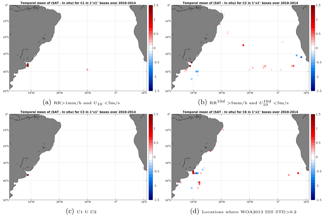
Figure 12: Temporal mean gridded over spatial boxes of size 1°x1° of \Delta SSS (SMOS-L3-CATDS-CECOS-LOCEAN-V2.1-9DAYS-25KM - TSG-GOSUD-Sailing-ship) for 4 different subdatasets corresponding to:RR>1mm/h and U_{10} < 5 m/s (a), RR^{10d} > 5 mm/h and U_{10}^{10d} < 5 m/s (b), C1 U C2 (c),Locations where WOA2013 SSS STD>0.2 (d).
