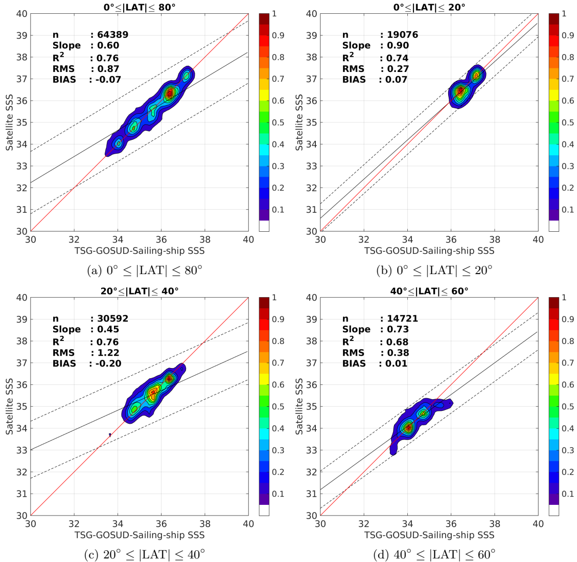
Figure 9: Contour maps of the concentration of SMOS-L3-CATDS-CECOS-LOCEAN-V2.1-9DAYS-25KM SSS (y-axis) versus TSG-GOSUD-Sailing-ship SSS (x-axis) at match-up pairs for different latitude bands. For each plot, the red line shows x=y . The black thin and dashed lines indicate a linear fit through the data cloud and the \pm 95\% confidence levels, respectively. The number match-up pairs n , the slope and R^2 coefficient of the linear fit, the root mean square (RMS) and the mean bias between satellite and in situ data are indicated for each latitude band in each plots.
