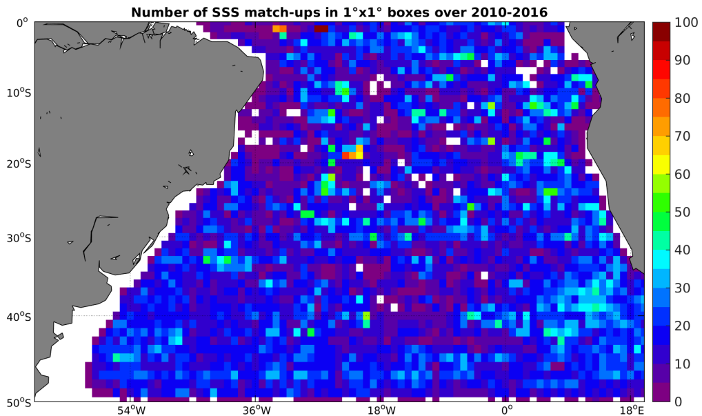
Figure 4: Number of SSS match-ups between Argo SSS and the SMOS-L3-CATDS-CECOS-LOCEAN-V2.1-9DAYS-25KM SSS product for the South Atlantic Ocean Pi-MEP region over 1^\circ \times 1^\circ boxes and for the full satellite product period.
