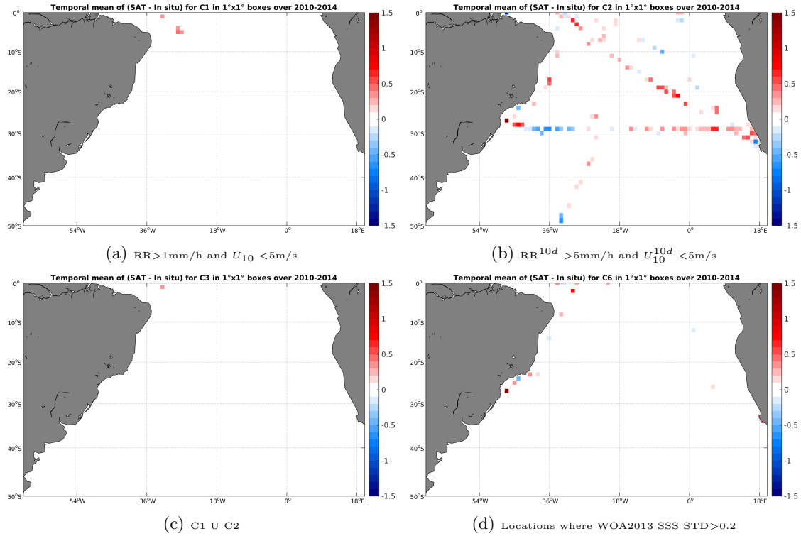
Figure 12: Temporal mean gridded over spatial boxes of size 1^\circ \times 1^\circ of \Delta SSS (SMOS-L3-CATDS-CECOS-LOCEAN-V2-9DAYS-25KM - TSG-SAMOS) for 4 different subdatasets corresponding to: RR > 1mm/h and U_{10} < 5 m/s (a), RR^{10d} > 5 mm/h and U_{10} < 5 m/s (b), C1 U C2 (c), Locations where WOA2013 SSS STD > 0.2 (d).
