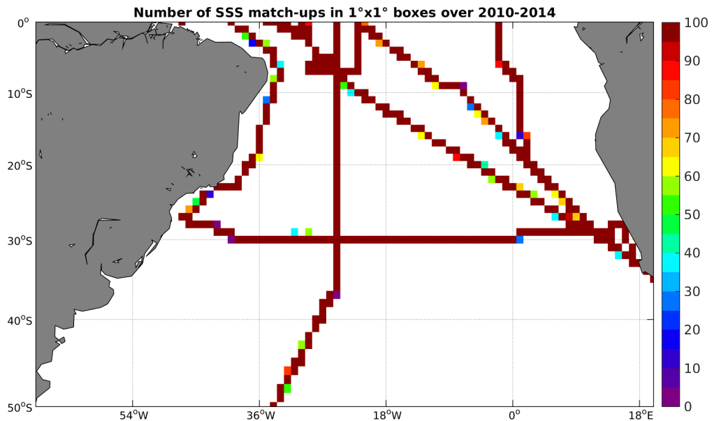
Figure 4: Number of SSS match-ups between TSG-SAMOS SSS and the SMOS-L3-CATDS-CECOS-LOCEAN-V2-9DAYS-25KM SSS product for the South Atlantic Ocean Pi-MEP region over 1^\circ \times 1^\circ boxes and for the full satellite product period.
