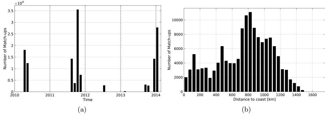
Figure 1: Number of match-ups between TSG-SAMOS and SMOS-L3-CATDS-CECOS-LOCEAN-V2-9DAYS-25KM SSS as a function of time (a) and as function of the distance to coast (b) over the South Atlantic Ocean Pi-MEP region and for the full satellite product period.
