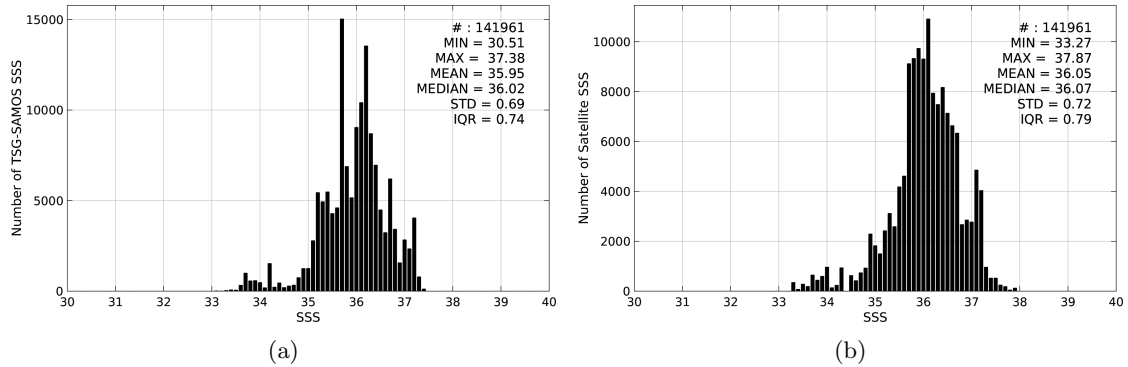
Figure 2: Histograms of SSS from TSG-SAMOS (a) and SMOS-L3-CATDS-CECOS-LOCEAN-V2-9DAYS-25KM (b) considering all match-up pairs per bins of 0.1 over the South Atlantic Ocean Pi-MEP region and for the full satellite product period.
