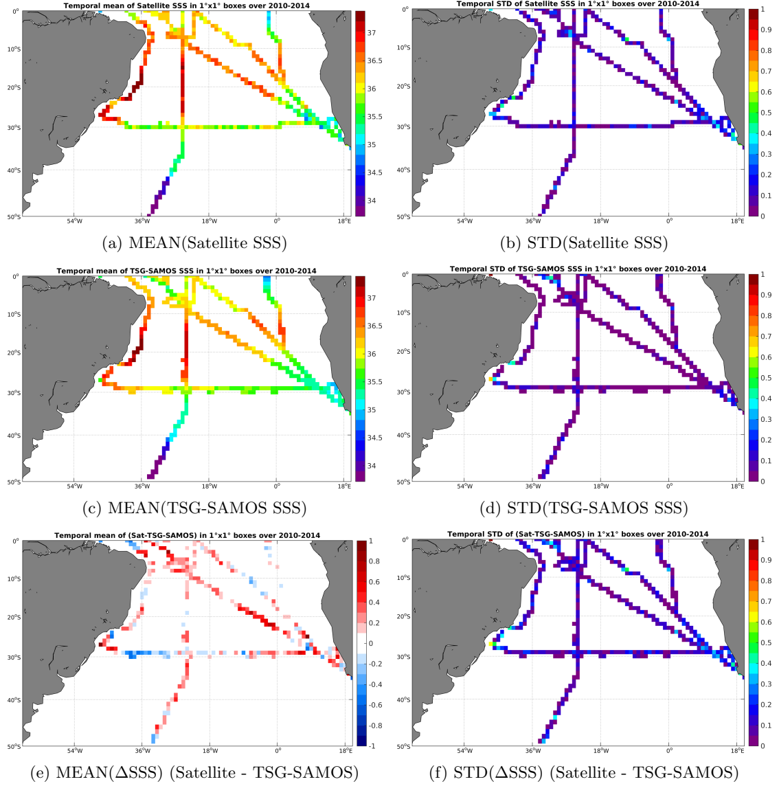
Figure 6: Temporal mean (left) and STD (right) of SSS from SMOS-L3-CATDS-CECOS-LOCEAN-V2-9DAYS-25KM (top), TSG-SAMOS (middle), and of \Delta SSS (Satellite - TSG-SAMOS). Only match-up pairs are used to generate these maps.
