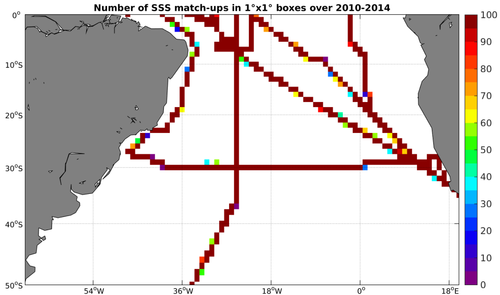
Figure 4: Number of SSS match-ups between TSG-SAMOS SSS and the SMOS-L3-CATDS-CECOS-LOCEAN-V2-9DAYS-25KM SSS product for the South Atlantic Ocean Pi-MEP region over 1^\circ \times 1^\circ boxes and for the full satellite product period.
