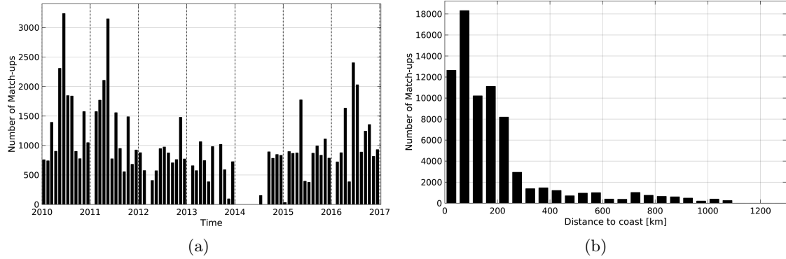
Figure 1: Number of match-ups between TSG-LEGOS-DM and SMOS-L3-CATDS-CECOS-LOCEAN-V2-9DAYS-25KM SSS as a function of time (a) and as function of the distance to coast (b) over the South Atlantic Ocean Pi-MEP region and for the full satellite product period.
