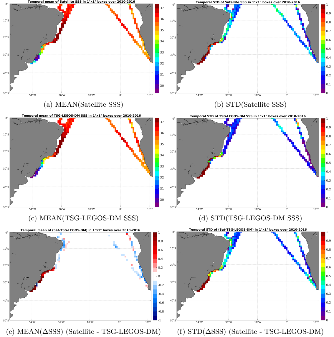
Figure 6: Temporal mean (left) and STD (right) of SSS from SMOS-L3-CATDS-CECOS-LOCEAN-V2-9DAYS-25KM (top), TSG-LEGOS-DM (middle), and of \Delta SSS (Satellite - TSG-LEGOS-DM). Only match-up pairs are used to generate these maps.
