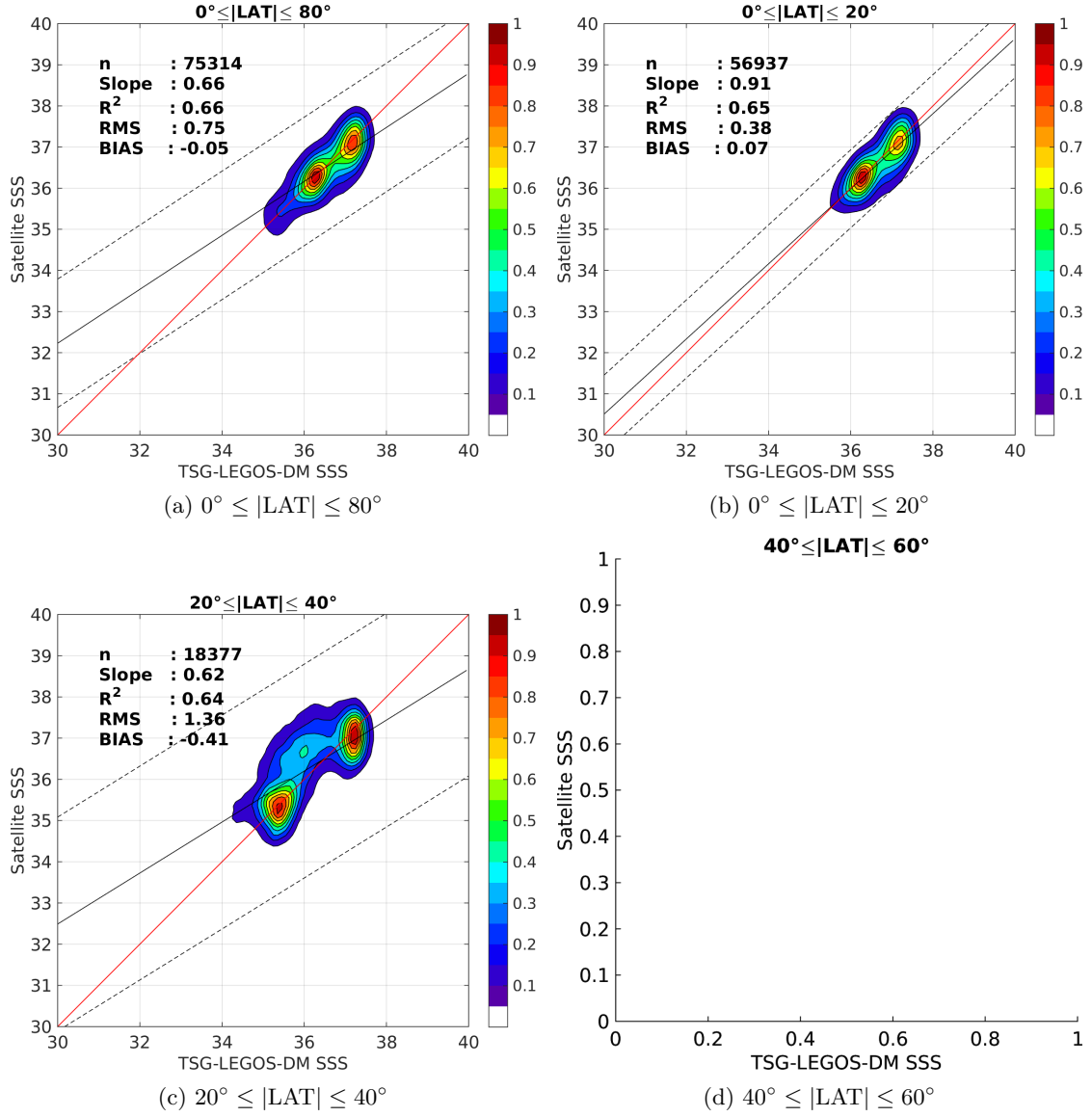
Figure 9: Contour maps of the concentration of SMOS-L3-CATDS-CECOS-LOCEAN-V2-9DAYS-25KM SSS (y-axis) versus TSG-LEGOS-DM SSS (x-axis) at match-up pairs for different latitude bands. For each plot, the red line shows x=y . The black thin and dashed lines indicate a linear fit through the data cloud and the \pm 95\% confidence levels, respectively. The number match-up pairs n , the slope and R^2 coefficient of the linear fit, the root mean square (RMS) and the mean bias between satellite and in situ data are indicated for each latitude band in each plots.
