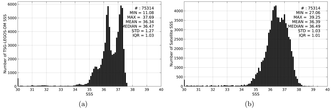
Figure 2: Histograms of SSS from TSG-LEGOS-DM (a) and SMOS-L3-CATDS-CECOS-LOCEAN-V2-9DAYS-25KM (b) considering all match-up pairs per bins of 0.1 over the South Atlantic Ocean Pi-MEP region and for the full satellite product period.
