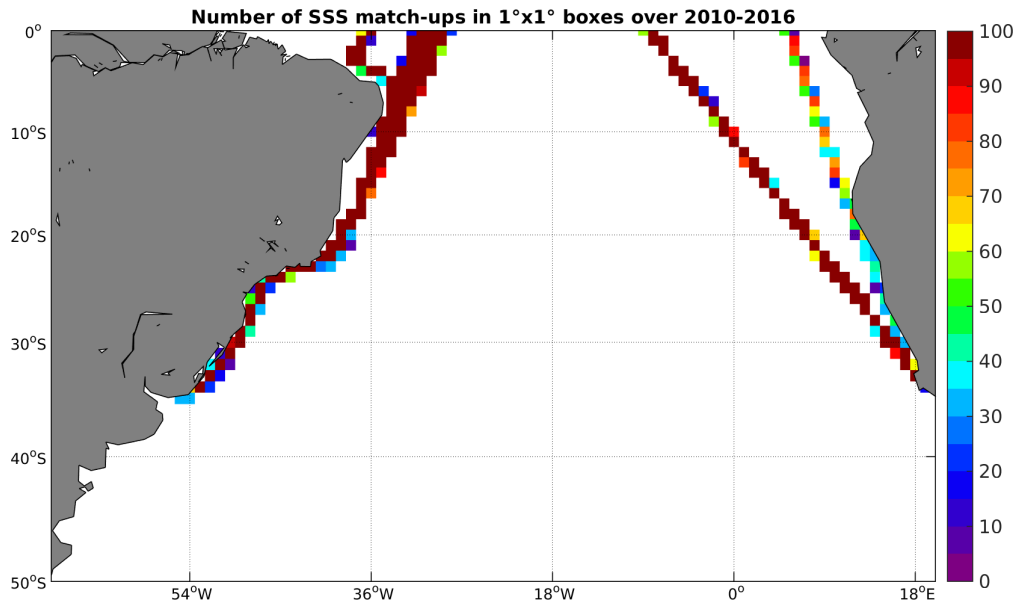
Figure 4: Number of SSS match-ups between TSG-LEGOS-DM SSS and the SMOS-L3-CATDS-CECOS-LOCEAN-V2-9DAYS-25KM SSS product for the South Atlantic Ocean Pi-MEP region over 1^\circ \times 1^\circ boxes and for the full satellite product period.
