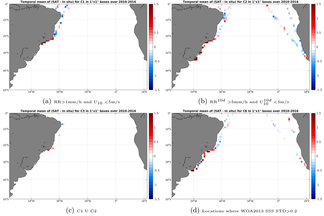
Figure 12: Temporal mean gridded over spatial boxes of size 1^\circ \times 1^\circ of \Delta SSS (SMOS-L3-CATDS-CECOS-LOCEAN-V2-9DAYS-25KM - TSG-LEGOS-DM) for 4 different subdatasets corresponding to: RR > 1\text{mm/h} and U_{10} < 5\text{m/s} (a), RR^{10d} > 5\text{mm/h} and U_{10}^{10d} < 5\text{m/s} (b), C1 \cup C2 (c), Locations where WOA2013 SSS STD > 0.2 (d).
