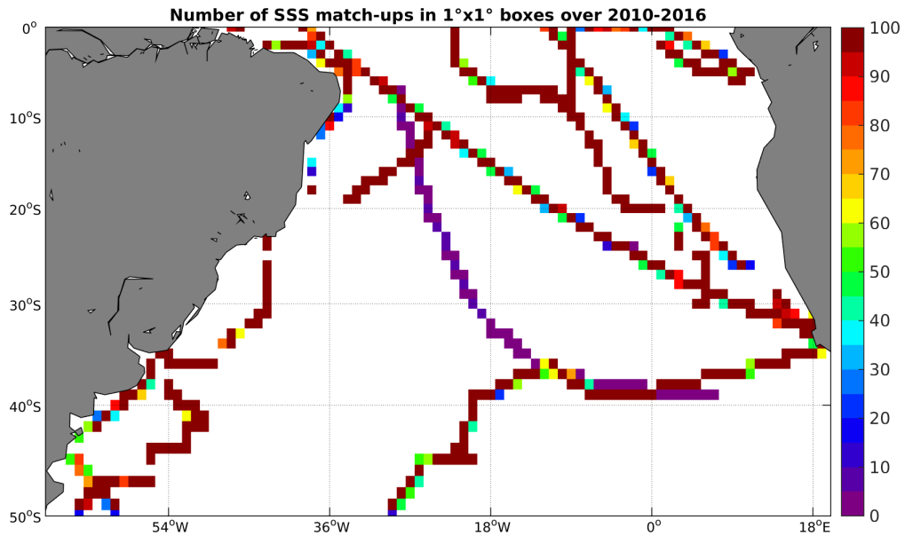
Figure 4: Number of SSS match-ups between TSG-GOSUD-Sailing-ship SSS and the SMOS-L3-CATDS-CECOS-LOCEAN-V2-9DAYS-25KM SSS product for the South Atlantic Ocean Pi-MEP region over 1^\circ \times 1^\circ boxes and for the full satellite product period.
