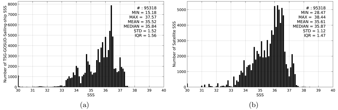
Figure 2: Histograms of SSS from TSG-GOSUD-Sailing-ship (a) and SMOS-L3-CATDS-CECOS-LOCEAN-V2-9DAYS-25KM (b) considering all match-up pairs per bins of 0.1 over the South Atlantic Ocean Pi-MEP region and for the full satellite product period.
