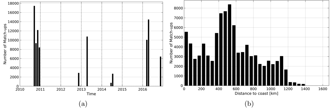
Figure 1: Number of match-ups between TSG-GOSUD-Sailing-ship and SMOS-L3-CATDS-CECOS-LOCEAN-V2-9DAYS-25KM SSS as a function of time (a) and as function of the distance to coast (b) over the South Atlantic Ocean Pi-MEP region and for the full satellite product period.
