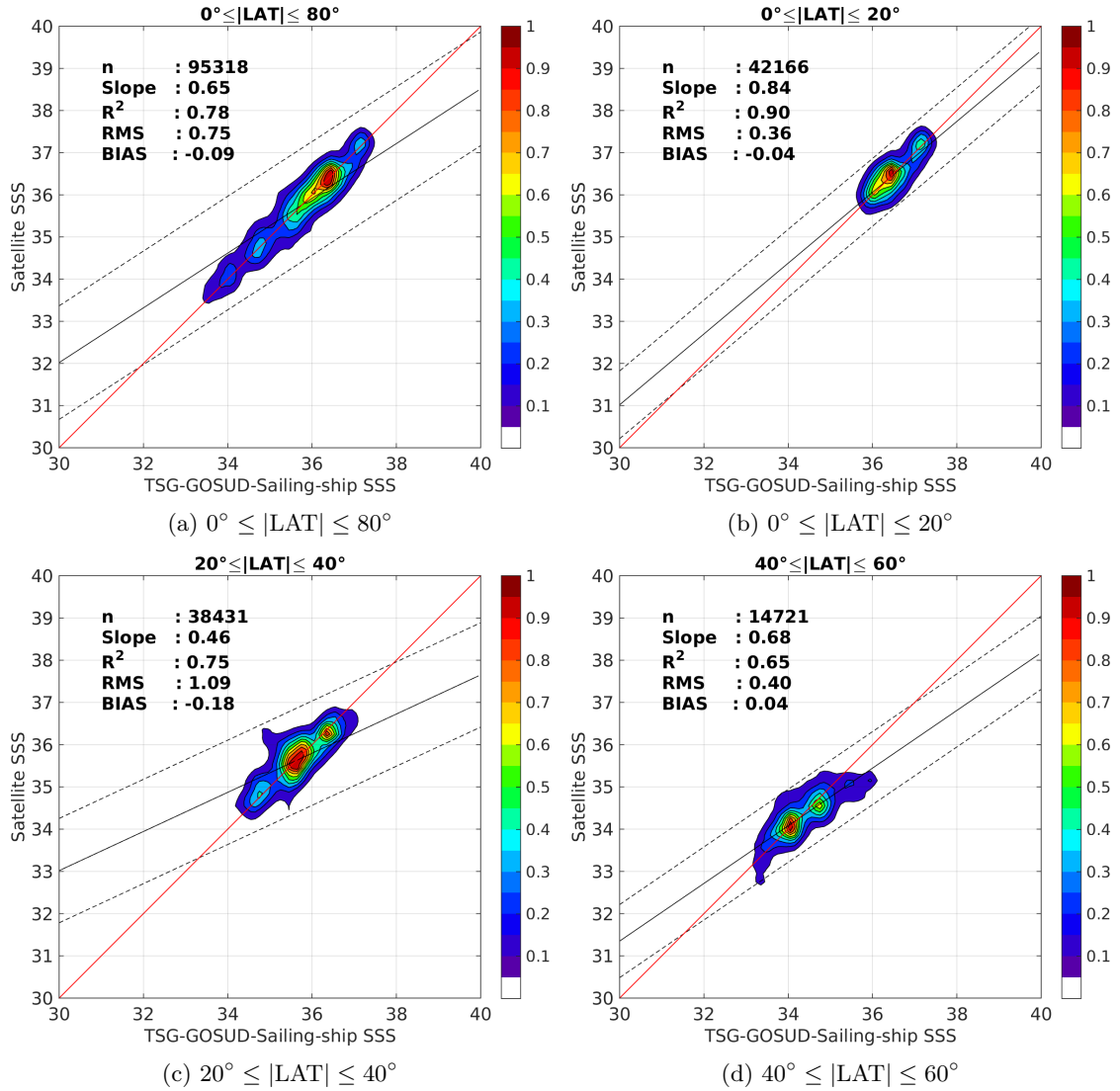
Figure 9: Contour maps of the concentration of SMOS-L3-CATDS-CECOS-LOCEAN-V2-9DAYS-25KM SSS (y-axis) versus TSG-GOSUD-Sailing-ship SSS (x-axis) at match-up pairs for different latitude bands. For each plot, the red line shows x=y . The black thin and dashed lines indicate a linear fit through the data cloud and the \pm 95\% confidence levels, respectively. The number match-up pairs n , the slope and R^2 coefficient of the linear fit, the root mean square (RMS) and the mean bias between satellite and in situ data are indicated for each latitude band in each plots.
