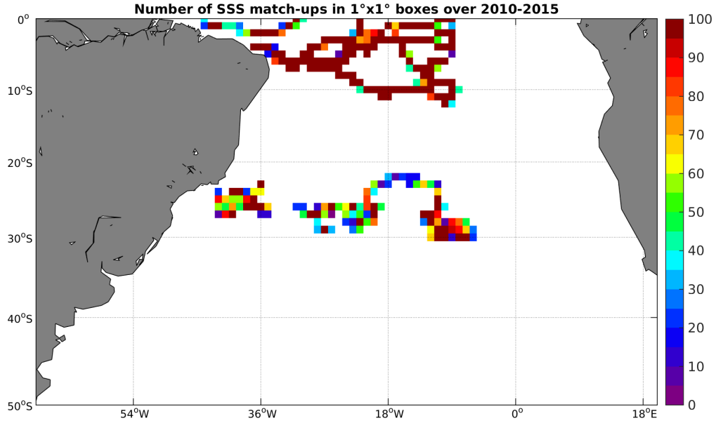
Figure 3: Number of SSS match-ups between Surface drifters SSS and the SMOS-L3-CATDS-CECOS-LOCEAN-V2-9DAYS-25KM SSS product for the South Atlantic Ocean Pi-MEP region over 1^\circ \times 1^\circ boxes and for the full satellite product period.
