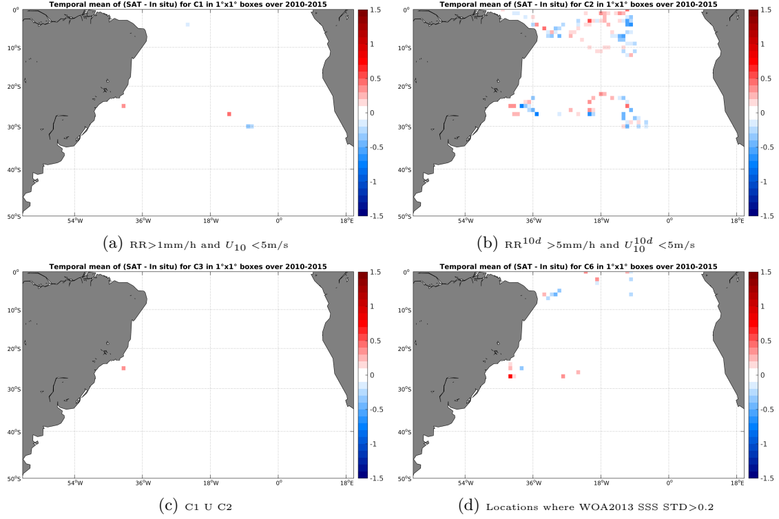
Figure 11: Temporal mean gridded over spatial boxes of size 1^\circ \times 1^\circ of \Delta SSS (SMOS-L3-CATDS-CECOS-LOCEAN-V2-9DAYS-25KM - Surface drifters) for 4 different subdatasets corresponding to: RR > 1mm/h and U_{10} < 5 m/s (a), RR^{10d} > 5 mm/h and U_{10}^{10d} < 5 m/s (b), C1 U C2 (c), Locations where WOA2013 SSS STD > 0.2 (d).
