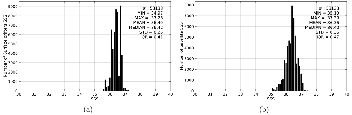
Figure 2: Histograms of SSS from Surface drifters (a) and SMOS-L3-CATDS-CECOS-LOCEAN-V2-9DAYS-25KM (b) considering all match-up pairs per bins of 0.1 over the South Atlantic Ocean Pi-MEP region and for the full satellite product period.
