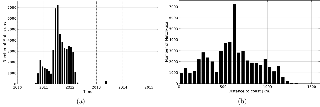
Figure 1: Number of match-ups between Surface drifters and SMOS-L3-CATDS-CECOS-LOCEAN-V2-9DAYS-25KM SSS as a function of time (a) and as function of the distance to coast (b) over the South Atlantic Ocean Pi-MEP region and for the full satellite product period.
