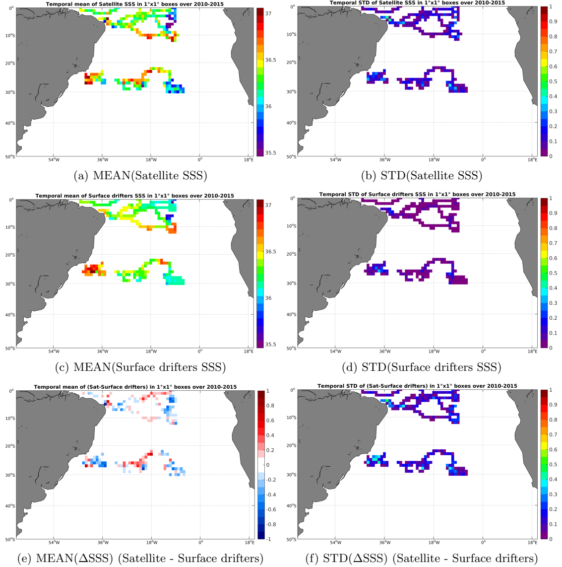
Figure 5: Temporal mean (left) and STD (right) of SSS from SMOS-L3-CATDS-CECOS-LOCEAN-V2-9DAYS-25KM (top), Surface drifters (middle), and of \Delta SSS (Satellite - Surface drifters). Only match-up pairs are used to generate these maps.
