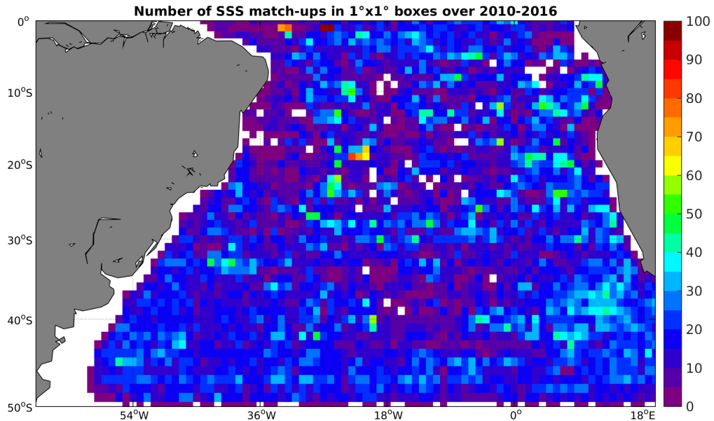
Figure 4: Number of SSS match-ups between Argo SSS and the SMOS-L3-CATDS-CECOS-LOCEAN-V2-9DAYS-25KM SSS product for the South Atlantic Ocean Pi-MEP region over 1^\circ \times 1^\circ boxes and for the full satellite product period.
