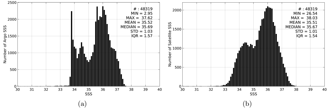
Figure 2: Histograms of SSS from Argo (a) and SMOS-L3-CATDS-CECOS-LOCEAN-V2-9DAYS-25KM (b) considering all match-up pairs per bins of 0.1 over the South Atlantic Ocean Pi-MEP region and for the full satellite product period.
