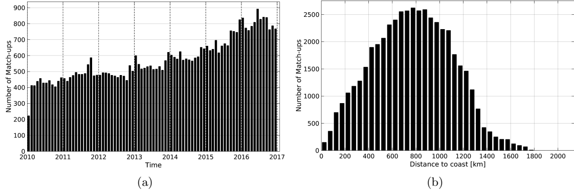
Figure 1: Number of match-ups between Argo and SMOS-L3-CATDS-CECOS-LOCEAN-V2-9DAYS-25KM SSS as a function of time (a) and as function of the distance to coast (b) over the South Atlantic Ocean Pi-MEP region and for the full satellite product period.
