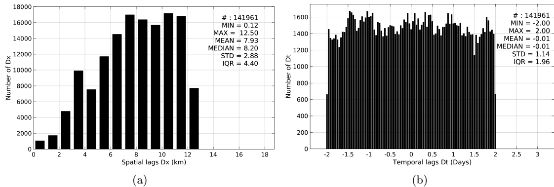
Figure 5: Histograms of the spatial (a) and temporal (b) lags between the time of the TSG-SAMOS measurements and the date of the corresponding SMOS-L3-CATDS-CECOS-LOCEAN-V2-18DAYS-25KM SSS product.
