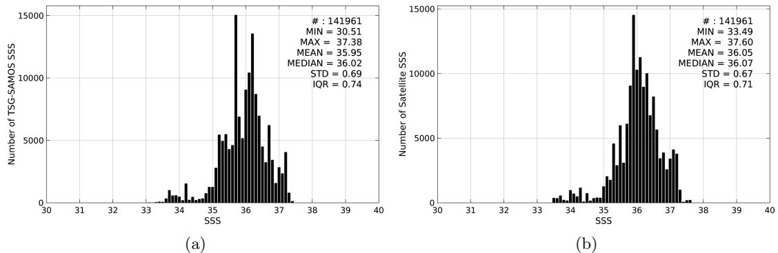
Figure 2: Histograms of SSS from TSG-SAMOS (a) and SMOS-L3-CATDS-CECOS-LOCEAN-V2-18DAYS-25KM (b) considering all match-up pairs per bins of 0.1 over the South Atlantic Ocean Pi-MEP region and for the full satellite product period.
