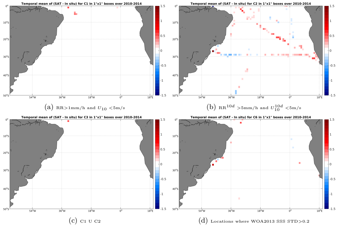
Figure 12: Temporal mean gridded over spatial boxes of size 1^\circ \times 1^\circ of \Delta SSS (SMOS-L3-CATDS-CECOS-LOCEAN-V2-18DAYS-25KM - TSG-SAMOS) for 4 different subdatasets corresponding to: RR > 1\text{mm/h} and U_{10} < 5\text{m/s} (a), RR^{10d} > 5\text{mm/h} and U_{10}^{10d} < 5\text{m/s} (b), C1 U C2 (c), Locations where WOA2013 SSS STD > 0.2 (d).
