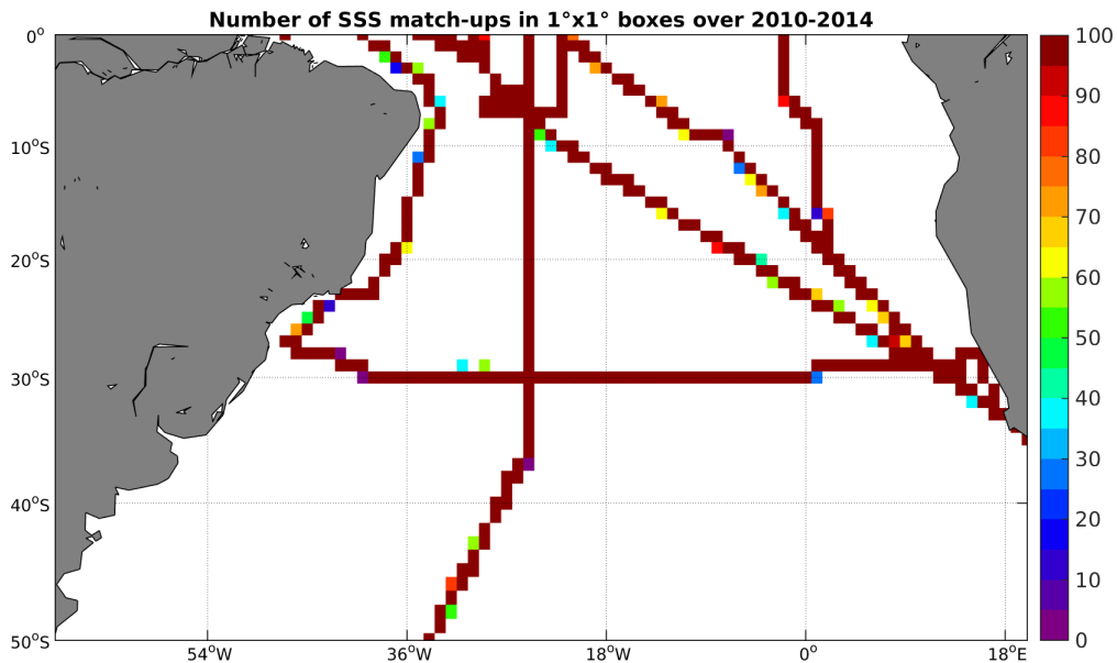
Figure 4: Number of SSS match-ups between TSG-SAMOS SSS and the SMOS-L3-CATDS-CECOS-LOCEAN-V2-18DAYS-25KM SSS product for the South Atlantic Ocean Pi-MEP region over 1^{\circ} \times 1^{\circ} boxes and for the full satellite product period.
