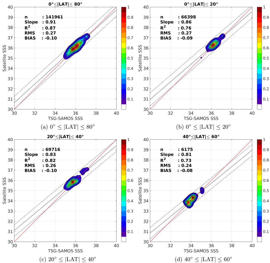
Figure 9: Contour maps of the concentration of SMOS-L3-CATDS-CECOS-LOCEAN-V2-18DAYS-25KM SSS (y-axis) versus TSG-SAMOS SSS (x-axis) at match-up pairs for different latitude bands. For each plot, the red line shows x=y . The black thin and dashed lines indicate a linear fit through the data cloud and the \pm 95\% confidence levels, respectively. The number match-up pairs n , the slope and R^2 coefficient of the linear fit, the root mean square (RMS) and the mean bias between satellite and in situ data are indicated for each latitude band in each plots.
