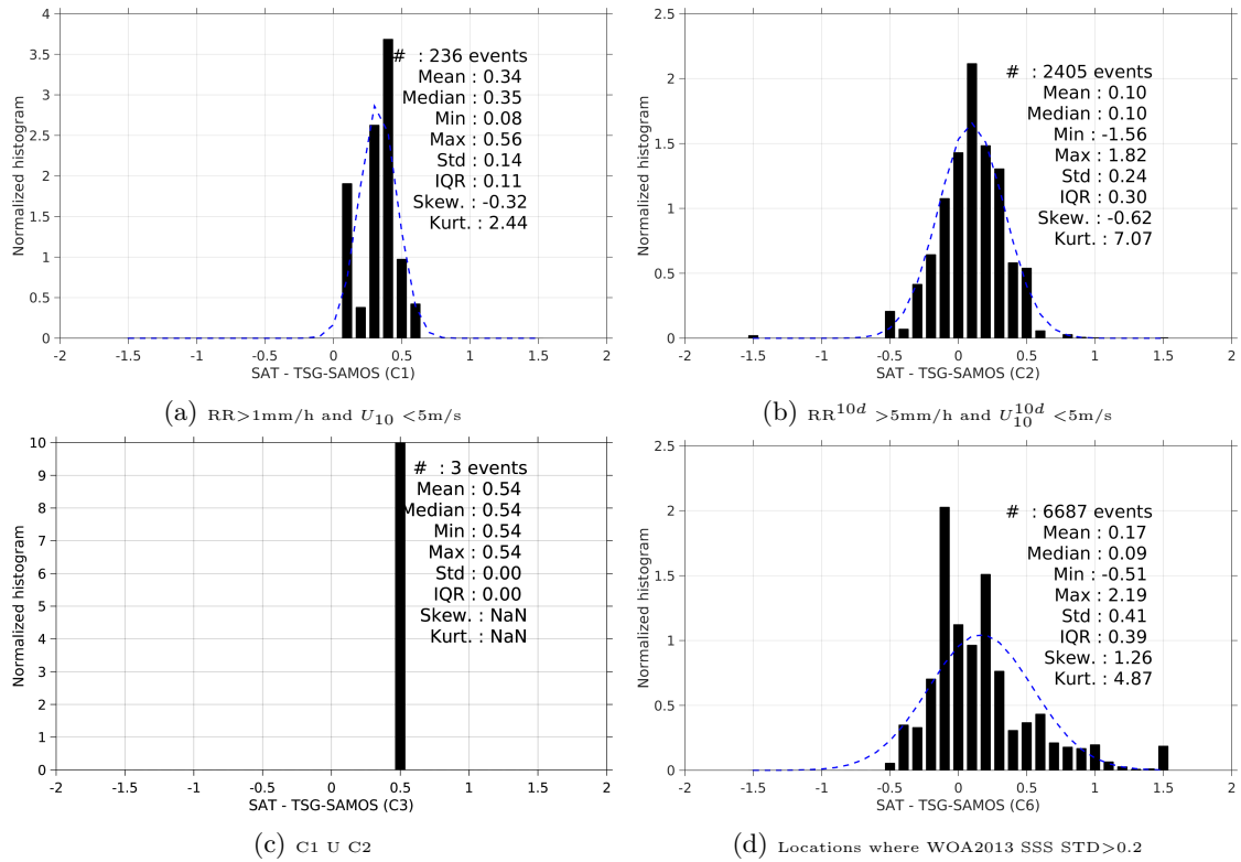
Figure 13: Normalized histogram of \Delta SSS (SMOS-L3-CATDS-CECOS-LOCEAN-V2-18DAYS-25KM - TSG-SAMOS) for 6 different subdatasets corresponding to: RR > 1mm/h and U_{10} < 5 m/s (a), RR^{10d} > 5 mm/h and U_{10}^{10d} < 5 m/s (b), C1 U C2 (c), Locations where WOA2013 SSS STD > 0.2 (d).
