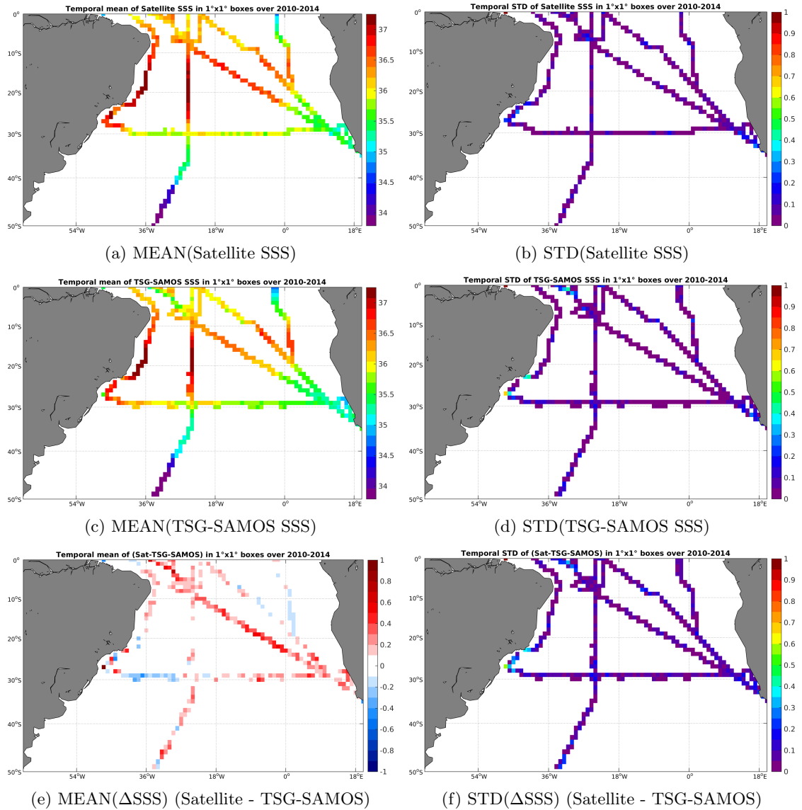
Figure 6: Temporal mean (left) and STD (right) of SSS from SMOS-L3-CATDS-CECOS-LOCEAN-V2-18DAYS-25KM (top), TSG-SAMOS (middle), and of \Delta SSS (Satellite - TSG-SAMOS). Only match-up pairs are used to generate these maps.
