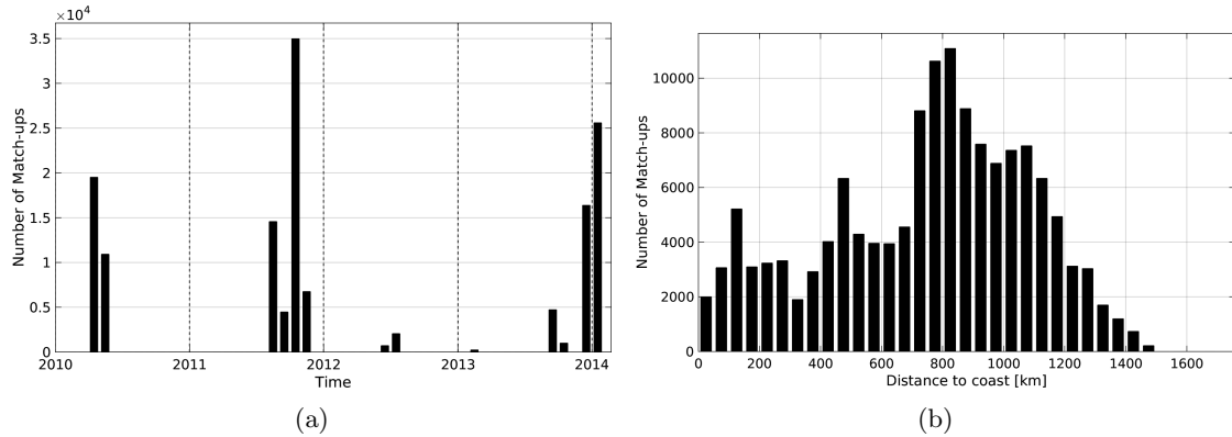
Figure 1: Number of match-ups between TSG-SAMOS and SMOS-L3-CATDS-CECOS-LOCEAN-V2-18DAYS-25KM SSS as a function of time (a) and as function of the distance to coast (b) over the South Atlantic Ocean Pi-MEP region and for the full satellite product period.
