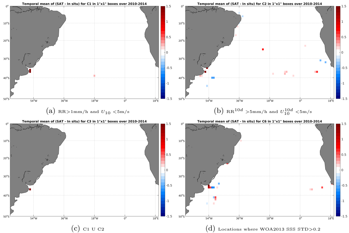
Figure 12: Temporal mean gridded over spatial boxes of size 1°x1° of \Delta SSS (SMOS-L3-CATDS-CECOS-LOCEAN-V2-18DAYS-25KM - TSG-GOSUD-Sailing-ship) for 4 different subdatasets corresponding to:RR>1mm/h and U_{10} < 5 m/s (a), RR^{10d} > 5 mm/h and U_{10}^{10d} < 5 m/s (b), C1 U C2 (c),Locations where WOA2013 SSS STD>0.2 (d).
