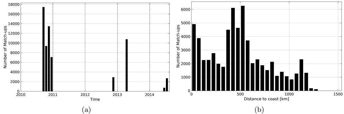
Figure 1: Number of match-ups between TSG-GOSUD-Sailing-ship and SMOS-L3-CATDS-CECOS-LOCEAN-V2-18DAYS-25KM SSS as a function of time (a) and as function of the distance to coast (b) over the South Atlantic Ocean Pi-MEP region and for the full satellite product period.
