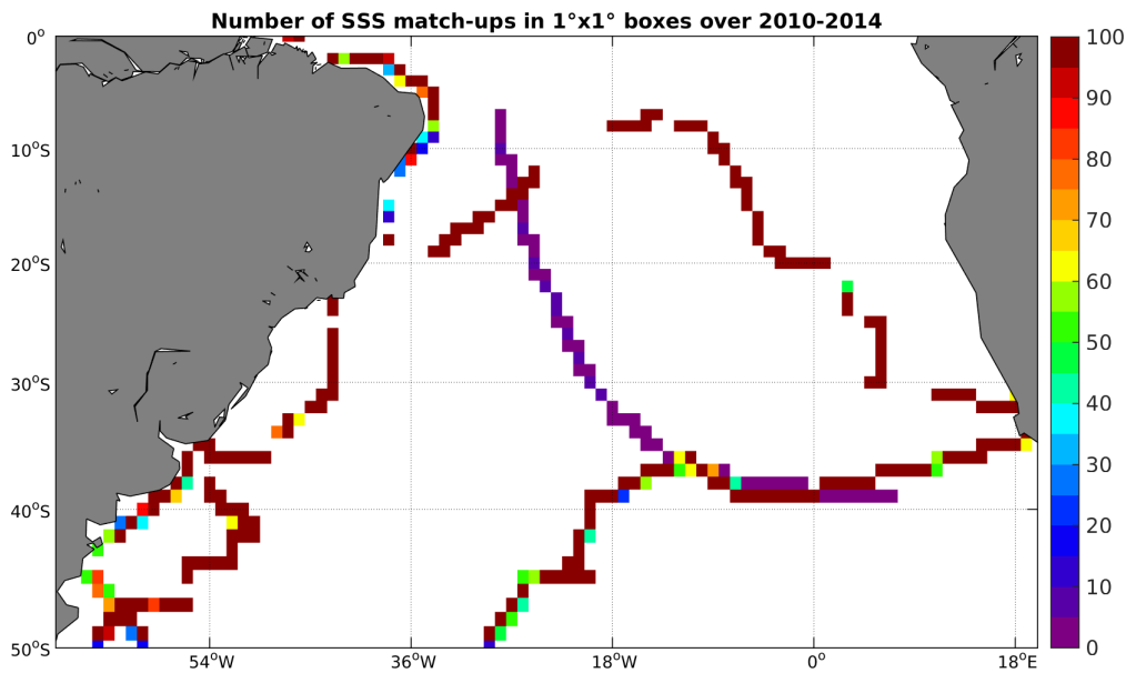
Figure 4: Number of SSS match-ups between TSG-GOSUD-Sailing-ship SSS and the SMOS-L3-CATDS-CECOS-LOCEAN-V2-18DAYS-25KM SSS product for the South Atlantic Ocean Pi-MEP region over 1°x1° boxes and for the full satellite product period.
