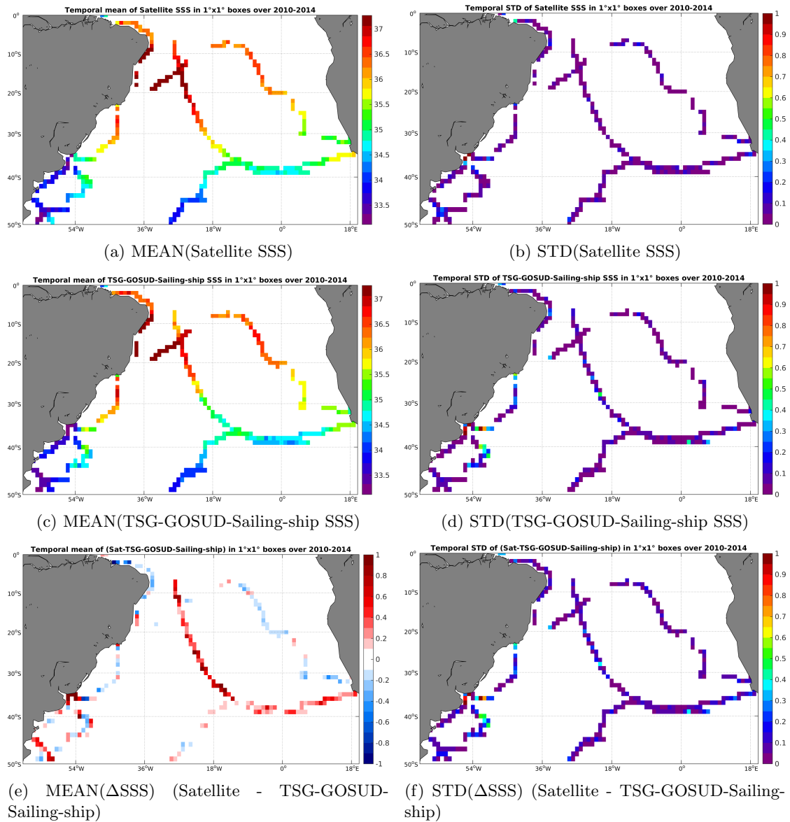
Figure 6: Temporal mean (left) and STD (right) of SSS from SMOS-L3-CATDS-CECOS-LOCEAN-V2-18DAYS-25KM (top), TSG-GOSUD-Sailing-ship (middle), and of \Delta SSS (Satellite - TSG-GOSUD-Sailing-ship). Only match-up pairs are used to generate these maps.
