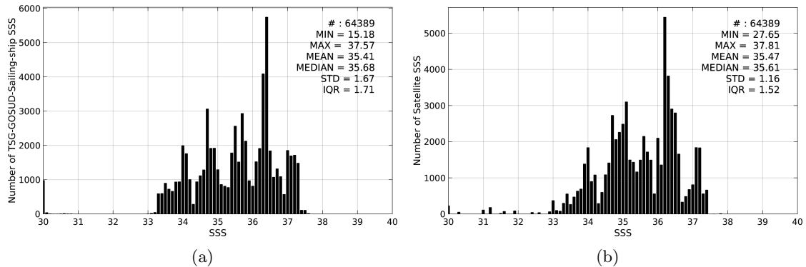
Figure 2: Histograms of SSS from TSG-GOSUD-Sailing-ship (a) and SMOS-L3-CATDS-CECOS-LOCEAN-V2-18DAYS-25KM (b) considering all match-up pairs per bins of 0.1 over the South Atlantic Ocean Pi-MEP region and for the full satellite product period.
