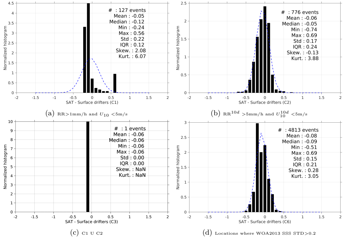
Figure 12: Normalized histogram of \Delta\text{SSS} (SMOS-L3-CATDS-CECOS-LOCEAN-V2-18DAYS-25KM - Surface drifters) for 6 different subdatasets corresponding to: RR > 1mm/h and U_{10} < 5\text{m/s} (a), RR^{10d} > 5\text{mm/h} and U_{10}^{10d} < 5\text{m/s} (b), C1 U C2 (c), Locations where WOA2013 SSS STD > 0.2 (d).
