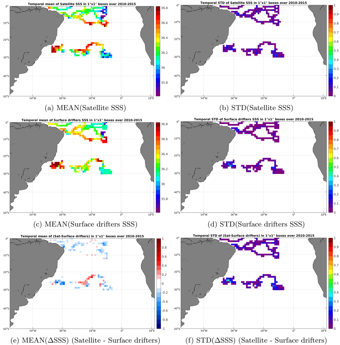
Figure 5: Temporal mean (left) and STD (right) of SSS from SMOS-L3-CATDS-CECOS-LOCEAN-V2-18DAYS-25KM (top), Surface drifters (middle), and of \Delta SSS (Satellite - Surface drifters). Only match-up pairs are used to generate these maps.
