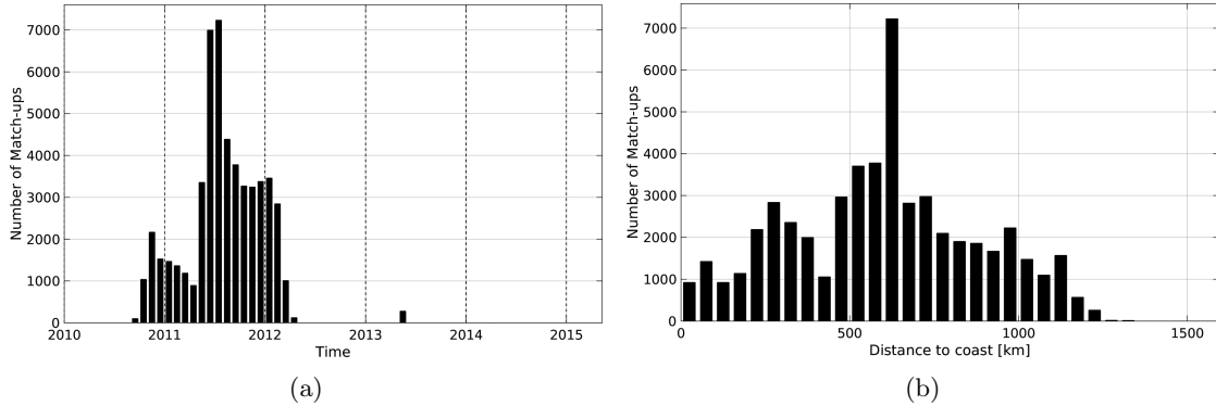
Figure 1: Number of match-ups between Surface drifters and SMOS-L3-CATDS-CECOS-LOCEAN-V2-18DAYS-25KM SSS as a function of time (a) and as function of the distance to coast (b) over the South Atlantic Ocean Pi-MEP region and for the full satellite product period.
