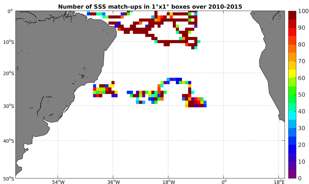
Figure 3: Number of SSS match-ups between Surface drifters SSS and the SMOS-L3-CATDS-CECOS-LOCEAN-V2-18DAYS-25KM SSS product for the South Atlantic Ocean Pi-MEP region over 1°x1° boxes and for the full satellite product period.
