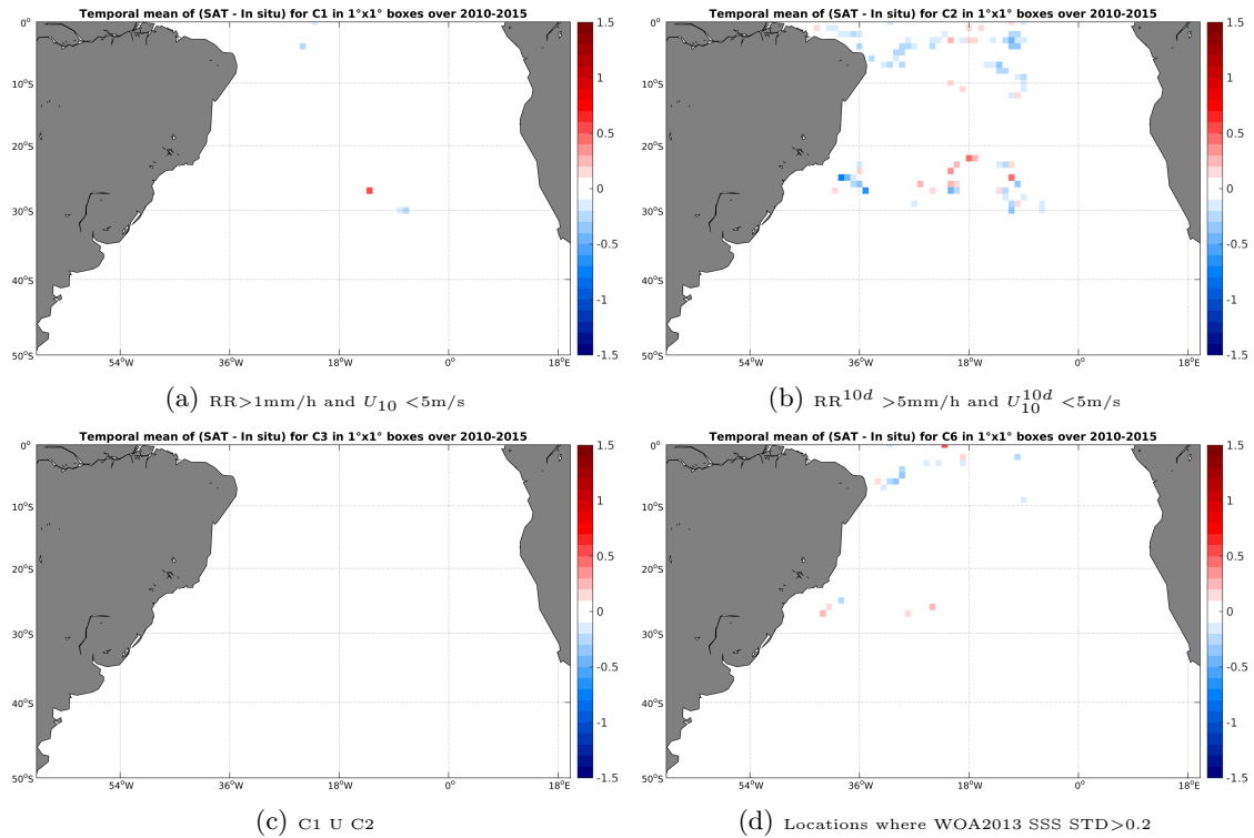
Figure 11: Temporal mean gridded over spatial boxes of size 1^\circ \times 1^\circ of \Delta SSS (SMOS-L3-CATDS-CECOS-LOCEAN-V2-18DAYS-25KM - Surface drifters) for 4 different subdatasets corresponding to: RR > 1\text{mm/h} and U_{10} < 5\text{m/s} (a), RR^{10d} > 5\text{mm/h} and U_{10}^{10d} < 5\text{m/s} (b), C1 U C2 (c), Locations where WOA2013 SSS STD > 0.2 (d).
