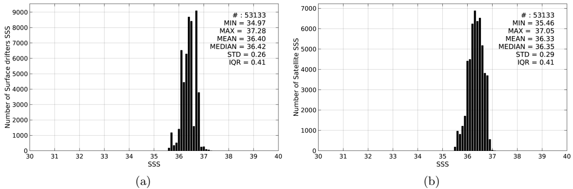
Figure 2: Histograms of SSS from Surface drifters (a) and SMOS-L3-CATDS-CECOS-LOCEAN-V2-18DAYS-25KM (b) considering all match-up pairs per bins of 0.1 over the South Atlantic Ocean Pi-MEP region and for the full satellite product period.
