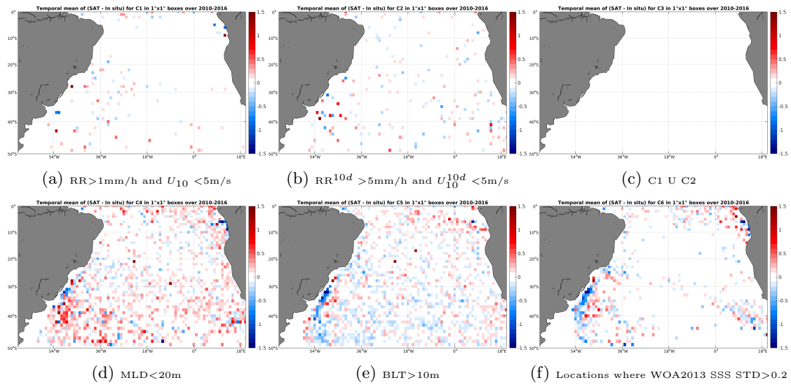
Figure 12: Temporal mean gridded over spatial boxes of size 1^\circ \times 1^\circ of \Delta SSS (SMOS-L3-CATDS-CECOS-LOCEAN-V2-18DAYS-25KM - Argo) for 6 different subdatasets corresponding to: RR > 1\text{mm/h} and U_{10} < 5\text{m/s} (a), RR^{10d} > 5\text{mm/h} and U_{10}^{10d} < 5\text{m/s} (b), C1 U C2 (c), MLD < 20\text{m} (d), BLT > 10\text{m} (e), Locations where WOA2013 SSS STD > 0.2 (f).
