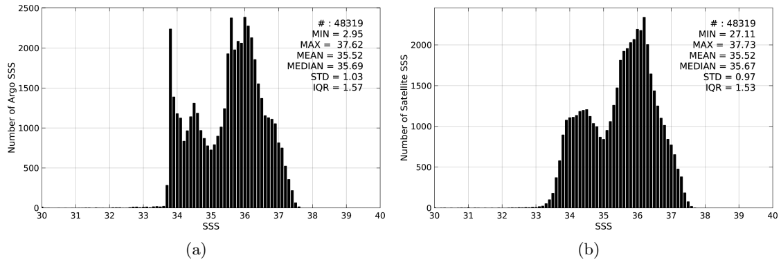
Figure 2: Histograms of SSS from Argo (a) and SMOS-L3-CATDS-CECOS-LOCEAN-V2-18DAYS-25KM (b) considering all match-up pairs per bins of 0.1 over the South Atlantic Ocean Pi-MEP region and for the full satellite product period.
