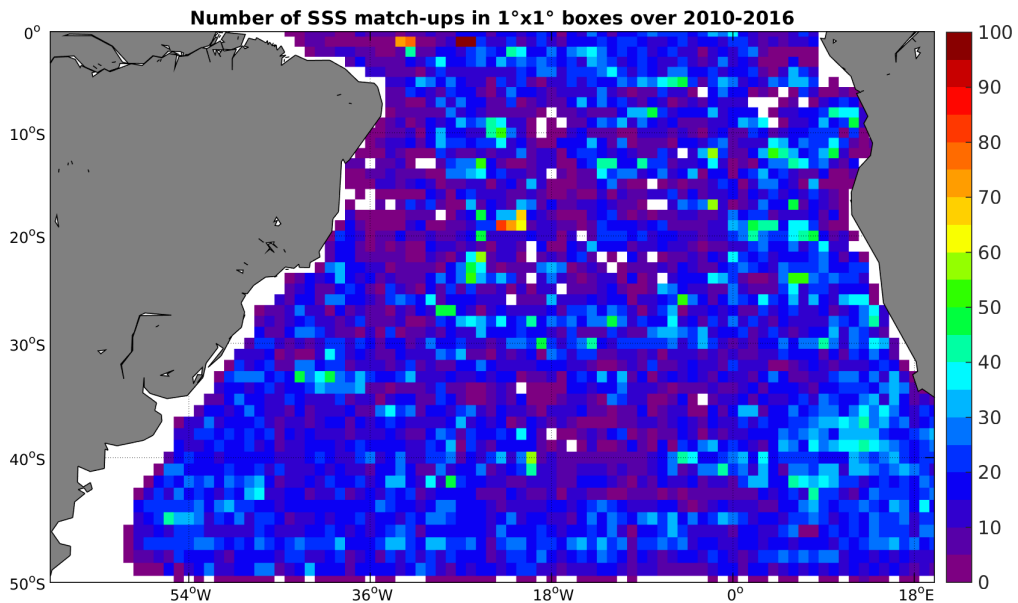
Figure 4: Number of SSS match-ups between Argo SSS and the SMOS-L3-CATDS-CECOS-LOCEAN-V2-18DAYS-25KM SSS product for the South Atlantic Ocean Pi-MEP region over 1^{\circ} \times 1^{\circ} boxes and for the full satellite product period.
