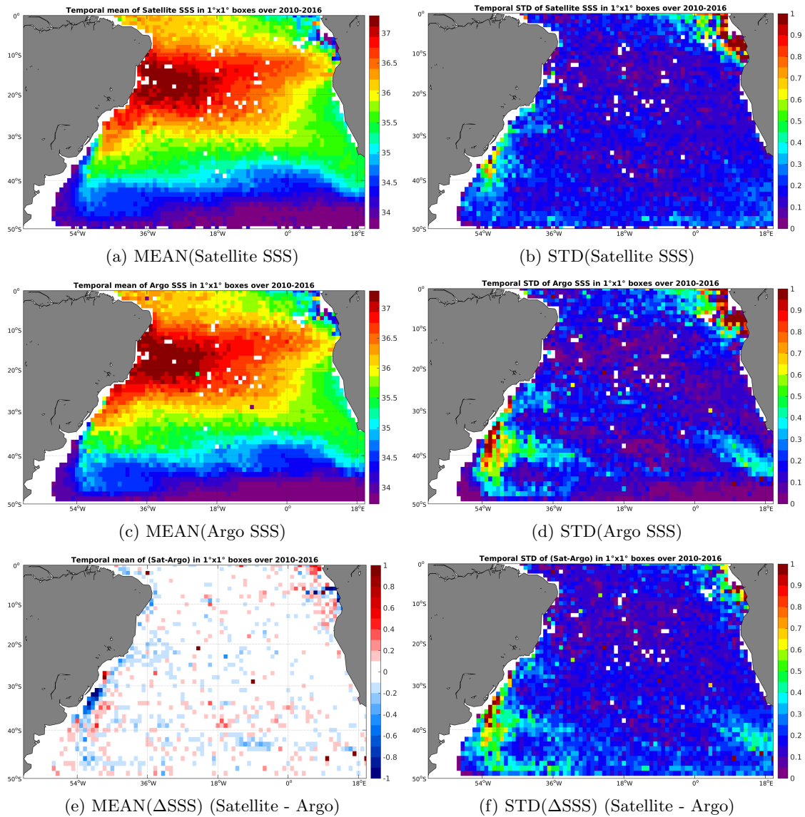
Figure 6: Temporal mean (left) and STD (right) of SSS from SMOS-L3-CATDS-CECOS-LOCEAN-V2-18DAYS-25KM (top), Argo (middle), and of \Delta SSS (Satellite - Argo). Only match-up pairs are used to generate these maps.
