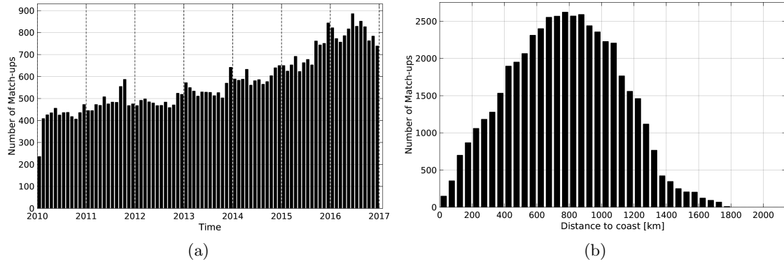
Figure 1: Number of match-ups between Argo and SMOS-L3-CATDS-CECOS-LOCEAN-V2-18DAYS-25KM SSS as a function of time (a) and as function of the distance to coast (b) over the South Atlantic Ocean Pi-MEP region and for the full satellite product period.
