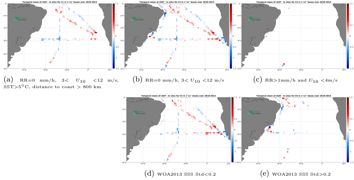
Figure 12: Temporal mean gridded over spatial boxes of size 1^\circ \times 1^\circ of \Delta SSS (SMOS SSS L3 v2 - Monthly - 0.25 Deg (CATDS-CECOS-IFREMER) - TSG (SAMOS)) for 5 different subdatasets corresponding to: RR=0 mm/h, 3 < U_{10} < 12 m/s, SST > 5^\circ C , distance to coast > 800 km (a), RR=0 mm/h, 3 < U_{10} < 12 m/s (b), RR > 1 mm/h and U_{10} < 4 m/s (c), WOA2013 SSS Std < 0.2 (d), WOA2013 SSS Std > 0.2 (e).
