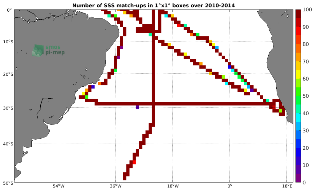
Figure 4: Number of SSS match-ups between TSG (SAMOS) SSS and the SMOS SSS L3 v2 - Monthly - 0.25 Deg (CATDS-CECOS-IFREMER) SSS product for the South Atlantic Ocean Pi-MEP region over 1^\circ \times 1^\circ boxes and for the full satellite product period.
