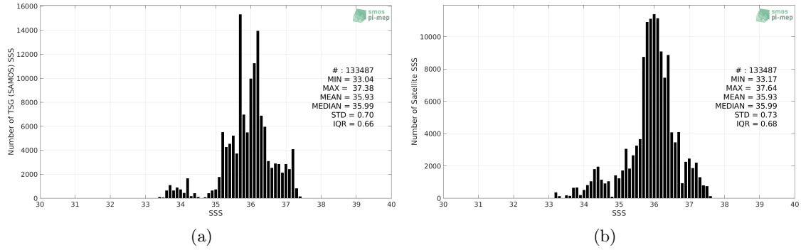
Figure 2: Histograms of SSS from TSG (SAMOS) (a) and SMOS SSS L3 v2 - Monthly - 0.25 Deg (CATDS-CECOS-IFREMER) (b) considering all match-up pairs per bins of 0.1 over the South Atlantic Ocean Pi-MEP region and for the full satellite product period.
