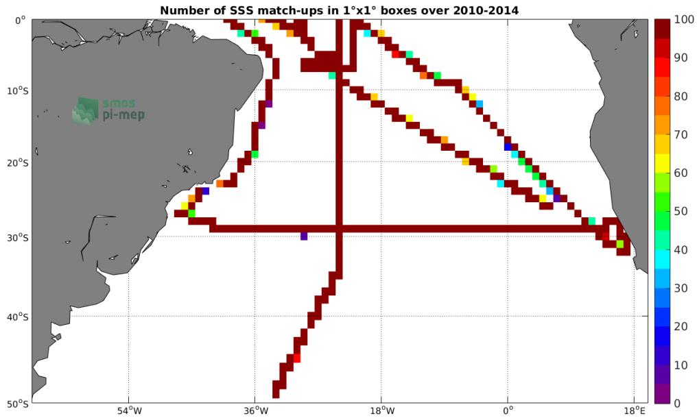
Figure 4: Number of SSS match-ups between TSG (SAMOS) SSS and the SMOS SSS L3 v2 - Monthly - 0.25 Deg (CATDS-CECOS-IFREMER) SSS product for the South Atlantic Ocean Pi-MEP region over 1°x1° boxes and for the full satellite product period.
