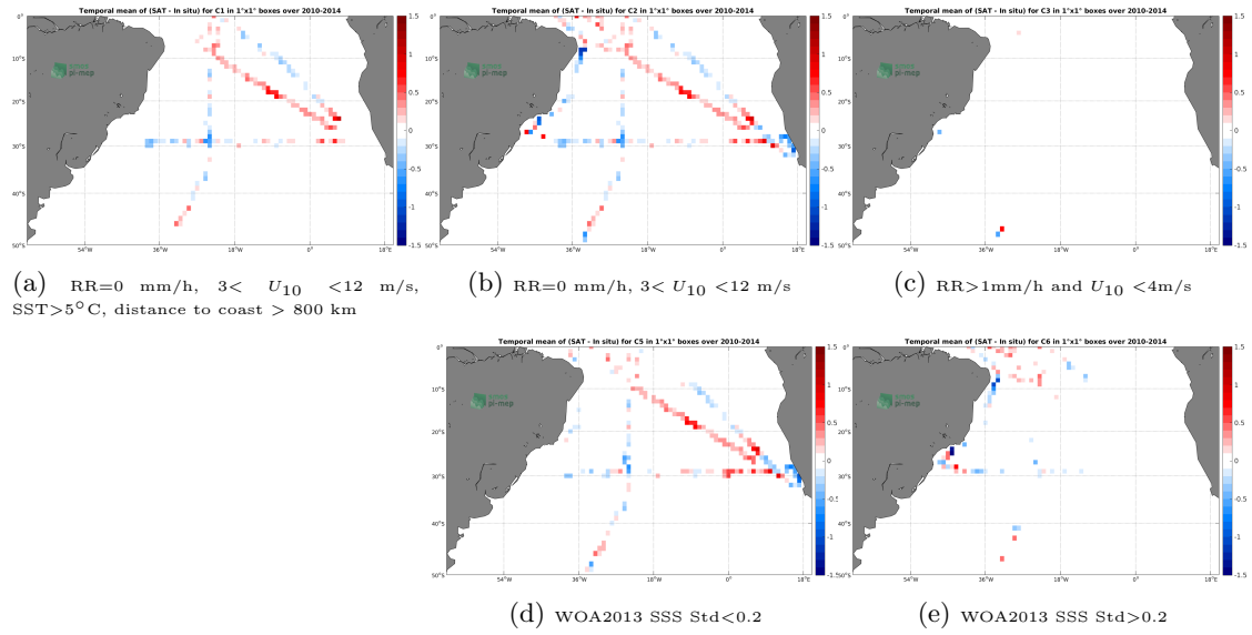
Figure 12: Temporal mean gridded over spatial boxes of size 1^\circ \times 1^\circ of \Delta SSS (SMOS SSS L3 v2 - Monthly - 0.25 Deg (CATDS-CECOS-IFREMER) - TSG (SAMOS)) for 5 different subdatasets corresponding to: RR=0 mm/h, 3 < U_{10} < 12 m/s, SST > 5^\circ C , distance to coast > 800 km (a), RR=0 mm/h, 3 < U_{10} < 12 m/s (b), RR > 1 mm/h and U_{10} < 4 m/s (c), WOA2013 SSS Std < 0.2 (d), WOA2013 SSS Std > 0.2 (e).
