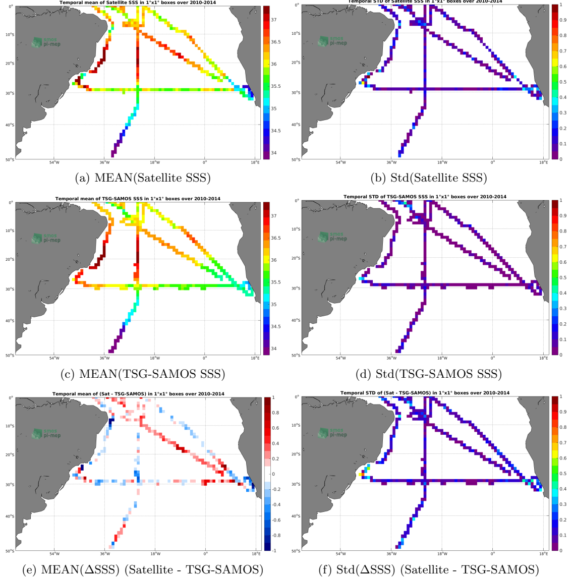
Figure 6: Temporal mean (left) and Std (right) of SSS from SMOS L3 v2 - Monthly - 0.25 Deg (CATDS-CECOS-IFREMER) (top), TSG-SAMOS (middle), and of \Delta SSS (Satellite - TSG-SAMOS). Only match-up pairs are used to generate these maps.
