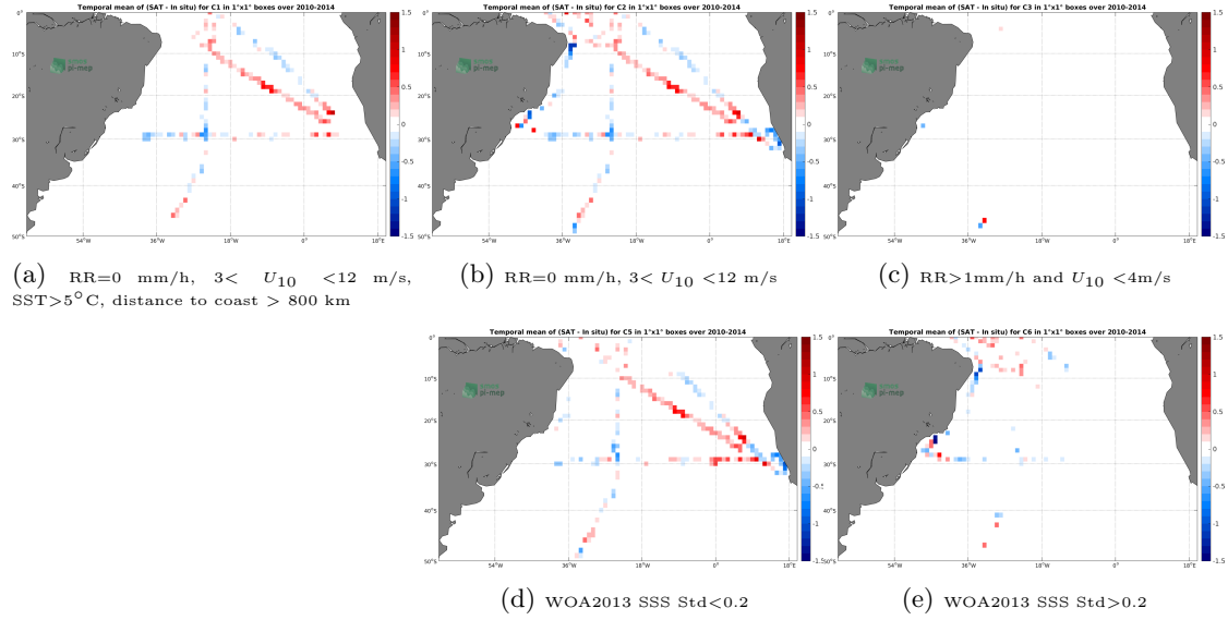
Figure 12: Temporal mean gridded over spatial boxes of size 1^\circ \times 1^\circ of \Delta SSS (SMOS L3 v2 - Monthly - 0.25 Deg (CATDS-CECOS-IFREMER) - TSG-SAMOS) for 5 different subdatasets corresponding to: RR=0 mm/h, 3 < U_{10} < 12 m/s, SST > 5^\circ C , distance to coast > 800 km (a), RR=0 mm/h, 3 < U_{10} < 12 m/s (b), RR > 1 mm/h and U_{10} < 4 m/s (c), WOA2013 SSS Std < 0.2 (d), WOA2013 SSS Std > 0.2 (e).
