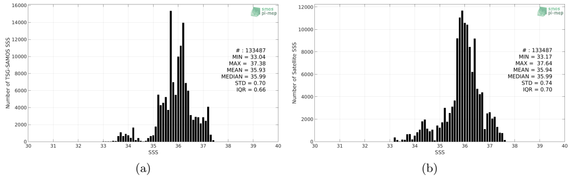
Figure 2: Histograms of SSS from TSG-SAMOS (a) and SMOS L3 v2 - Monthly - 0.25 Deg (CATDS-CECOS-IFREMER) (b) considering all match-up pairs per bins of 0.1 over the South Atlantic Ocean Pi-MEP region and for the full satellite product period.
