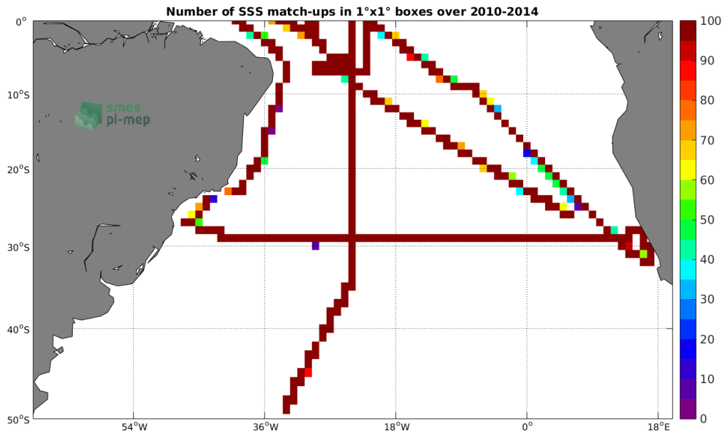
Figure 4: Number of SSS match-ups between TSG-SAMOS SSS and the SMOS L3 v2 - Monthly - 0.25 Deg (CATDS-CECOS-IFREMER) SSS product for the South Atlantic Ocean Pi-MEP region over 1°x1° boxes and for the full satellite product period.
