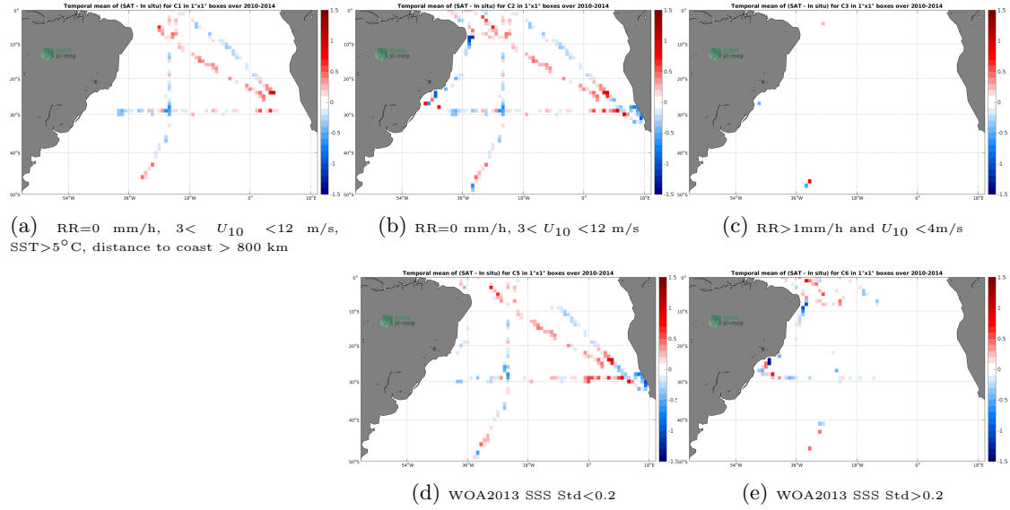
Figure 12: Temporal mean gridded over spatial boxes of size 1^\circ \times 1^\circ of \Delta SSS (SMOS-L3-CATDS-IFREMER-CECOS-V2-MONTHLY-0.25DEG - TSG-SAMOS) for 5 different subdatasets corresponding to: RR=0 mm/h, 3 < U_{10} < 12 m/s, SST > 5^\circ\text{C} , distance to coast > 800 km (a), RR=0 mm/h, 3 < U_{10} < 12 m/s (b), RR > 1 mm/h and U_{10} < 4 m/s (c), WOA2013 SSS Std < 0.2 (d), WOA2013 SSS Std > 0.2 (e).
