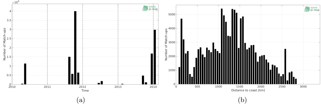
Figure 1: Number of match-ups between TSG-SAMOS and SMOS-L3-CATDS-IFREMER-CECOS-V2-MONTHLY-0.25DEG SSS as a function of time (a) and as function of the distance to coast (b) over the South Atlantic Ocean Pi-MEP region and for the full satellite product period.
