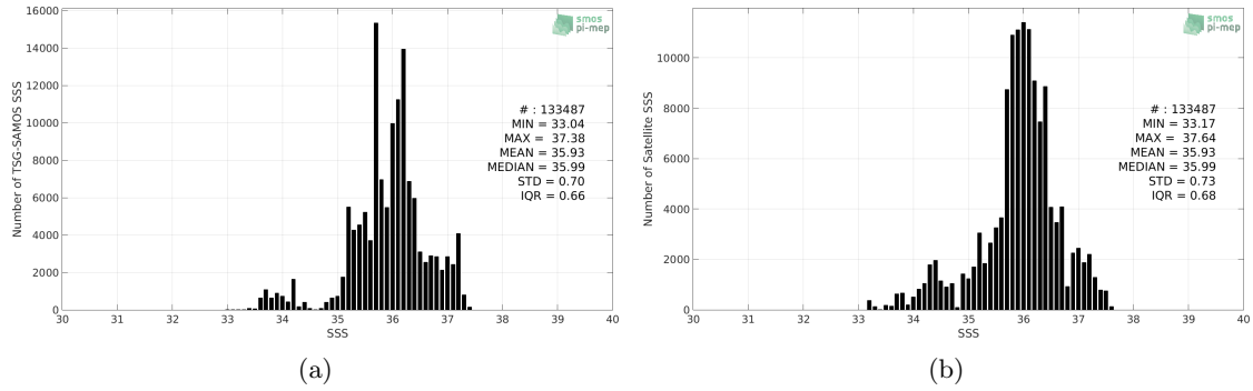
Figure 2: Histograms of SSS from TSG-SAMOS (a) and SMOS-L3-CATDS-IFREMER-CECOS-V2-MONTHLY-0.25DEG (b) considering all match-up pairs per bins of 0.1 over the South Atlantic Ocean Pi-MEP region and for the full satellite product period.
