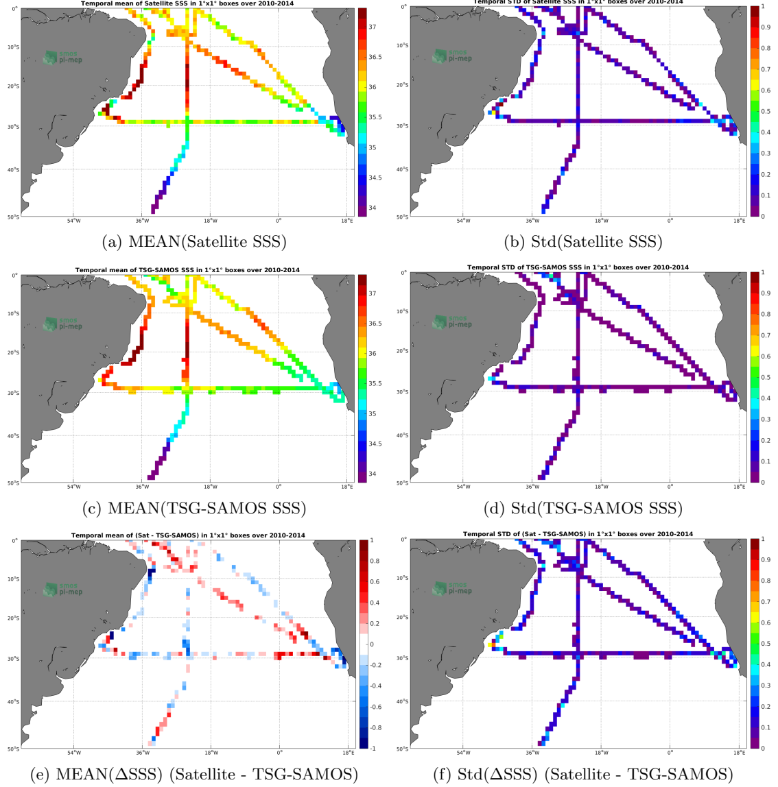
Figure 6: Temporal mean (left) and Std (right) of SSS from SMOS-L3-CATDS-IFREMER-CECOS-V2-MONTHLY-0.25DEG (top), TSG-SAMOS (middle), and of \Delta SSS (Satellite - TSG-SAMOS). Only match-up pairs are used to generate these maps.
