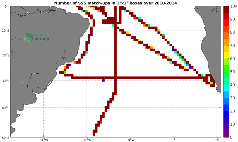
Figure 4: Number of SSS match-ups between TSG-SAMOS SSS and the SMOS-L3-CATDS-IFREMER-CECOS-V2-MONTHLY-0.25DEG SSS product for the South Atlantic Ocean Pi-MEP region over 1°x1° boxes and for the full satellite product period.
