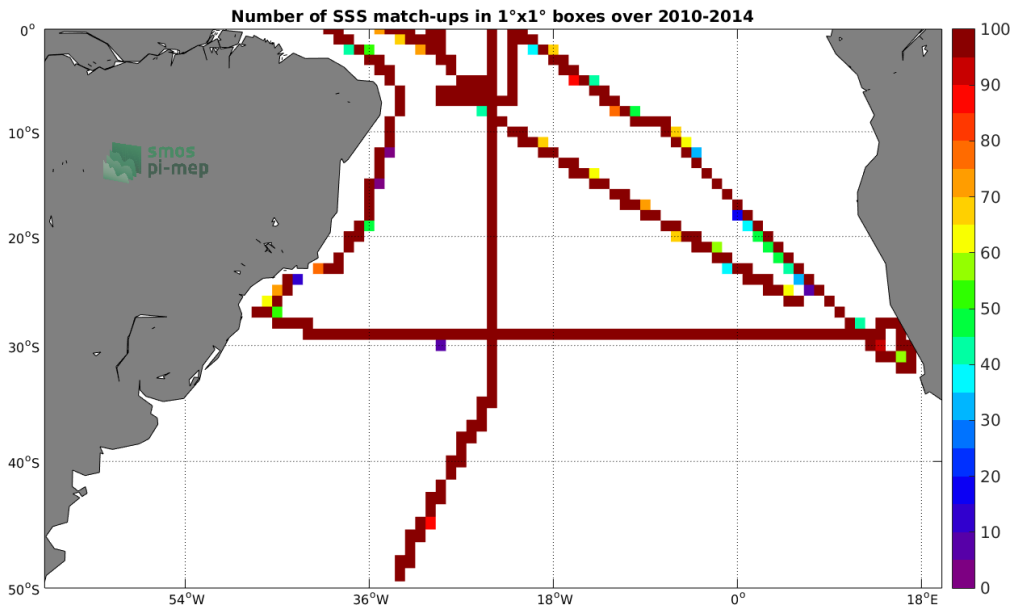
Figure 4: Number of SSS match-ups between TSG-SAMOS SSS and the SMOS-L3-CATDS-IFREMER-CECOS-V2-MONTHLY-0.25DEG SSS product for the South Atlantic Ocean Pi-MEP region over 1^\circ \times 1^\circ boxes and for the full satellite product period.
