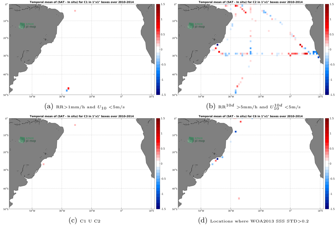
Figure 12: Temporal mean gridded over spatial boxes of size 1^\circ \times 1^\circ of \Delta SSS (SMOS-L3-CATDS-IFREMER-CECOS-V2-MONTHLY-0.25DEG - TSG-SAMOS) for 4 different subdatasets corresponding to: RR > 1mm/h and U_{10} < 5\text{m/s} (a), RR^{10d} > 5\text{mm/h} and U_{10}^{10d} < 5\text{m/s} (b), C1 U C2 (c), Locations where WOA2013 SSS STD > 0.2 (d).
