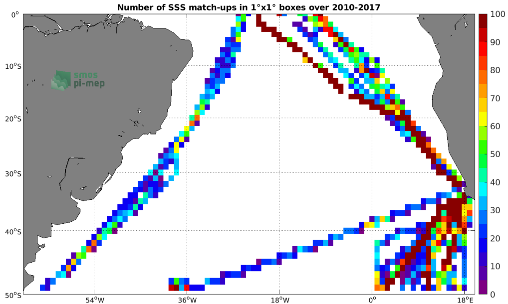
Figure 4: Number of SSS match-ups between TSG (Polarstern) SSS and the SMOS SSS L3 v2 - Monthly - 0.25 Deg (CATDS-CECOS-IFREMER) SSS product for the South Atlantic Ocean Pi-MEP region over 1^\circ \times 1^\circ boxes and for the full satellite product period.
