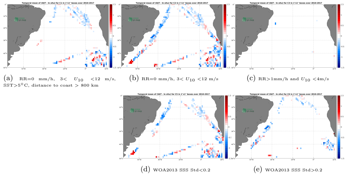
Figure 12: Temporal mean gridded over spatial boxes of size 1^\circ \times 1^\circ of \Delta SSS (SMOS SSS L3 v2 - Monthly - 0.25 Deg (CATDS-CECOS-IFREMER) - TSG (Polarstern)) for 5 different subdatasets corresponding to:RR=0 mm/h, 3 < U_{10} < 12 m/s, SST >5^\circ\text{C} , distance to coast > 800 km (a), RR=0 mm/h, 3 < U_{10} < 12 m/s (b), RR >1 mm/h and U_{10} < 4 m/s (c), WOA2013 SSS Std <0.2 (d), WOA2013 SSS Std >0.2 (e).
