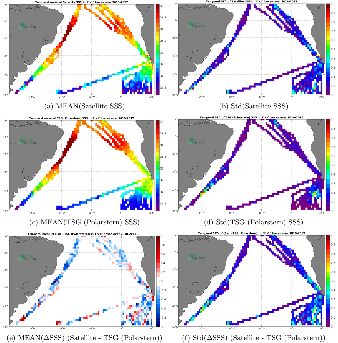
Figure 6: Temporal mean (left) and Std (right) of SSS from SMOS SSS L3 v2 - Monthly - 0.25 Deg (CATDS-CECOS-IFREMER) (top), TSG (Polarstern) (middle), and of \Delta SSS (Satellite - TSG (Polarstern)). Only match-up pairs are used to generate these maps.
