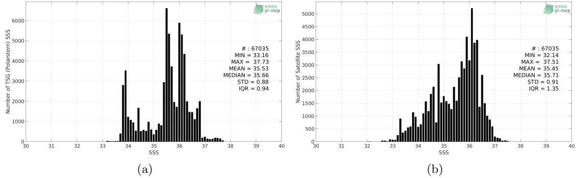
Figure 2: Histograms of SSS from TSG (Polarstern) (a) and SMOS SSS L3 v2 - Monthly - 0.25 Deg (CATDS-CECOS-IFREMER) (b) considering all match-up pairs per bins of 0.1 over the South Atlantic Ocean Pi-MEP region and for the full satellite product period.
