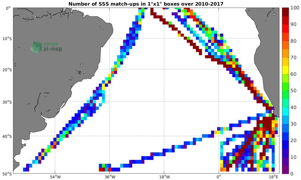
Figure 4: Number of SSS match-ups between TSG (Polarstern) SSS and the SMOS SSS L3 v2 - Monthly - 0.25 Deg (CATDS-CECOS-IFREMER) SSS product for the South Atlantic Ocean Pi-MEP region over 1°x1° boxes and for the full satellite product period.
