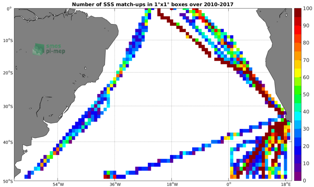
Figure 4: Number of SSS match-ups between TSG-POLARSTERN SSS and the SMOS-L3-CATDS-IFREMER-CECOS-V2-MONTHLY-0.25DEG SSS product for the South Atlantic Ocean Pi-MEP region over 1°x1° boxes and for the full satellite product period.
