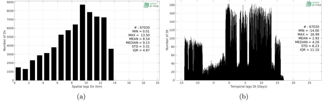
Figure 5: Histograms of the spatial (a) and temporal (b) lags between the time of the TSG-POLARSTERN measurements and the date of the corresponding SMOS-L3-CATDS-IFREMER-CECOS-V2-MONTHLY-0.25DEG SSS product.
