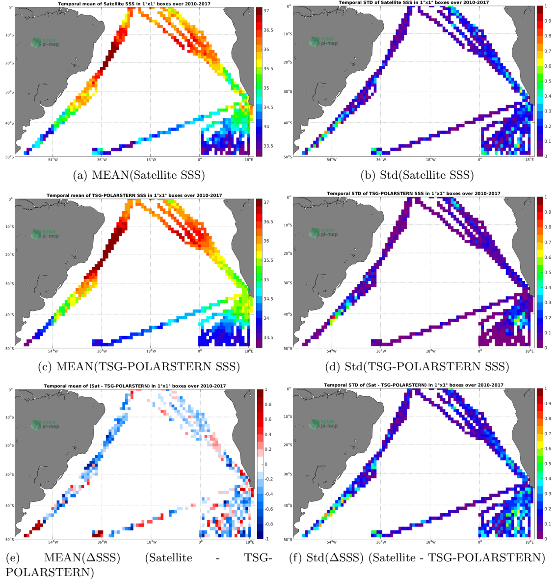
Figure 6: Temporal mean (left) and Std (right) of SSS from SMOS-L3-CATDS-IFREMER-CECOS-V2-MONTHLY-0.25DEG (top), TSG-POLARSTERN (middle), and of \Delta SSS (Satellite - TSG-POLARSTERN). Only match-up pairs are used to generate these maps.
