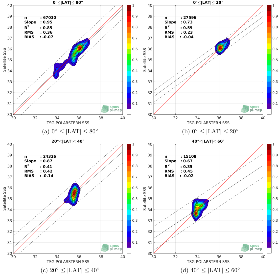
Figure 9: Contour maps of the concentration of SMOS-L3-CATDS-IFREMER-CECOS-V2-MONTHLY-0.25DEG SSS (y-axis) versus TSG-POLARSTERN SSS (x-axis) at match-up pairs for different latitude bands. For each plot, the red line shows x=y . The black thin and dashed lines indicate a linear fit through the data cloud and the \pm 95\% confidence levels, respectively. The number match-up pairs n , the slope and R^2 coefficient of the linear fit, the root mean square (RMS) and the mean bias between satellite and in situ data are indicated for each latitude band in each plots.
