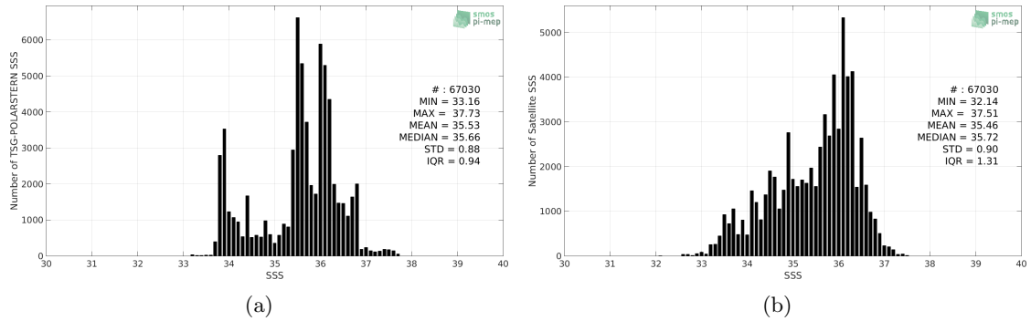
Figure 2: Histograms of SSS from TSG-POLARSTERN (a) and SMOS-L3-CATDS-IFREMER-CECOS-V2-MONTHLY-0.25DEG (b) considering all match-up pairs per bins of 0.1 over the South Atlantic Ocean Pi-MEP region and for the full satellite product period.
