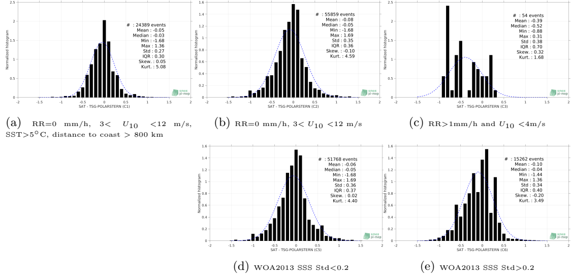
Figure 13: Normalized histogram of \Delta SSS (SMOS-L3-CATDS-IFREMER-CECOS-V2-MONTHLY-0.25DEG - TSG-POLARSTERN) for 5 different subdatasets corresponding to: RR=0 mm/h, 3 < U_{10} < 12 m/s, SST>5°C, distance to coast > 800 km (a), RR=0 mm/h, 3 < U_{10} < 12 m/s (b), RR>1mm/h and U_{10} < 4 m/s (c), WOA2013 SSS Std<0.2 (d), WOA2013 SSS Std>0.2 (e).
