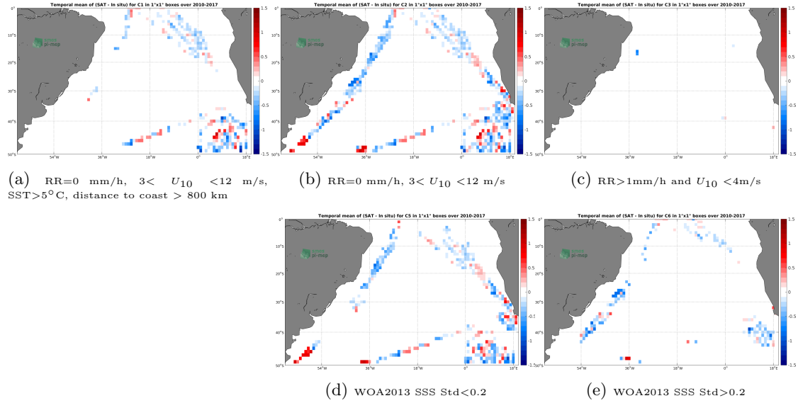
Figure 12: Temporal mean gridded over spatial boxes of size 1^\circ \times 1^\circ of \Delta SSS (SMOS-L3-CATDS-IFREMER-CECOS-V2-MONTHLY-0.25DEG - TSG-POLARSTERN) for 5 different subdatasets corresponding to: RR=0 mm/h, 3 < U_{10} < 12 m/s, SST > 5^\circ C , distance to coast > 800 km (a), RR=0 mm/h, 3 < U_{10} < 12 m/s (b), RR > 1 mm/h and U_{10} < 4 m/s (c), WOA2013 SSS Std < 0.2 (d), WOA2013 SSS Std > 0.2 (e).
