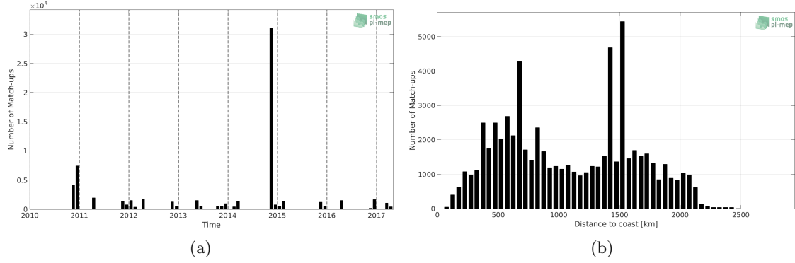
Figure 1: Number of match-ups between TSG-POLARSTERN and SMOS-L3-CATDS-IFREMER-CECOS-V2-MONTHLY-0.25DEG SSS as a function of time (a) and as function of the distance to coast (b) over the South Atlantic Ocean Pi-MEP region and for the full satellite product period.
