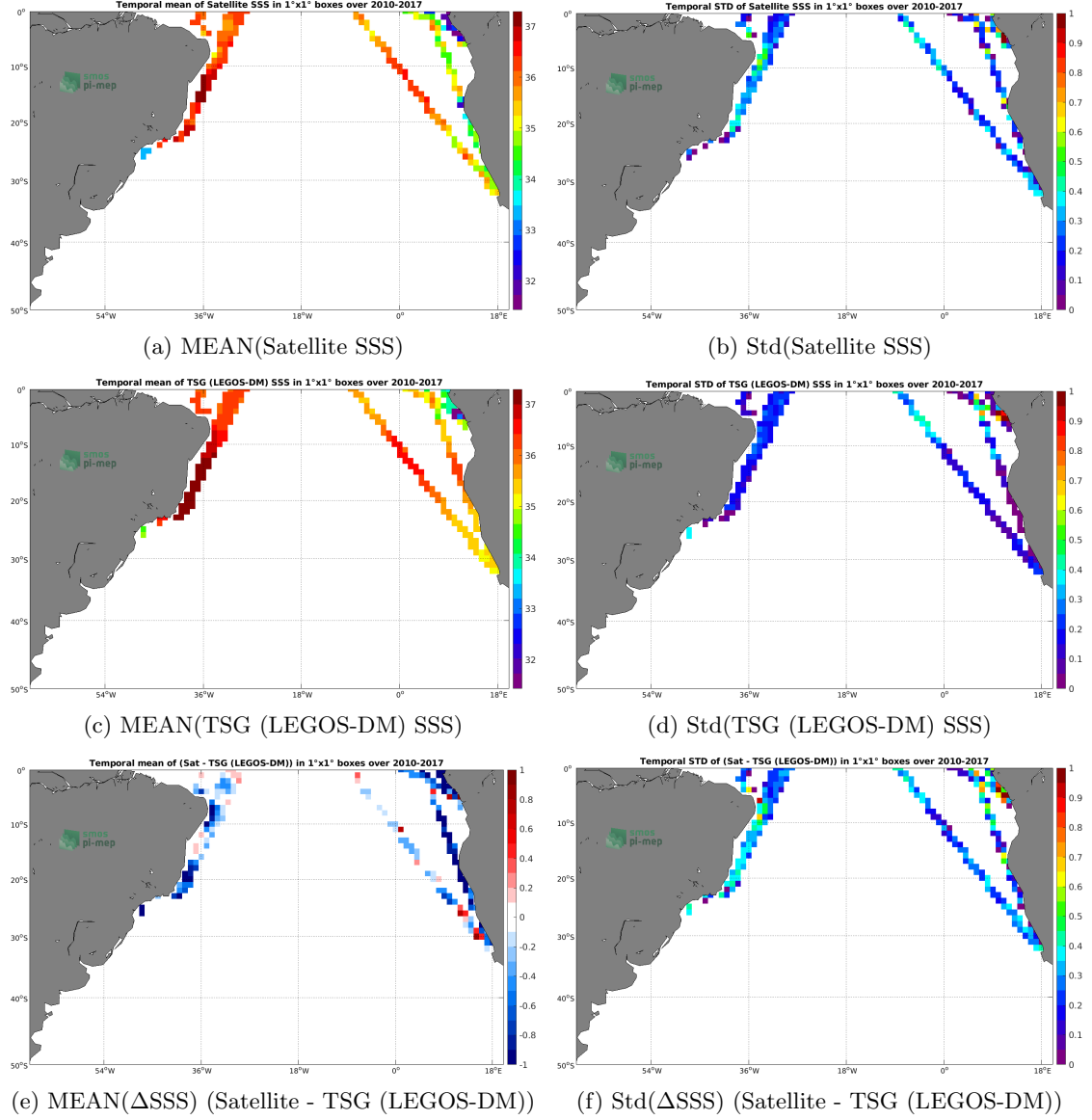
Figure 6: Temporal mean (left) and Std (right) of SSS from SMOS SSS L3 v2 - Monthly - 0.25 Deg (CATDS-CECOS-IFREMER) (top), TSG (LEGOS-DM) (middle), and of \Delta SSS (Satellite - TSG (LEGOS-DM)). Only match-up pairs are used to generate these maps.
