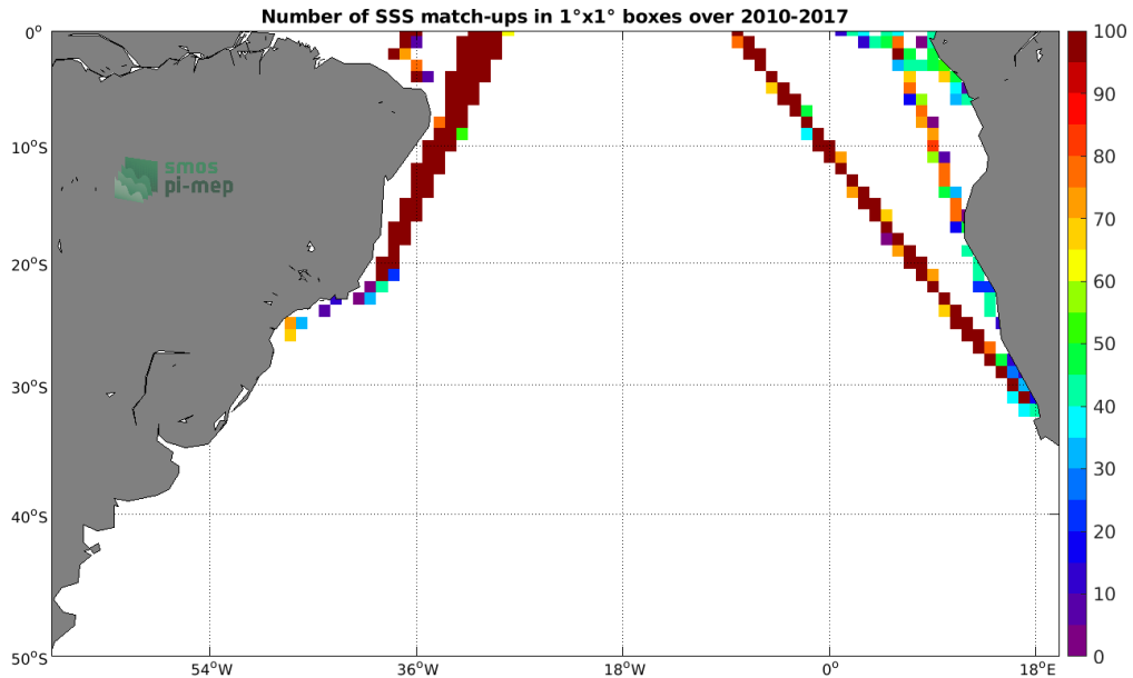
Figure 4: Number of SSS match-ups between TSG (LEGOS-DM) SSS and the SMOS SSS L3 v2 - Monthly - 0.25 Deg (CATDS-CECOS-IFREMER) SSS product for the South Atlantic Ocean Pi-MEP region over 1^\circ \times 1^\circ boxes and for the full satellite product period.
