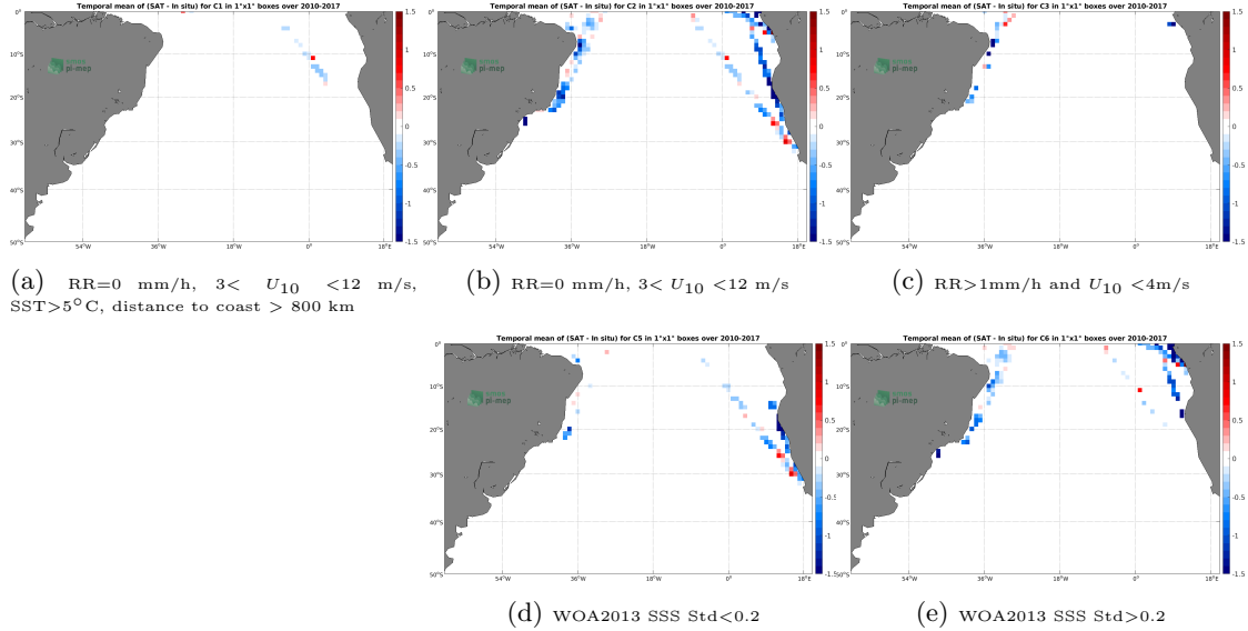
Figure 12: Temporal mean gridded over spatial boxes of size 1^{\circ}\times 1^{\circ} of \Delta\text{SSS} (SMOS SSS L3 v2 - Monthly - 0.25 Deg (CATDS-CECOS-IFREMER) - TSG (LEGOS-DM)) for 5 different subdatasets corresponding to: RR=0 mm/h, 3 < U_{10} < 12 m/s, SST > 5^{\circ}\text{C} , distance to coast > 800 km (a), RR=0 mm/h, 3 < U_{10} < 12 m/s (b), RR > 1 mm/h and U_{10} < 4 m/s (c), WOA2013 SSS Std < 0.2 (d), WOA2013 SSS Std > 0.2 (e).
