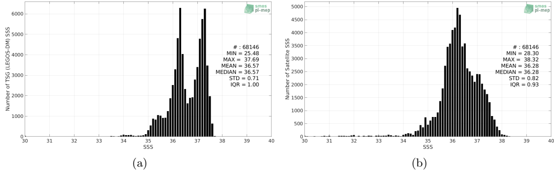
Figure 2: Histograms of SSS from TSG (LEGOS-DM) (a) and SMOS SSS L3 v2 - Monthly - 0.25 Deg (CATDS-CECOS-IFREMER) (b) considering all match-up pairs per bins of 0.1 over the South Atlantic Ocean Pi-MEP region and for the full satellite product period.
