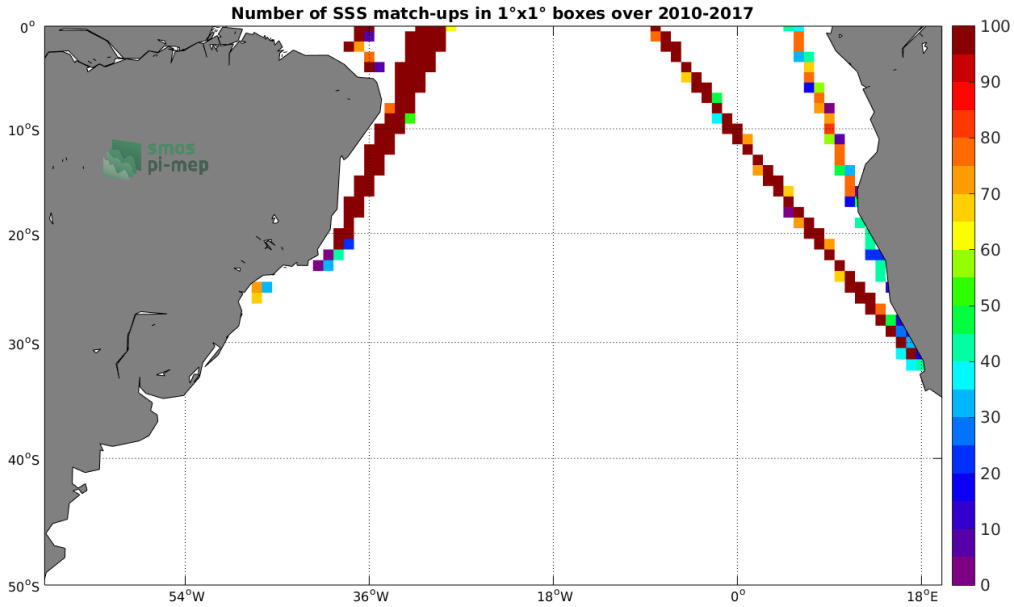
Figure 4: Number of SSS match-ups between TSG-LEGOS-DM SSS and the SMOS L3 v2 - Monthly - 0.25 Deg (CATDS-CECOS-IFREMER) SSS product for the South Atlantic Ocean Pi-MEP region over 1^\circ \times 1^\circ boxes and for the full satellite product period.
