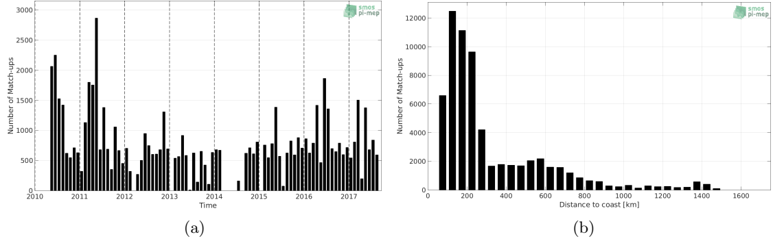
Figure 1: Number of match-ups between TSG-LEGOS-DM and SMOS L3 v2 - Monthly - 0.25 Deg (CATDS-CECOS-IFREMER) SSS as a function of time (a) and as function of the distance to coast (b) over the South Atlantic Ocean Pi-MEP region and for the full satellite product period.
