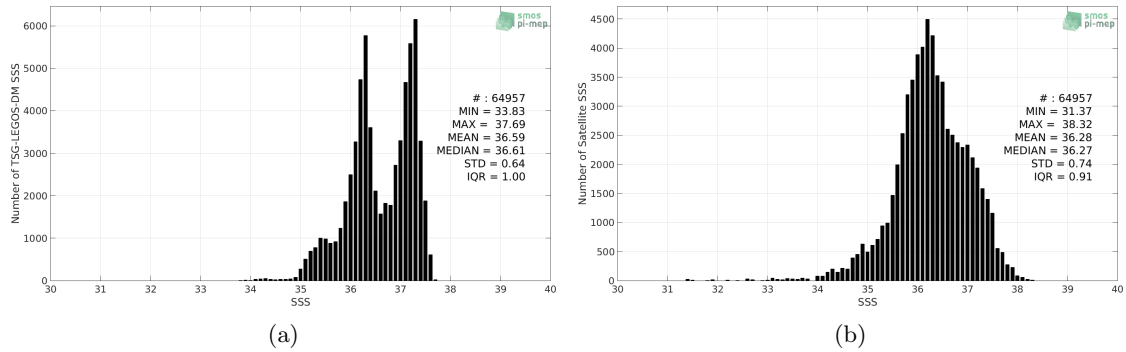
Figure 2: Histograms of SSS from TSG-LEGOS-DM (a) and SMOS L3 v2 - Monthly - 0.25 Deg (CATDS-CECOS-IFREMER) (b) considering all match-up pairs per bins of 0.1 over the South Atlantic Ocean Pi-MEP region and for the full satellite product period.
