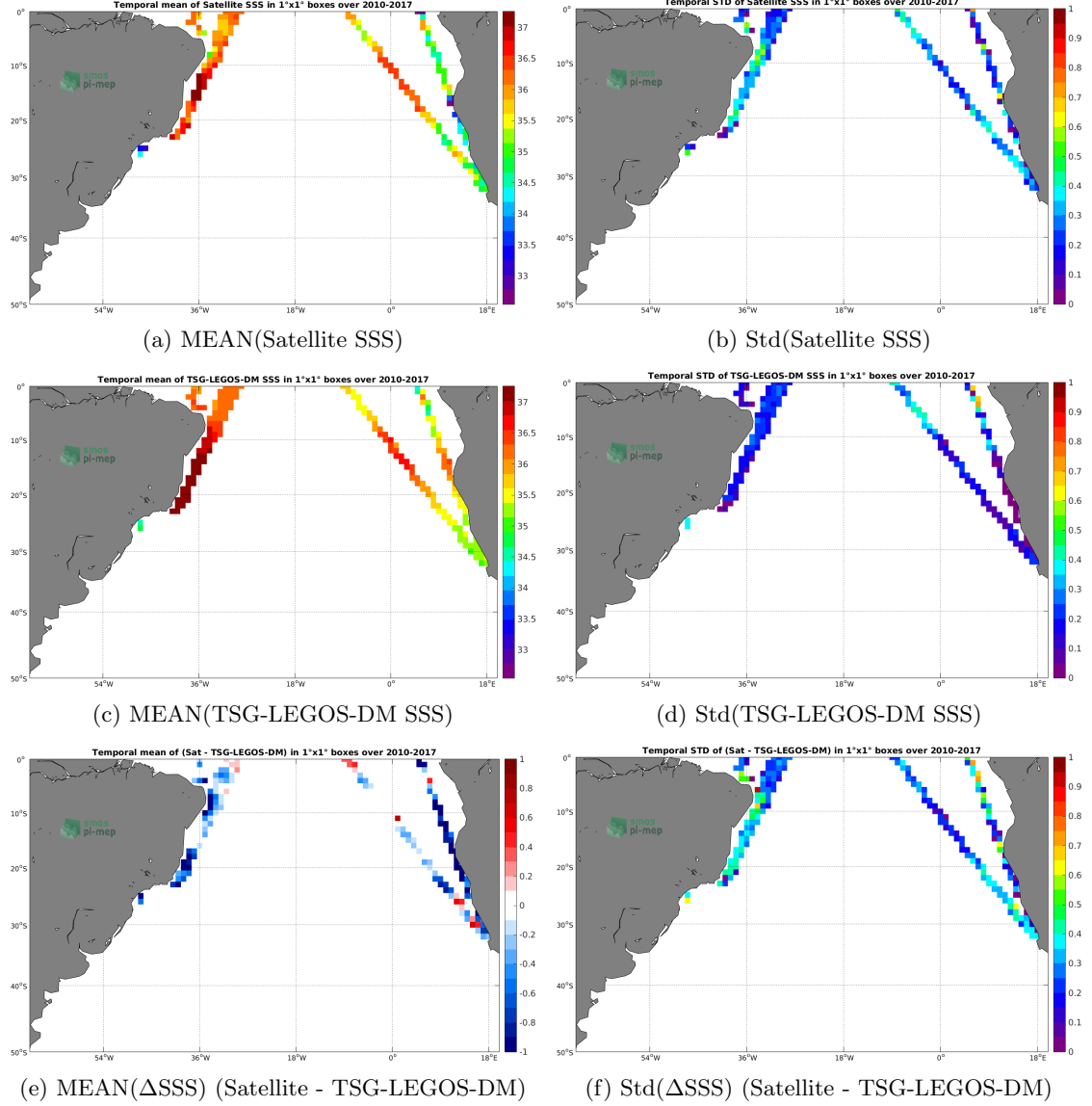
Figure 6: Temporal mean (left) and Std (right) of SSS from SMOS L3 v2 - Monthly - 0.25 Deg (CATDS-CECOS-IFREMER) (top), TSG-LEGOS-DM (middle), and of \Delta SSS (Satellite - TSG-LEGOS-DM). Only match-up pairs are used to generate these maps.
