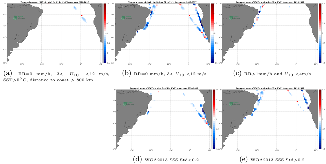
Figure 12: Temporal mean gridded over spatial boxes of size 1^{\circ}\times 1^{\circ} of \Delta\text{SSS} (SMOS L3 v2 - Monthly - 0.25 Deg (CATDS-CECOS-IFREMER) - TSG-LEGOS-DM) for 5 different subdatasets corresponding to: \text{RR}=0 mm/h, 3 < U_{10} < 12 m/s, \text{SST} > 5^{\circ}\text{C} , distance to coast > 800 km (a), \text{RR}=0 mm/h, 3 < U_{10} < 12 m/s (b), \text{RR} > 1 mm/h and U_{10} < 4 m/s (c), WOA2013 SSS Std < 0.2 (d), WOA2013 SSS Std > 0.2 (e).
