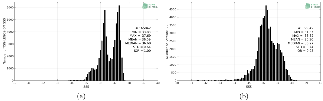
Figure 2: Histograms of SSS from TSG-LEGOS-DM (a) and SMOS-L3-CATDS-IFREMER-CECOS-V2-MONTHLY-0.25DEG (b) considering all match-up pairs per bins of 0.1 over the South Atlantic Ocean Pi-MEP region and for the full satellite product period.
