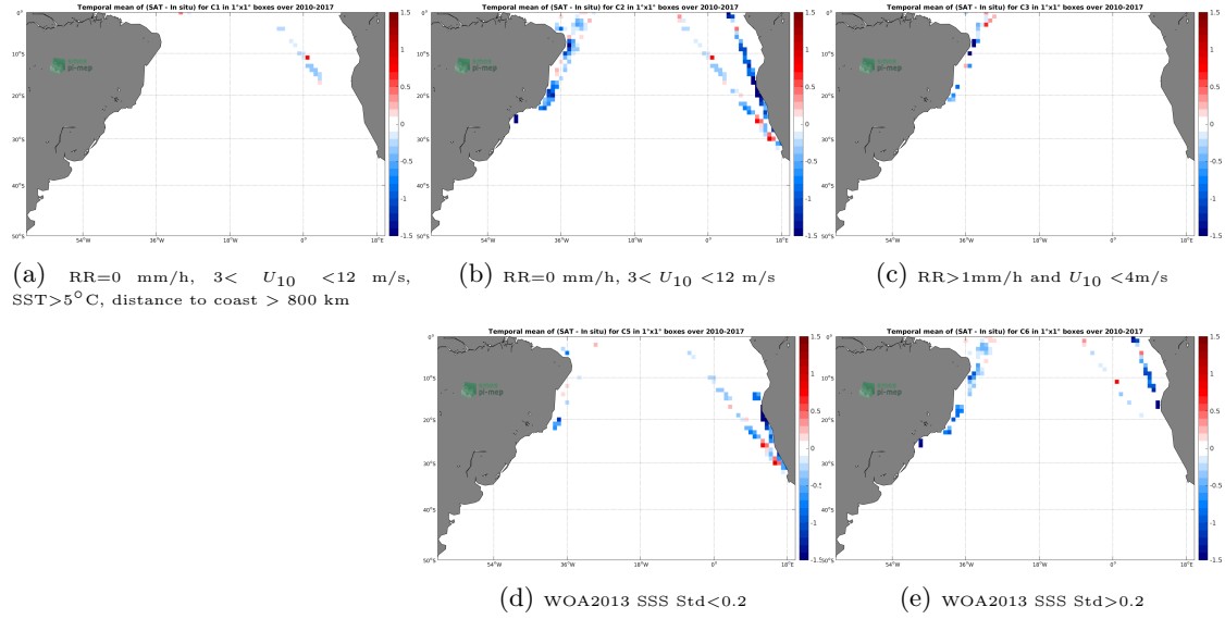
Figure 12: Temporal mean gridded over spatial boxes of size 1^\circ \times 1^\circ of \Delta SSS (SMOS-L3-CATDS-IFREMER-CECOS-V2-MONTHLY-0.25DEG - TSG-LEGOS-DM) for 5 different subdatasets corresponding to: RR=0 mm/h, 3 < U_{10} < 12 m/s, SST > 5^\circ\text{C} , distance to coast > 800 km (a), RR=0 mm/h, 3 < U_{10} < 12 m/s (b), RR > 1 mm/h and U_{10} < 4 m/s (c), WOA2013 SSS Std < 0.2 (d), WOA2013 SSS Std > 0.2 (e).
