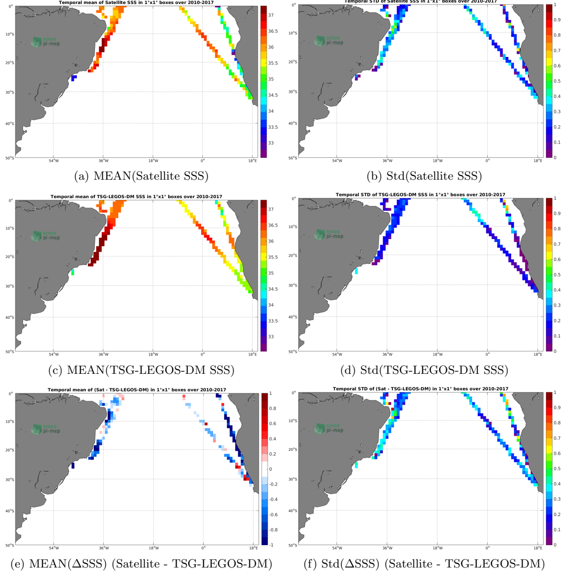
Figure 6: Temporal mean (left) and Std (right) of SSS from SMOS-L3-CATDS-IFREMER-CECOS-V2-MONTHLY-0.25DEG (top), TSG-LEGOS-DM (middle), and of \Delta SSS (Satellite - TSG-LEGOS-DM). Only match-up pairs are used to generate these maps.
