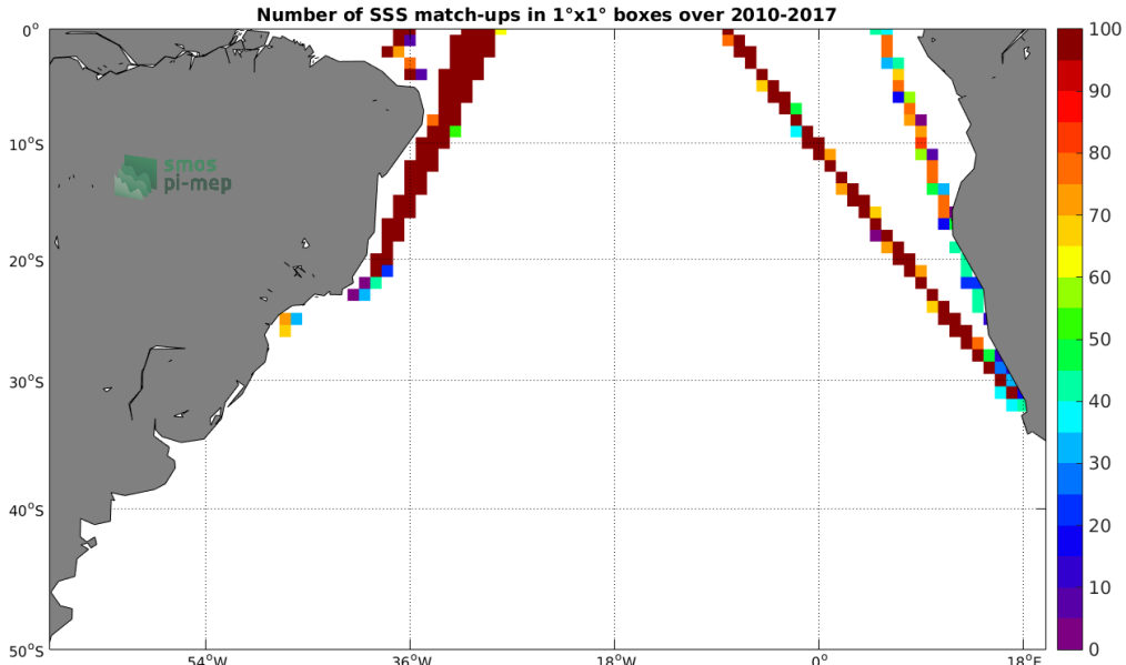
Figure 4: Number of SSS match-ups between TSG-LEGOS-DM SSS and the SMOS-L3-CATDS-IFREMER-CECOS-V2-MONTHLY-0.25DEG SSS product for the South Atlantic Ocean Pi-MEP region over 1^\circ \times 1^\circ boxes and for the full satellite product period.
