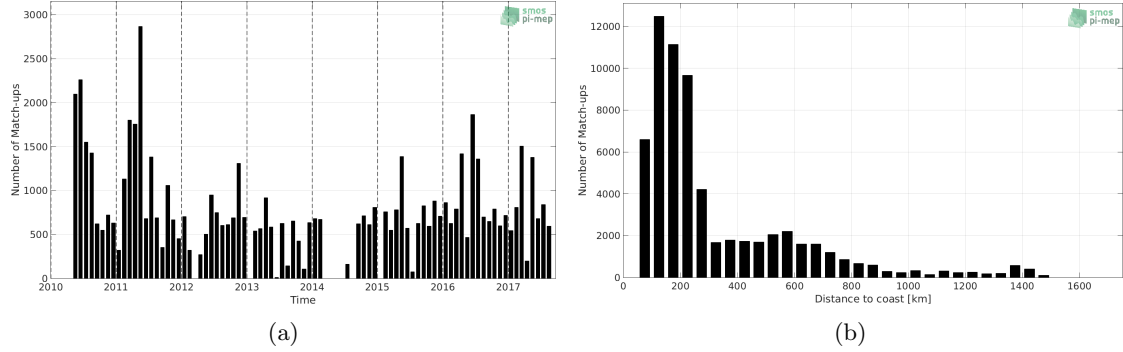
Figure 1: Number of match-ups between TSG-LEGOS-DM and SMOS-L3-CATDS-IFREMER-CECOS-V2-MONTHLY-0.25DEG SSS as a function of time (a) and as function of the distance to coast (b) over the South Atlantic Ocean Pi-MEP region and for the full satellite product period.
