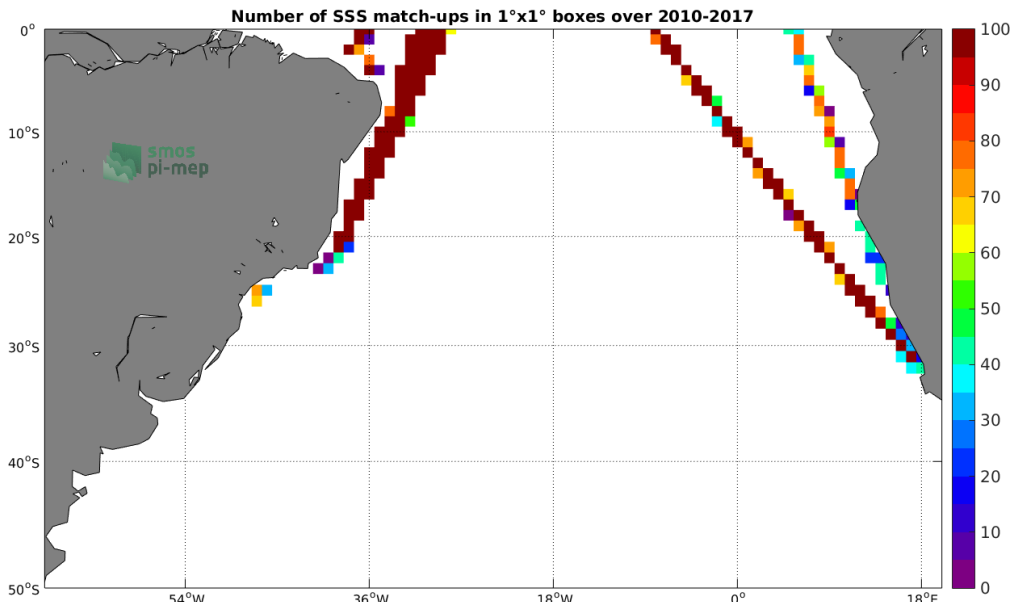
Figure 4: Number of SSS match-ups between TSG-LEGOS-DM SSS and the SMOS-L3-CATDS-IFREMER-CECOS-V2-MONTHLY-0.25DEG SSS product for the South Atlantic Ocean Pi-MEP region over 1^\circ \times 1^\circ boxes and for the full satellite product period.
