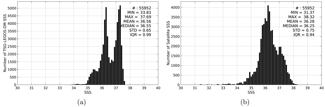
Figure 2: Histograms of SSS from TSG-LEGOS-DM (a) and SMOS-L3-CATDS-IFREMER-CECOS-V2-MONTHLY-0.25DEG (b) considering all match-up pairs per bins of 0.1 over the South Atlantic Ocean Pi-MEP region and for the full satellite product period.
