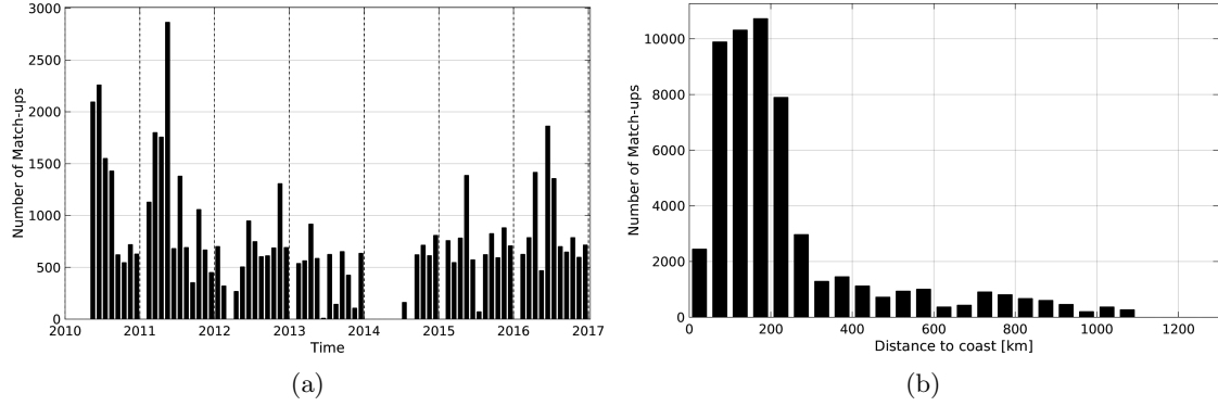
Figure 1: Number of match-ups between TSG-LEGOS-DM and SMOS-L3-CATDS-IFREMER-CECOS-V2-MONTHLY-0.25DEG SSS as a function of time (a) and as function of the distance to coast (b) over the South Atlantic Ocean Pi-MEP region and for the full satellite product period.
