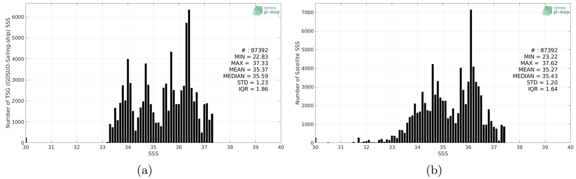
Figure 2: Histograms of SSS from TSG (GOSUD-Sailing-ship) (a) and SMOS SSS L3 v2 - Monthly - 0.25 Deg (CATDS-CECOS-IFREMER) (b) considering all match-up pairs per bins of 0.1 over the South Atlantic Ocean Pi-MEP region and for the full satellite product period.
