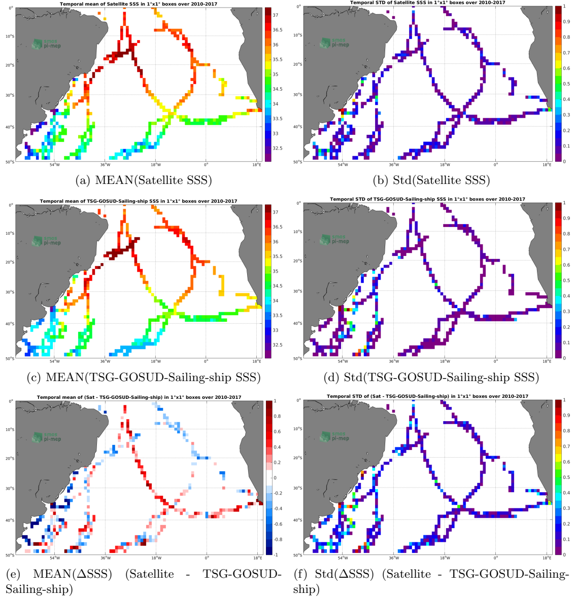
Figure 6: Temporal mean (left) and Std (right) of SSS from SMOS-L3-CATDS-IFREMER-CECOS-V2-MONTHLY-0.25DEG (top), TSG-GOSUD-Sailing-ship (middle), and of \Delta SSS (Satellite - TSG-GOSUD-Sailing-ship). Only match-up pairs are used to generate these maps.
