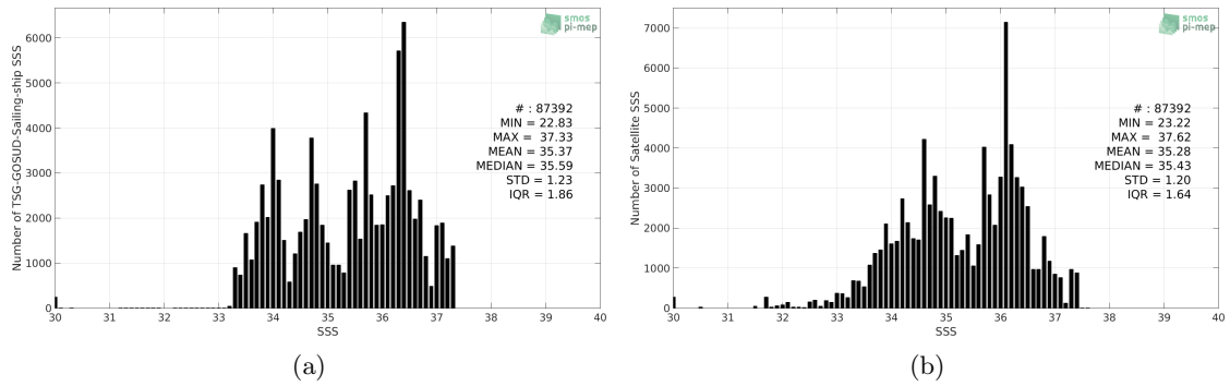
Figure 2: Histograms of SSS from TSG-GOSUD-Sailing-ship (a) and SMOS-L3-CATDS-IFREMER-CECOS-V2-MONTHLY-0.25DEG (b) considering all match-up pairs per bins of 0.1 over the South Atlantic Ocean Pi-MEP region and for the full satellite product period.
