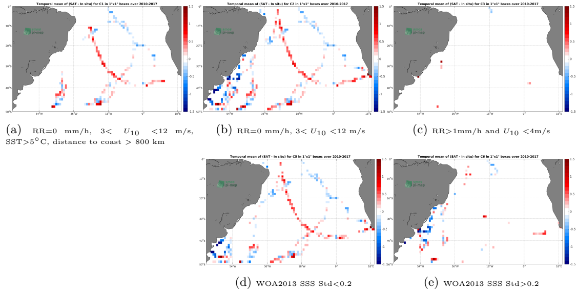
Figure 12: Temporal mean gridded over spatial boxes of size 1^\circ \times 1^\circ of \Delta SSS (SMOS-L3-CATDS-IFREMER-CECOS-V2-MONTHLY-0.25DEG - TSG-GOSUD-Sailing-ship) for 5 different sub-datasets corresponding to: RR=0 mm/h, 3 < U_{10} < 12 m/s, SST > 5^\circ C , distance to coast > 800 km (a), RR=0 mm/h, 3 < U_{10} < 12 m/s (b), RR > 1 mm/h and U_{10} < 4 m/s (c), WOA2013 SSS Std < 0.2 (d), WOA2013 SSS Std > 0.2 (e).
