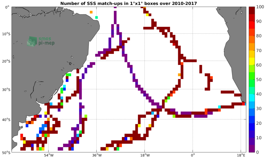
Figure 4: Number of SSS match-ups between TSG-GOSUD-Sailing-ship SSS and the SMOS-L3-CATDS-IFREMER-CECOS-V2-MONTHLY-0.25DEG SSS product for the South Atlantic Ocean Pi-MEP region over 1^\circ \times 1^\circ boxes and for the full satellite product period.
