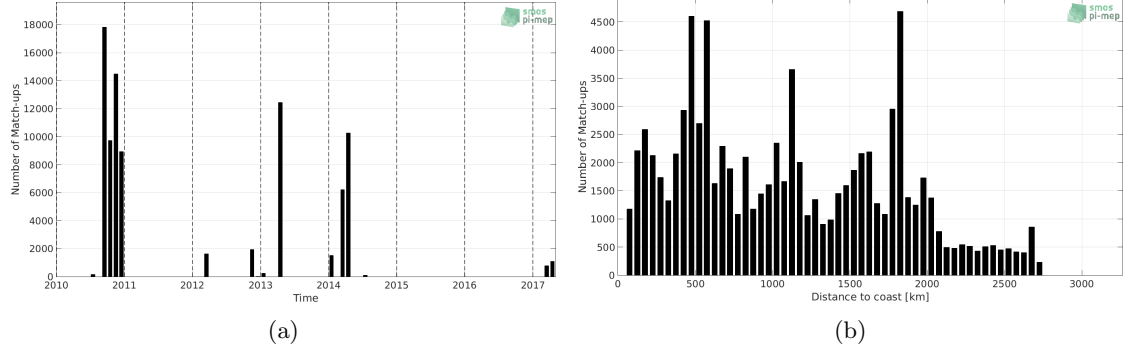
Figure 1: Number of match-ups between TSG-GOSUD-Sailing-ship and SMOS-L3-CATDS-IFREMER-CECOS-V2-MONTHLY-0.25DEG SSS as a function of time (a) and as function of the distance to coast (b) over the South Atlantic Ocean Pi-MEP region and for the full satellite product period.
