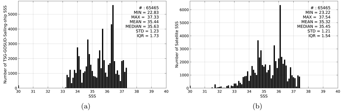
Figure 2: Histograms of SSS from TSG-GOSUD-Sailing-ship (a) and SMOS-L3-CATDS-IFREMER-CECOS-V2-MONTHLY-0.25DEG (b) considering all match-up pairs per bins of 0.1 over the South Atlantic Ocean Pi-MEP region and for the full satellite product period.
