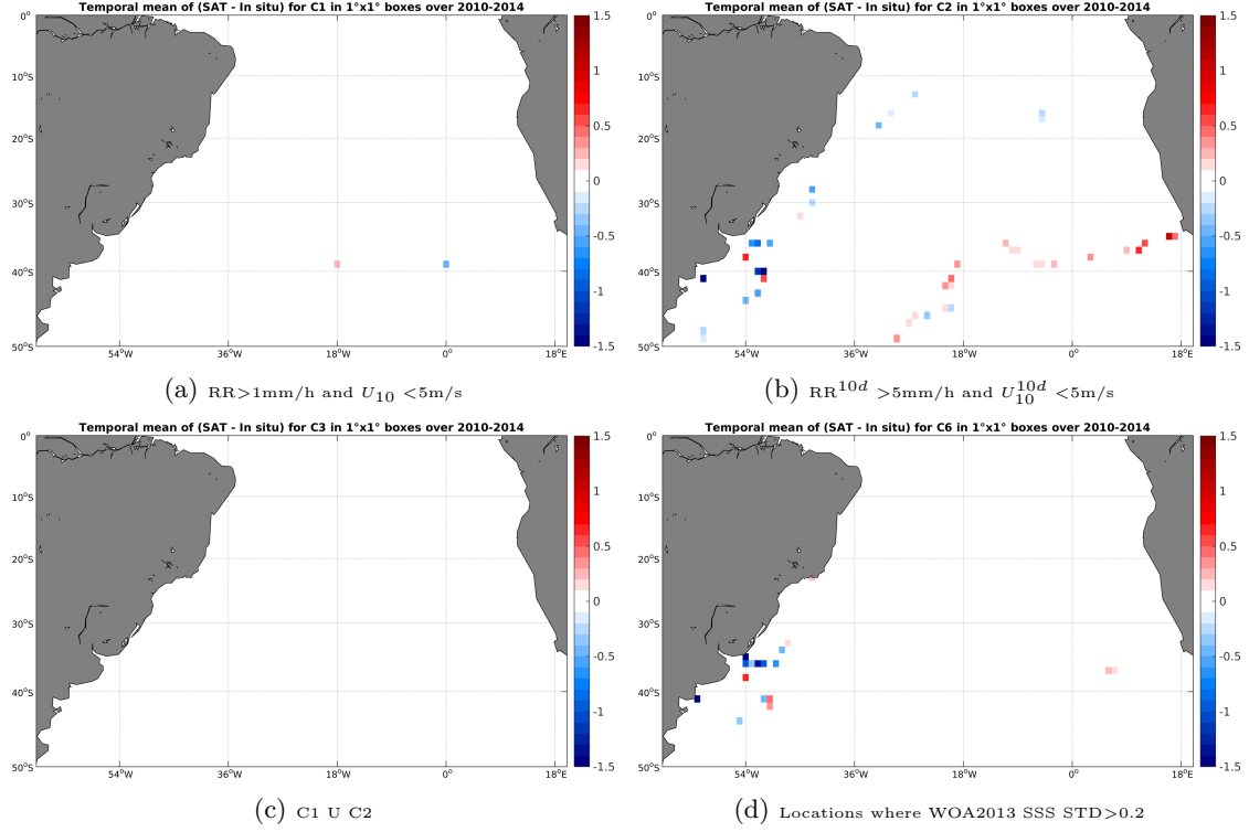
Figure 12: Temporal mean gridded over spatial boxes of size 1^\circ \times 1^\circ of \Delta SSS (SMOS-L3-CATDS-IFREMER-CECOS-V2-MONTHLY-0.25DEG - TSG-GOSUD-Sailing-ship) for 4 different sub-datasets corresponding to: RR > 1\text{mm/h} and U_{10} < 5\text{m/s} (a), RR^{10d} > 5\text{mm/h} and U_{10}^{10d} < 5\text{m/s} (b), C1 U C2 (c), Locations where WOA2013 SSS STD > 0.2 (d).
