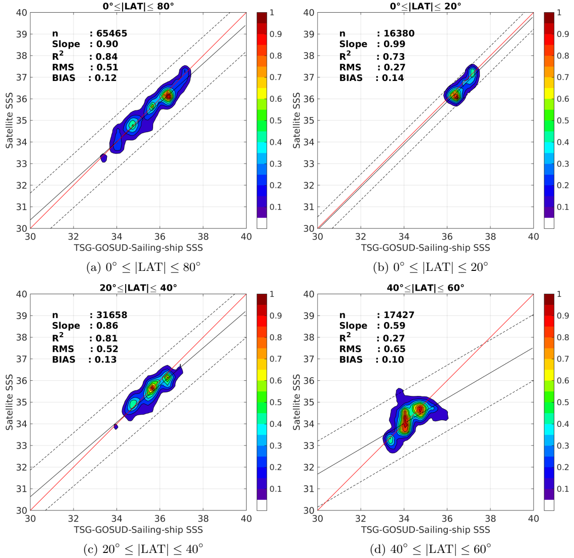
Figure 9: Contour maps of the concentration of SMOS-L3-CATDS-IFREMER-CECOS-V2-MONTHLY-0.25DEG SSS (y-axis) versus TSG-GOSUD-Sailing-ship SSS (x-axis) at match-up pairs for different latitude bands. For each plot, the red line shows x=y . The black thin and dashed lines indicate a linear fit through the data cloud and the \pm 95\% confidence levels, respectively. The number match-up pairs n , the slope and R^2 coefficient of the linear fit, the root mean square (RMS) and the mean bias between satellite and in situ data are indicated for each latitude band in each plots.
