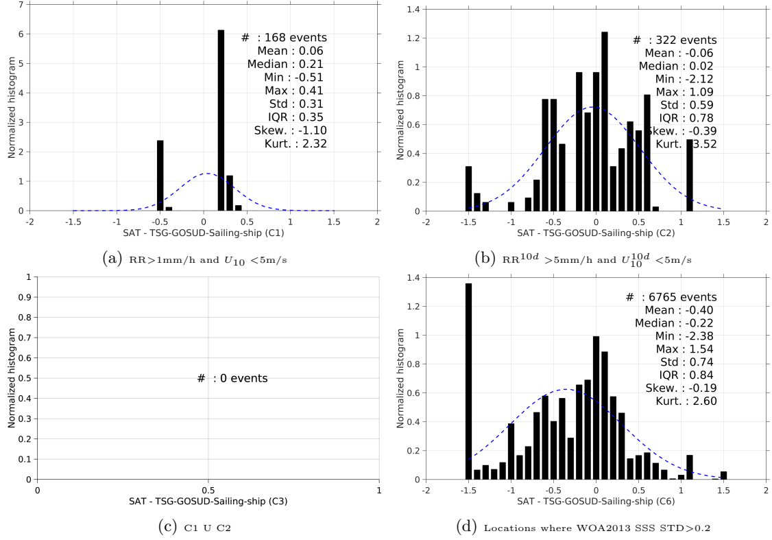
Figure 13: Normalized histogram of \Delta SSS (SMOS-L3-CATDS-IFREMER-CECOS-V2-MONTHLY-0.25DEG - TSG-GOSUD-Sailing-ship) for 6 different subdatasets corresponding to: RR > 1\text{mm/h} and U_{10} < 5\text{m/s} (a), RR^{10d} > 5\text{mm/h} and U_{10}^{10d} < 5\text{m/s} (b), C1 \cup C2 (c), Locations where WOA2013 SSS STD > 0.2 (d).
