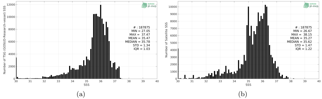
Figure 2: Histograms of SSS from TSG (GOSUD-Research-vessel) (a) and SMOS SSS L3 v2 - Monthly - 0.25 Deg (CATDS-CECOS-IFREMER) (b) considering all match-up pairs per bins of 0.1 over the South Atlantic Ocean Pi-MEP region and for the full satellite product period.
