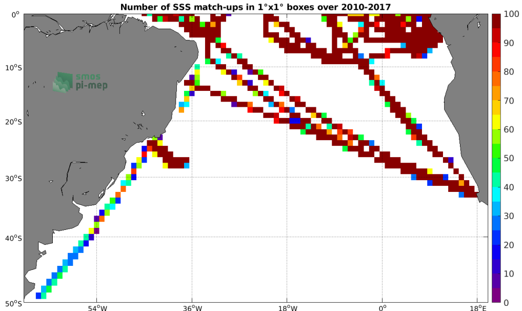
Figure 4: Number of SSS match-ups between TSG (GOSUD-Research-vessel) SSS and the SMOS SSS L3 v2 - Monthly - 0.25 Deg (CATDS-CECOS-IFREMER) SSS product for the South Atlantic Ocean Pi-MEP region over 1°x1° boxes and for the full satellite product period.
