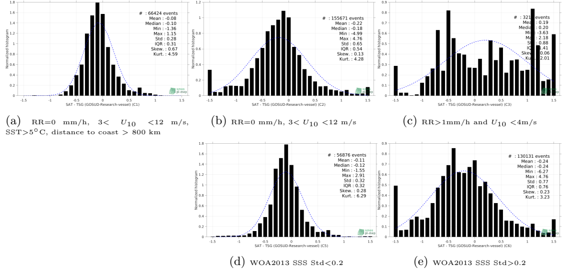
Figure 13: Normalized histogram of \Delta\text{SSS} (SMOS SSS L3 v2 - Monthly - 0.25 Deg (CATDS-CECOS-IFREMER) - TSG (GOSUD-Research-vessel)) for 5 different subdatasets corresponding to: RR=0 mm/h, 3 < U_{10} < 12 m/s, SST > 5^\circ\text{C} , distance to coast > 800 km (a), RR=0 mm/h, 3 < U_{10} < 12 m/s (b), RR > 1\text{mm/h} and U_{10} < 4\text{m/s} (c), WOA2013 SSS Std < 0.2 (d), WOA2013 SSS Std > 0.2 (e).
