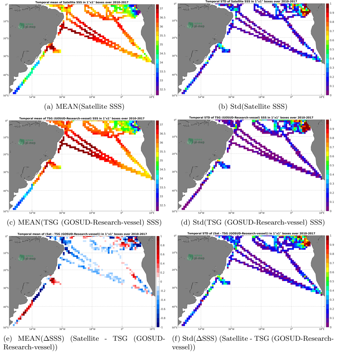
Figure 6: Temporal mean (left) and Std (right) of SSS from SMOS SSS L3 v2 - Monthly - 0.25 Deg (CATDS-CECOS-IFREMER) (top), TSG (GOSUD-Research-vessel) (middle), and of \Delta SSS (Satellite - TSG (GOSUD-Research-vessel)). Only match-up pairs are used to generate these maps.
