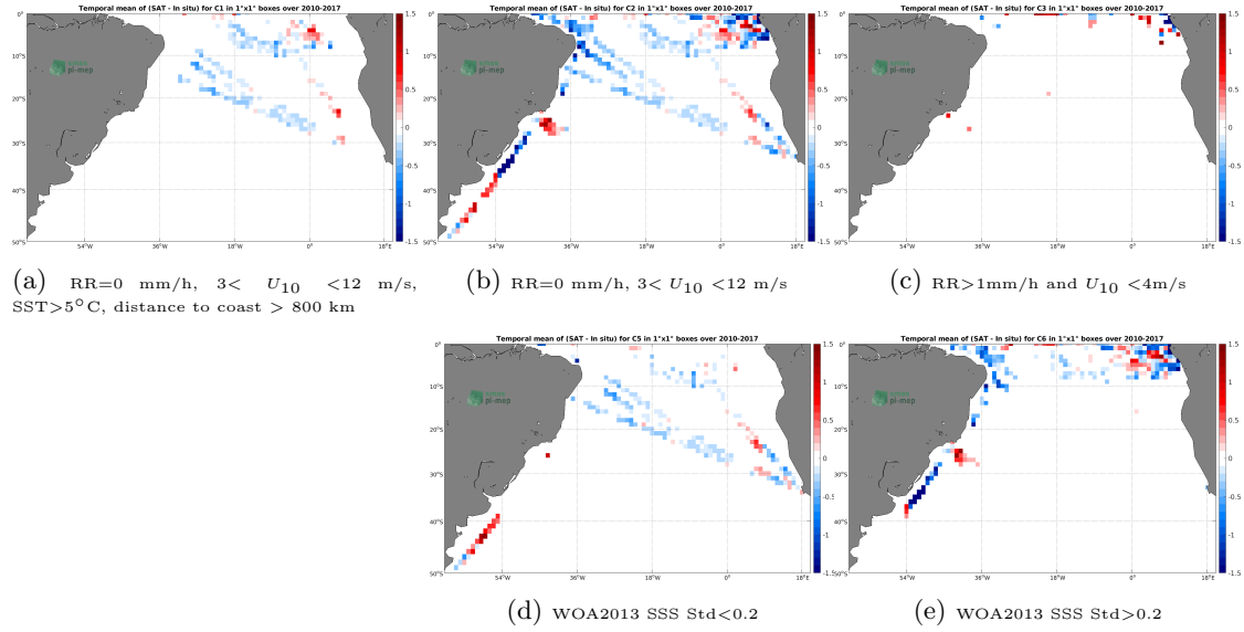
Figure 12: Temporal mean gridded over spatial boxes of size 1^\circ \times 1^\circ of \Delta SSS (SMOS SSS L3 v2 - Monthly - 0.25 Deg (CATDS-CECOS-IFREMER) - TSG (GOSUD-Research-vessel)) for 5 different subdatasets corresponding to:RR=0 mm/h, 3 < U_{10} < 12 m/s, SST >5^\circ\text{C} , distance to coast > 800 km (a), RR=0 mm/h, 3 < U_{10} < 12 m/s (b), RR >1 mm/h and U_{10} < 4 m/s (c), WOA2013 SSS Std <0.2 (d), WOA2013 SSS Std >0.2 (e).
