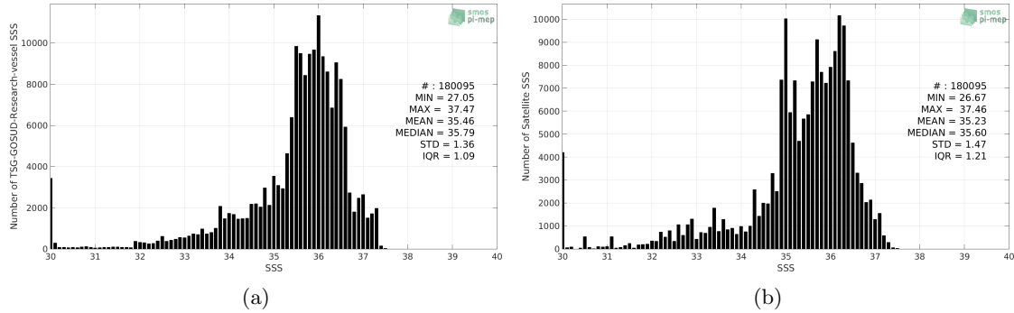
Figure 2: Histograms of SSS from TSG-GOSUD-Research-vessel (a) and SMOS-L3-CATDS-IFREMER-CECOS-V2-MONTHLY-0.25DEG (b) considering all match-up pairs per bins of 0.1 over the South Atlantic Ocean Pi-MEP region and for the full satellite product period.
