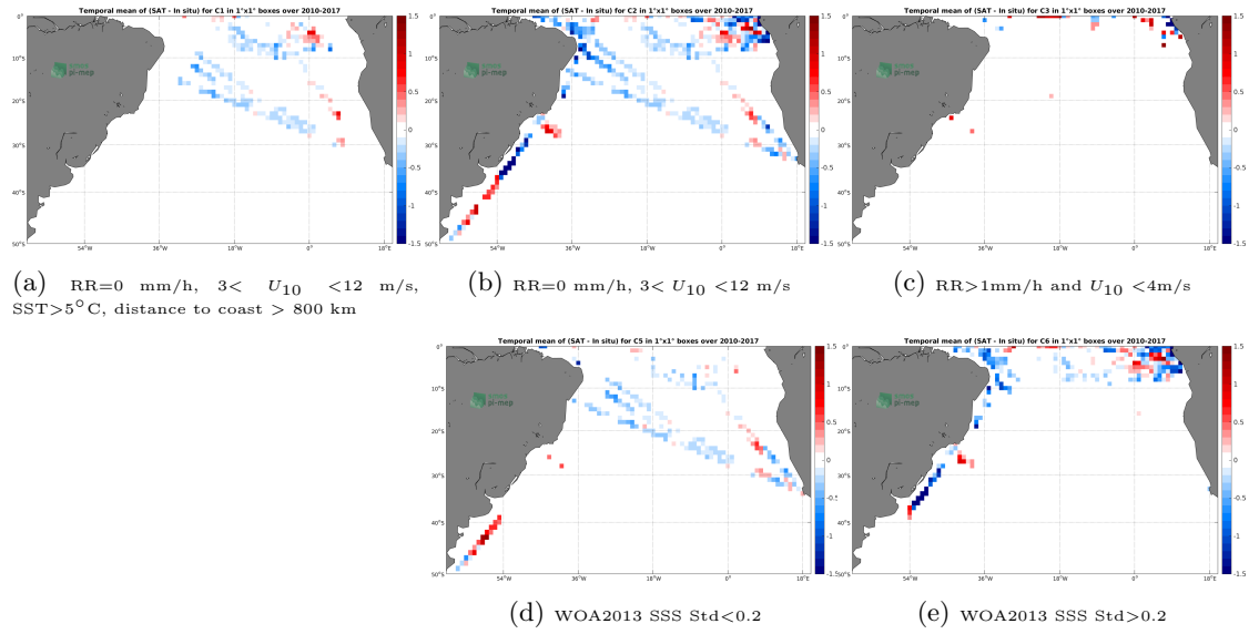
Figure 12: Temporal mean gridded over spatial boxes of size 1^\circ \times 1^\circ of \Delta SSS (SMOS-L3-CATDS-IFREMER-CECOS-V2-MONTHLY-0.25DEG - TSG-GOSUD-Research-vessel) for 5 different subdatasets corresponding to: RR=0 mm/h, 3 < U_{10} < 12 m/s, SST > 5^\circ C , distance to coast > 800 km (a), RR=0 mm/h, 3 < U_{10} < 12 m/s (b), RR > 1 mm/h and U_{10} < 4 m/s (c), WOA2013 SSS Std < 0.2 (d), WOA2013 SSS Std > 0.2 (e).
