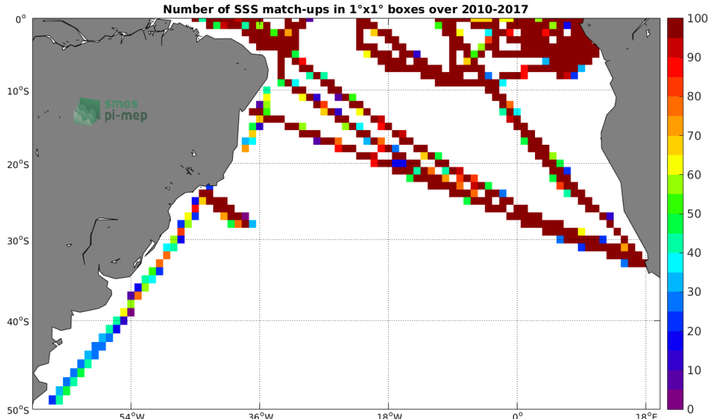
Figure 4: Number of SSS match-ups between TSG-GOSUD-Research-vessel SSS and the SMOS-L3-CATDS-IFREMER-CECOS-V2-MONTHLY-0.25DEG SSS product for the South Atlantic Ocean Pi-MEP region over 1°x1° boxes and for the full satellite product period.
