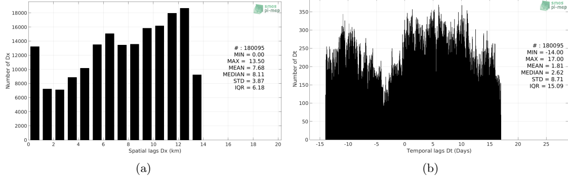
Figure 5: Histograms of the spatial (a) and temporal (b) lags between the time of the TSG-GOSUD-Research-vessel measurements and the date of the corresponding SMOS-L3-CATDS-IFREMER-CECOS-V2-MONTHLY-0.25DEG SSS product.
