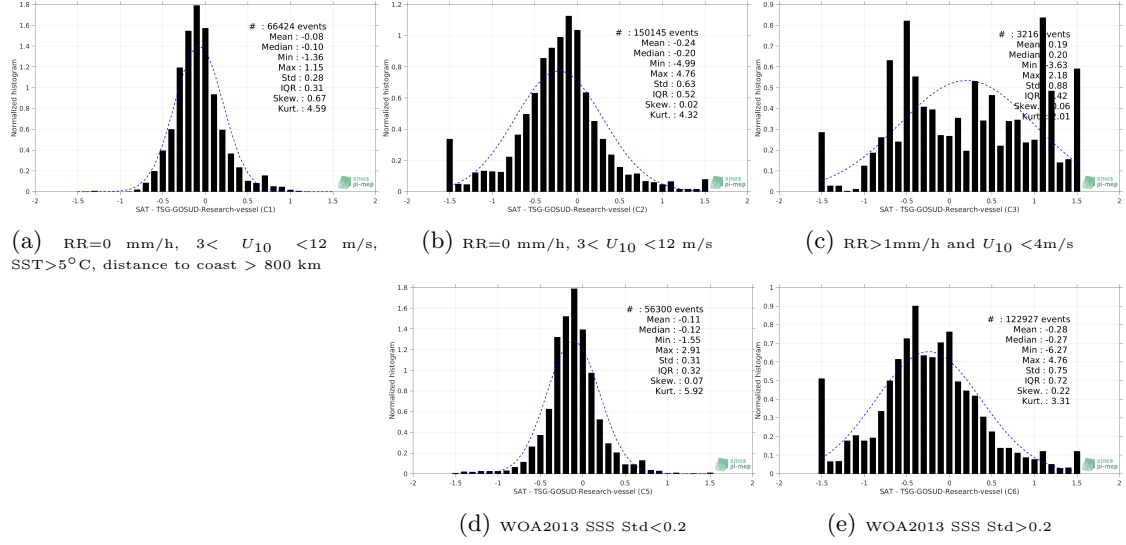
Figure 13: Normalized histogram of \Delta\text{SSS} (SMOS-L3-CATDS-IFREMER-CECOS-V2-MONTHLY-0.25DEG - TSG-GOSUD-Research-vessel) for 5 different subdatasets corresponding to: RR=0 mm/h, 3 < U_{10} < 12 m/s, SST >5^{\circ}\text{C} , distance to coast > 800 km (a), RR=0 mm/h, 3 < U_{10} < 12 m/s (b), RR>1\text{mm/h} and U_{10} < 4\text{m/s} (c), WOA2013 SSS Std <0.2 (d), WOA2013 SSS Std >0.2 (e).
