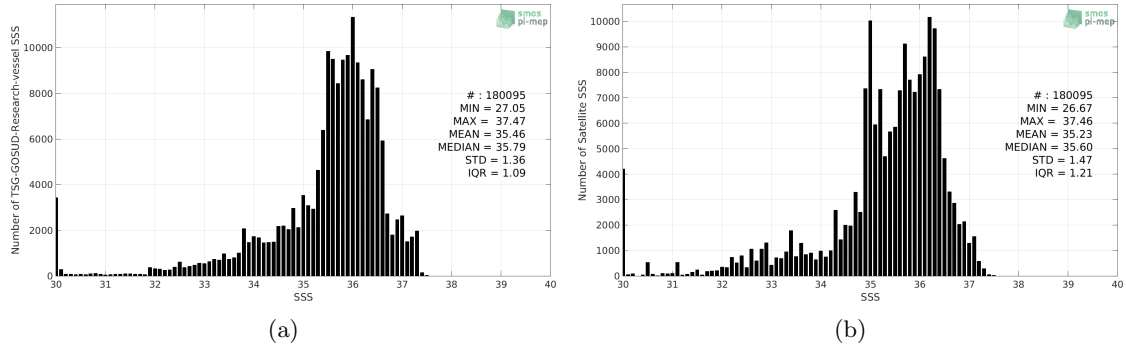
Figure 2: Histograms of SSS from TSG-GOSUD-Research-vessel (a) and SMOS-L3-CATDS-IFREMER-CECOS-V2-MONTHLY-0.25DEG (b) considering all match-up pairs per bins of 0.1 over the South Atlantic Ocean Pi-MEP region and for the full satellite product period.
