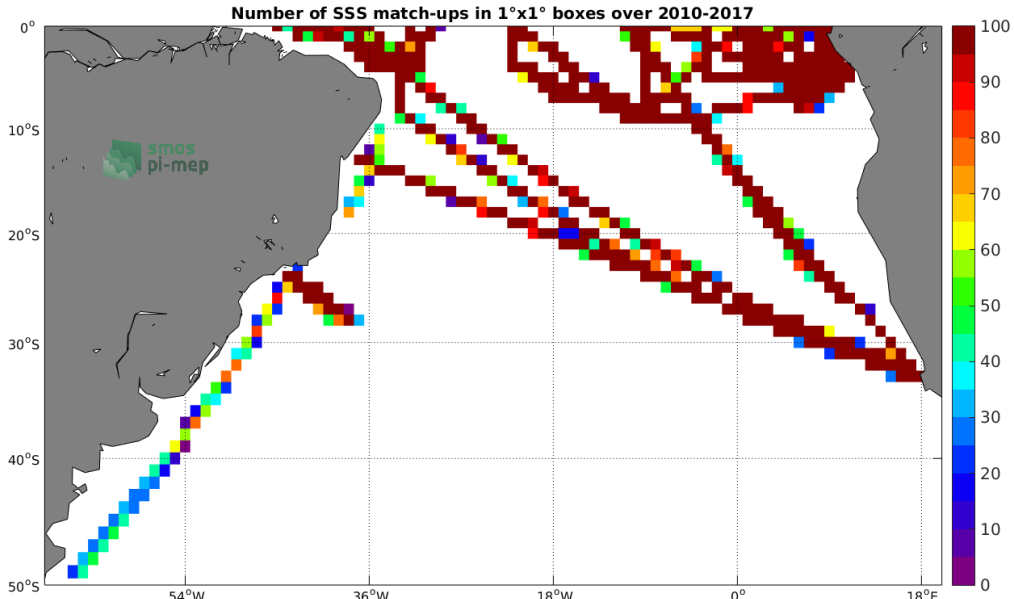
Figure 4: Number of SSS match-ups between TSG-GOSUD-Research-vessel SSS and the SMOS-L3-CATDS-IFREMER-CECOS-V2-MONTHLY-0.25DEG SSS product for the South Atlantic Ocean Pi-MEP region over 1^\circ \times 1^\circ boxes and for the full satellite product period.
