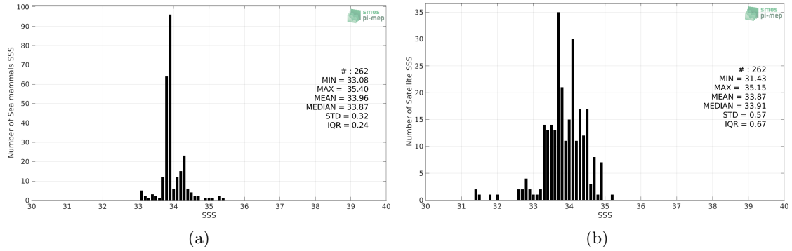
Figure 2: Histograms of SSS from Sea mammals (a) and SMOS SSS L3 v2 - Monthly - 0.25 Deg (CATDS-CECOS-IFREMER) (b) considering all match-up pairs per bins of 0.1 over the South Atlantic Ocean Pi-MEP region and for the full satellite product period.
