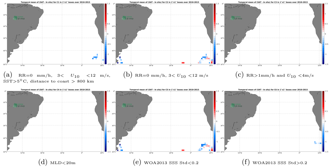
Figure 12: Temporal mean gridded over spatial boxes of size 1^{\circ}\times 1^{\circ} of \Delta\text{SSS} (SMOS SSS L3 v2 - Monthly - 0.25 Deg (CATDS-CECOS-IFREMER) - Sea mammals) for 6 different subdatasets corresponding to: \text{RR}=0 mm/h, 3 < U_{10} < 12 m/s, \text{SST} > 5^{\circ}\text{C} , distance to coast > 800 km (a), \text{RR}=0 mm/h, 3 < U_{10} < 12 m/s (b), \text{RR} > 1\text{mm/h} and U_{10} < 4\text{m/s} (c), \text{MLD} < 20\text{m} (d), \text{WOA2013 SSS Std} < 0.2 (e), \text{WOA2013 SSS Std} > 0.2 (f).
