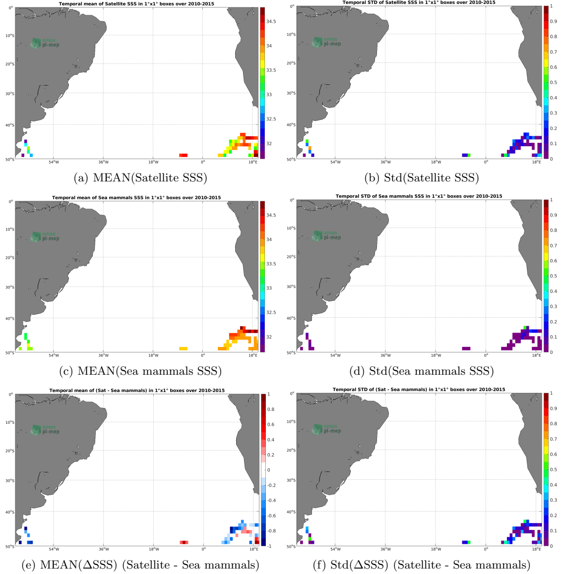
Figure 6: Temporal mean (left) and Std (right) of SSS from SMOS SSS L3 v2 - Monthly - 0.25 Deg (CATDS-CECOS-IFREMER) (top), Sea mammals (middle), and of \Delta SSS (Satellite - Sea mammals). Only match-up pairs are used to generate these maps.
