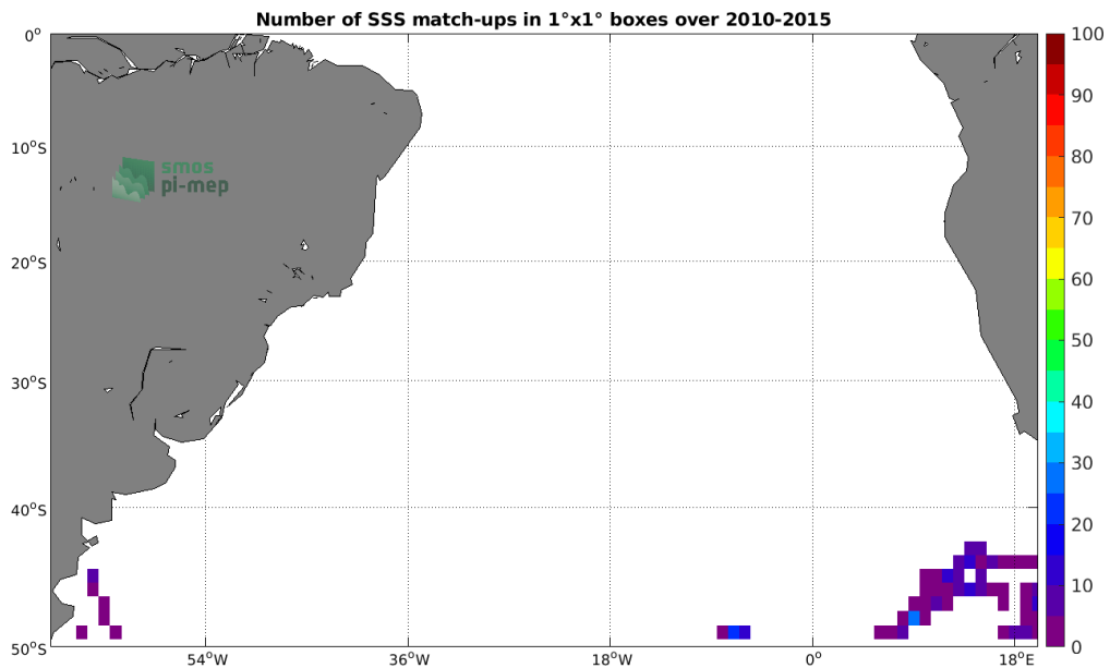
Figure 4: Number of SSS match-ups between Sea mammals SSS and the SMOS SSS L3 v2 - Monthly - 0.25 Deg (CATDS-CECOS-IFREMER) SSS product for the South Atlantic Ocean Pi-MEP region over 1°x1° boxes and for the full satellite product period.
