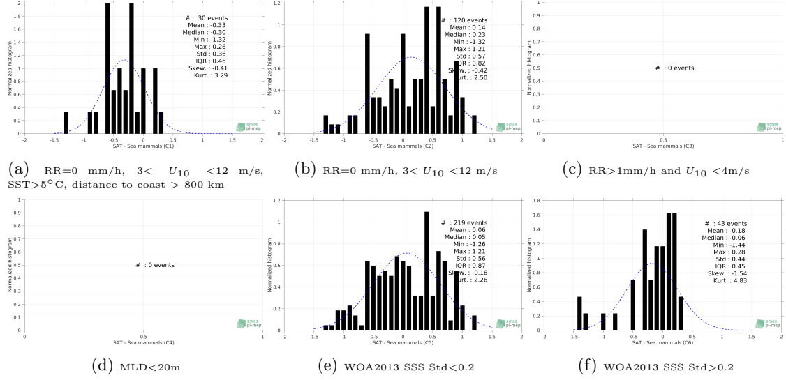
Figure 13: Normalized histogram of \Delta\text{SSS} (SMOS SSS L3 v2 - Monthly - 0.25 Deg (CATDS-CECOS-IFREMER) - Sea mammals) for 6 different subdatasets corresponding to: RR=0 mm/h, 3 < U_{10} < 12 m/s, SST > 5^{\circ}\text{C} , distance to coast > 800 km (a), RR=0 mm/h, 3 < U_{10} < 12 m/s (b), RR > 1\text{mm/h} and U_{10} < 4\text{m/s} (c), MLD < 20\text{m} (d), WOA2013 SSS Std < 0.2 (e), WOA2013 SSS Std > 0.2 (f).
