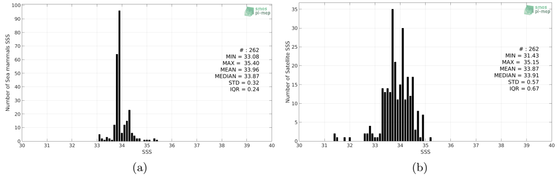
Figure 2: Histograms of SSS from Sea mammals (a) and SMOS-L3-CATDS-IFREMER-CECOS-V2-MONTHLY-0.25DEG (b) considering all match-up pairs per bins of 0.1 over the South Atlantic Ocean Pi-MEP region and for the full satellite product period.
