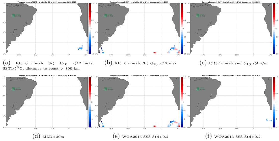
Figure 12: Temporal mean gridded over spatial boxes of size 1^\circ \times 1^\circ of \Delta SSS (SMOS-L3-CATDS-IFREMER-CECOS-V2-MONTHLY-0.25DEG - Sea mammals) for 6 different subdatasets corresponding to: RR=0 mm/h, 3 < U_{10} < 12 m/s, SST > 5^\circ\text{C} , distance to coast > 800 km (a), RR=0 mm/h, 3 < U_{10} < 12 m/s (b), RR > 1 mm/h and U_{10} < 4 m/s (c), MLD < 20 m (d), WOA2013 SSS Std < 0.2 (e), WOA2013 SSS Std > 0.2 (f).
