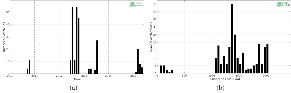
Figure 1: Number of match-ups between Sea mammals and SMOS-L3-CATDS-IFREMER-CECOS-V2-MONTHLY-0.25DEG SSS as a function of time (a) and as function of the distance to coast (b) over the South Atlantic Ocean Pi-MEP region and for the full satellite product period.
