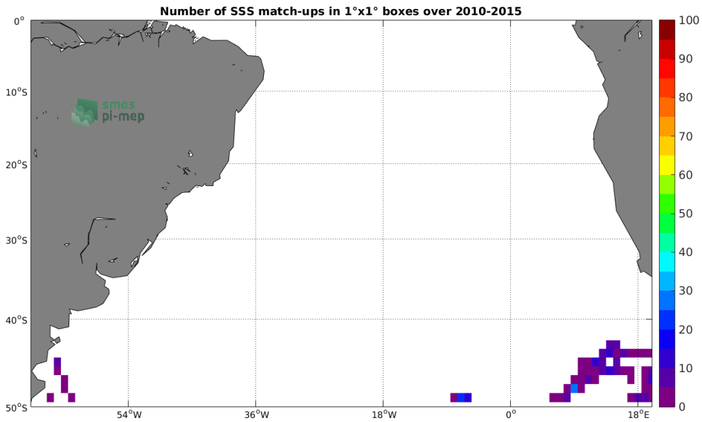
Figure 4: Number of SSS match-ups between Sea mammals SSS and the SMOS-L3-CATDS-IFREMER-CECOS-V2-MONTHLY-0.25DEG SSS product for the South Atlantic Ocean Pi-MEP region over 1°x1° boxes and for the full satellite product period.
