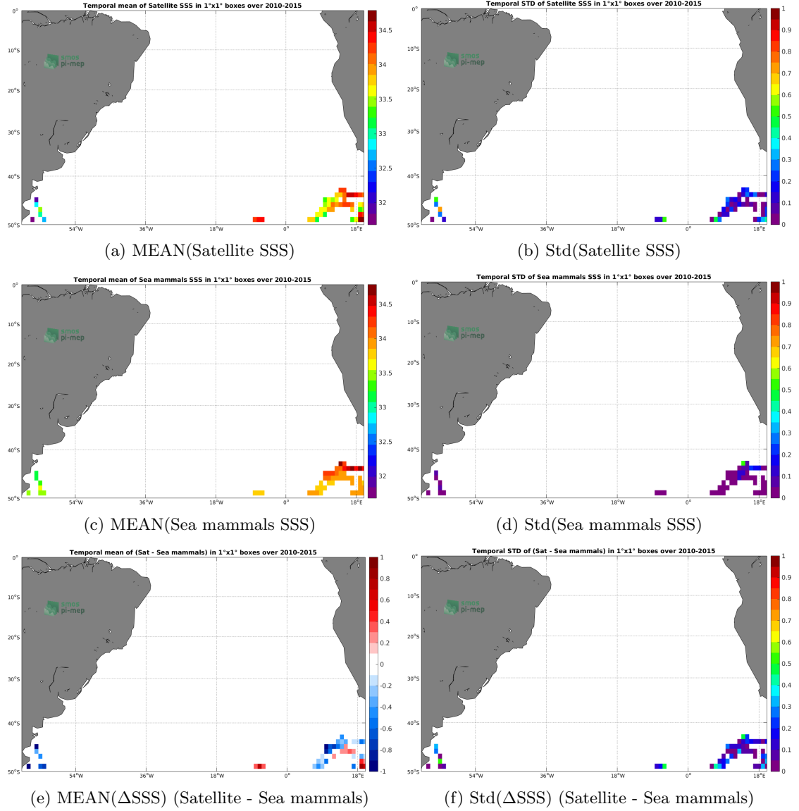
Figure 6: Temporal mean (left) and Std (right) of SSS from SMOS-L3-CATDS-IFREMER-CECOS-V2-MONTHLY-0.25DEG (top), Sea mammals (middle), and of \Delta SSS (Satellite - Sea mammals). Only match-up pairs are used to generate these maps.
